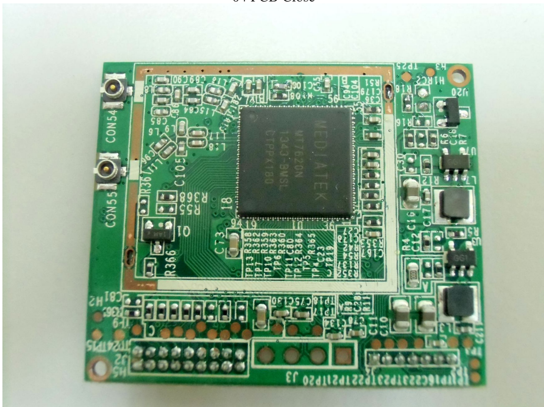
04 PCB Close
