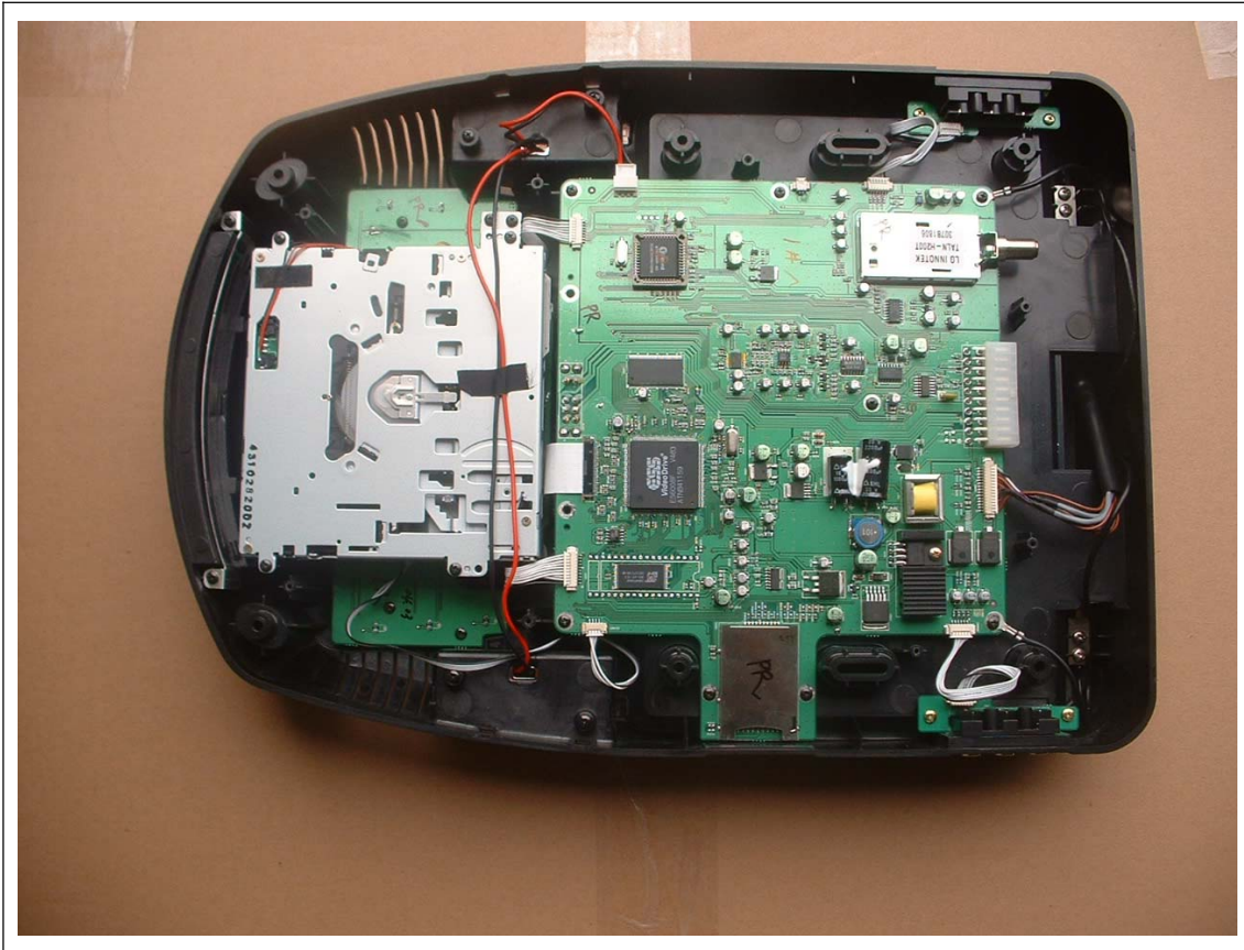
View 1 (Internal)
