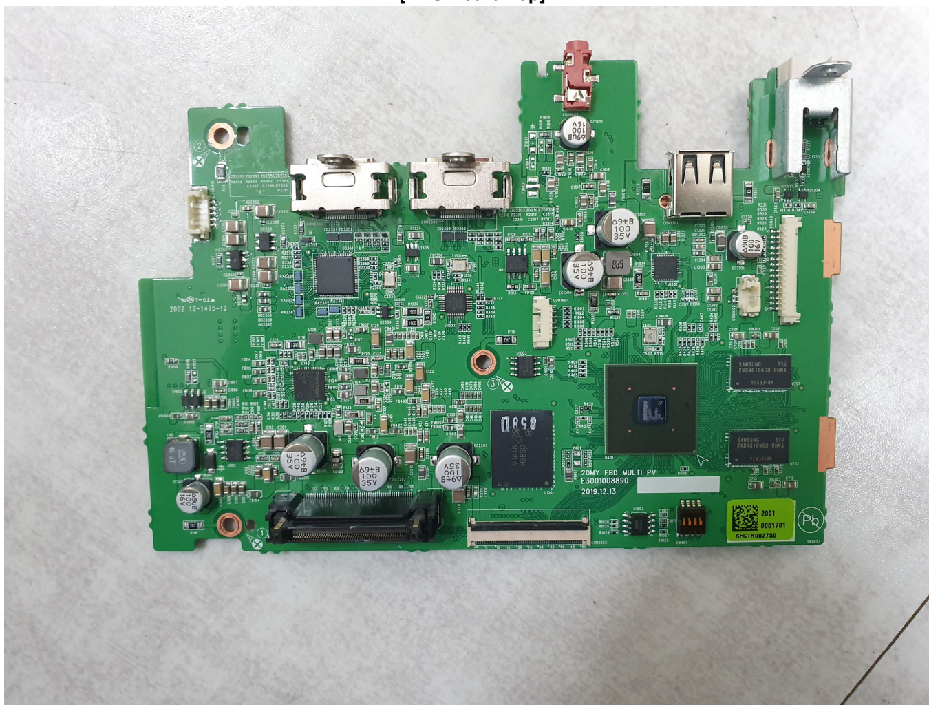
[CPU Board Top]
