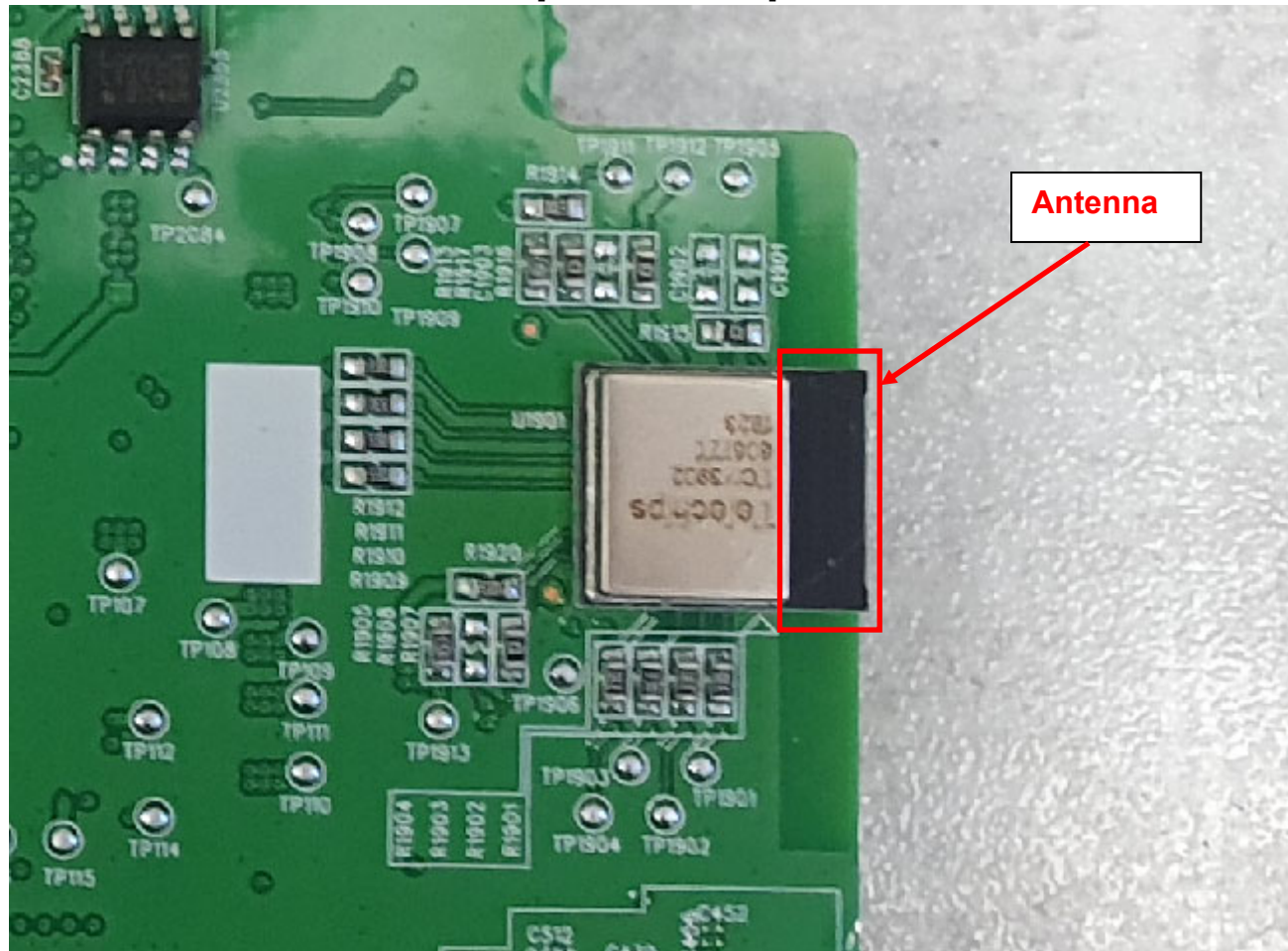
[Bluetooth Module]
