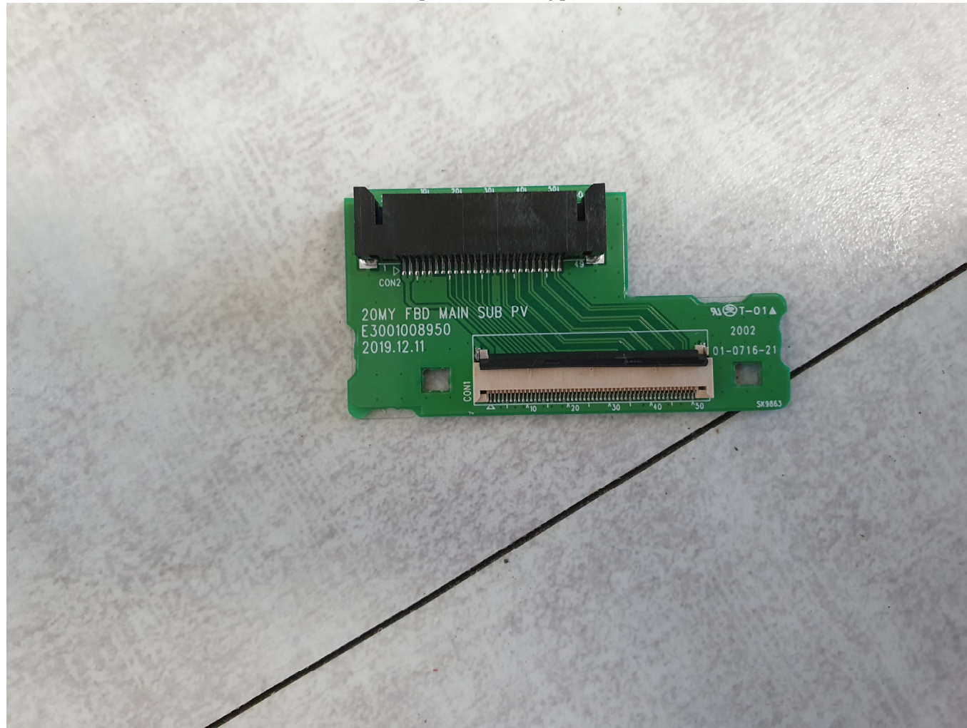
[Sub Board Top]
