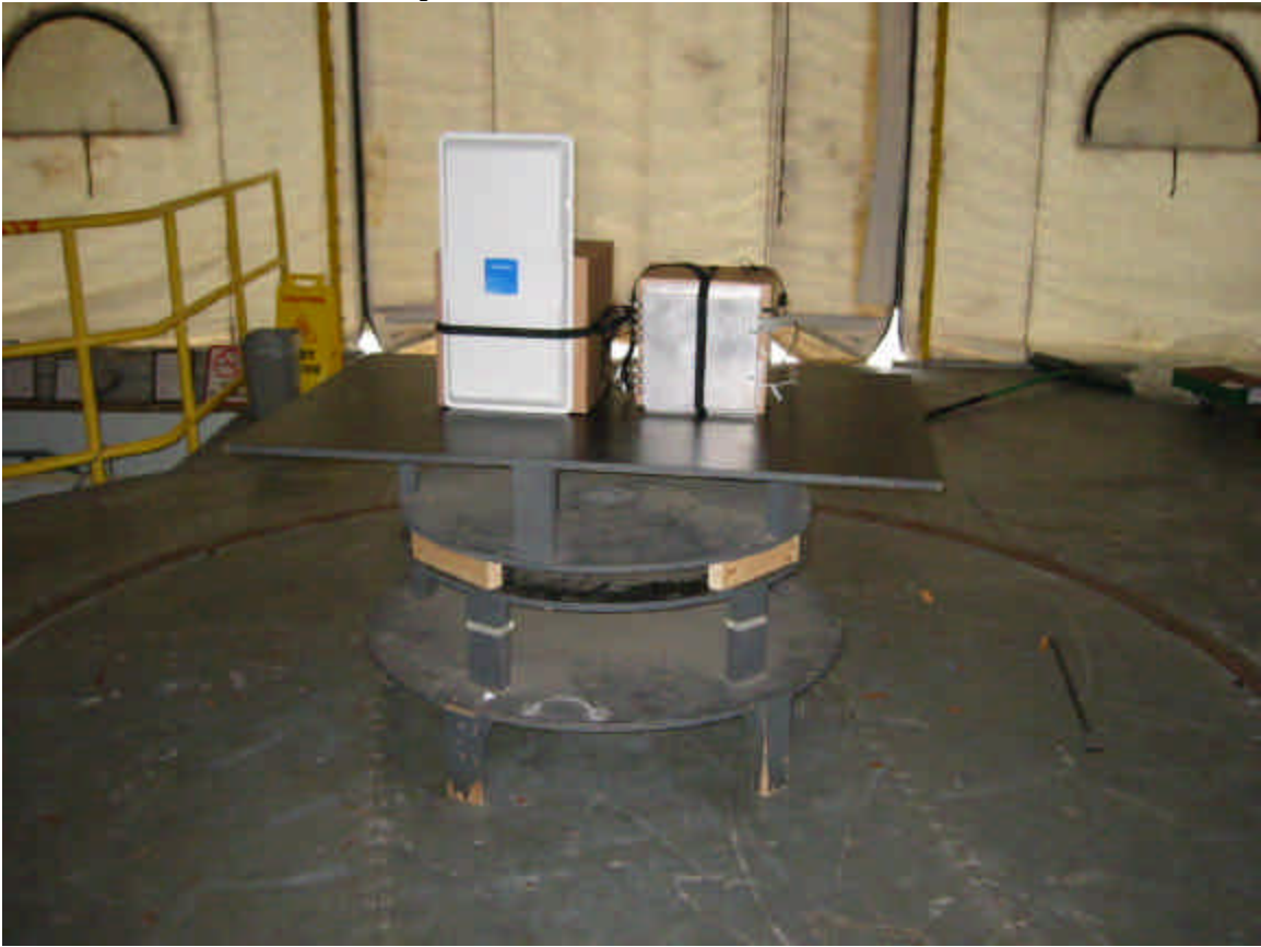
Radiated Emissions Test Setup Photos
