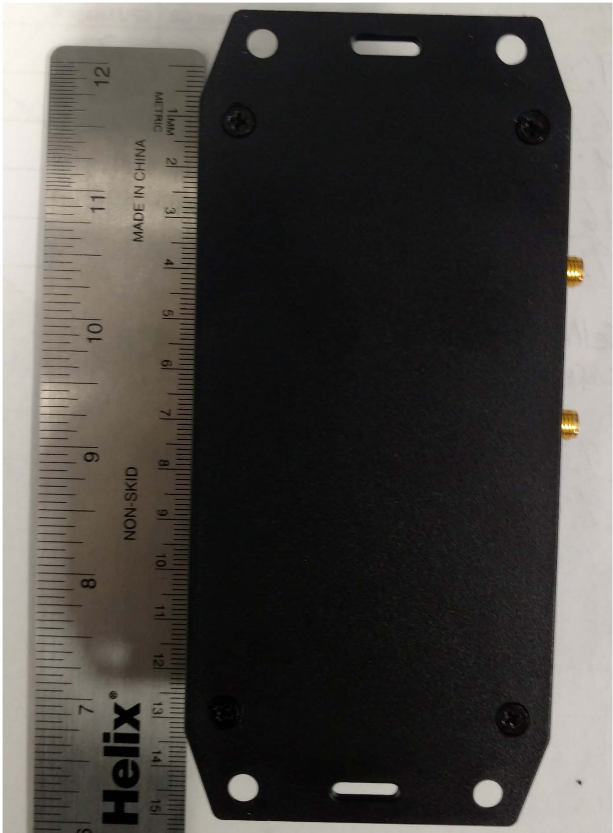
Figure 6 Bottom RFID enclosure and module
