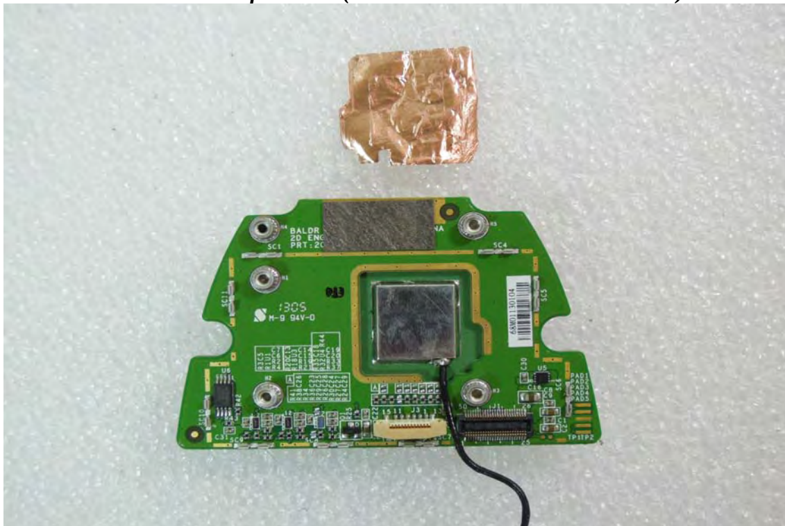
Internal View of EUT-21 (Model no.: JUNO/T41/5-BWCRFG)
