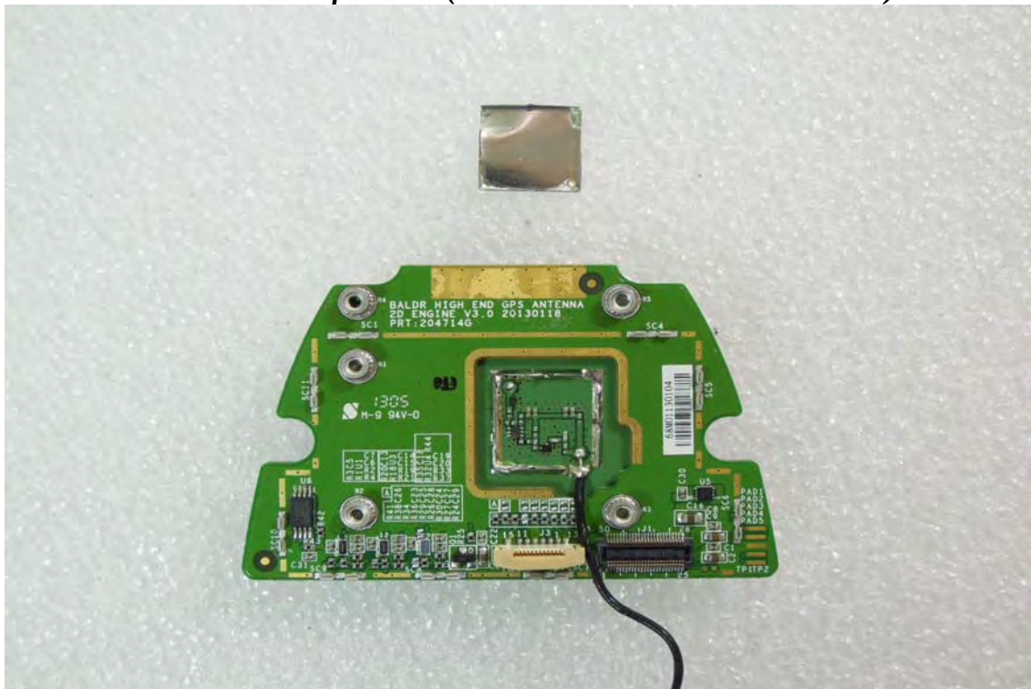
Internal View of EUT-23(Model no.: JUNO/T41/5-BWCRFG)
