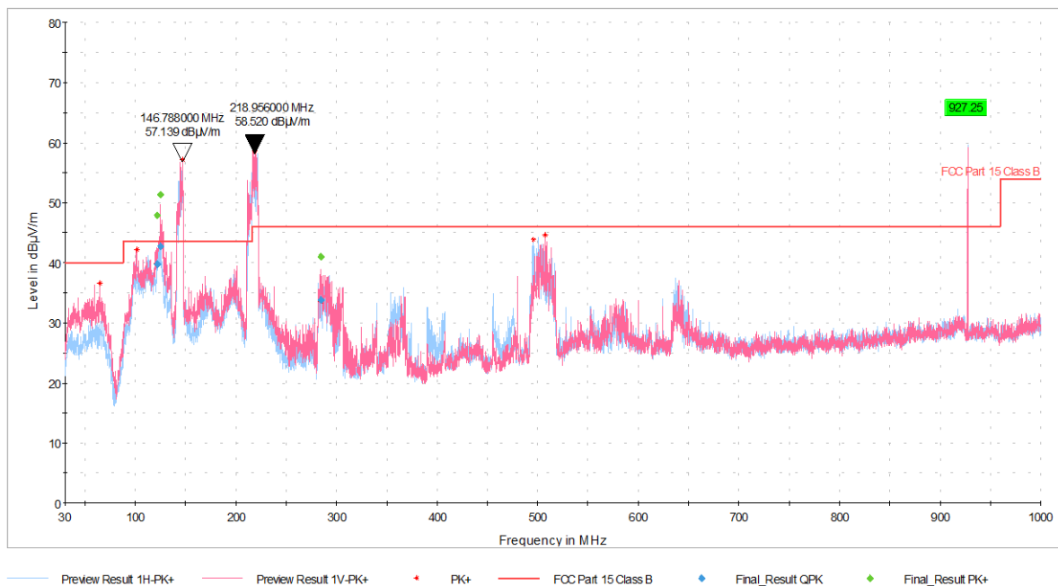
Figure 5. 30MHz-1GHz, 927.25 MHz
