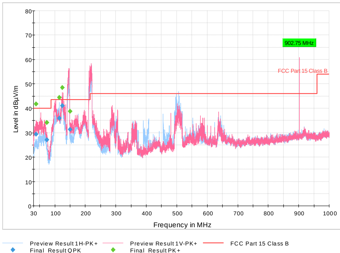
Figure 3. 30MHz-1GHz, 902.75 MHz
