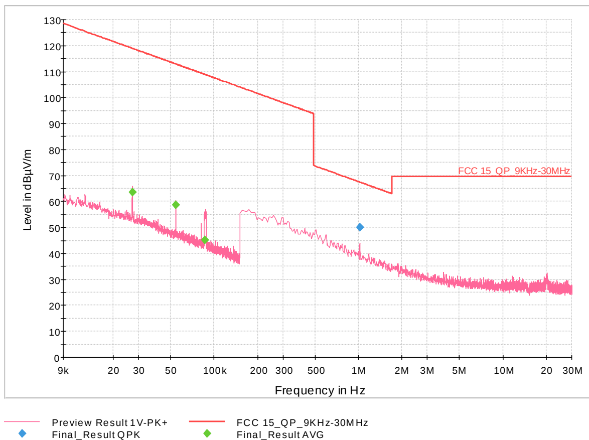
Figure 1. 9 kHz-30 MHz, 902.75 MHz, 0 Degrees
