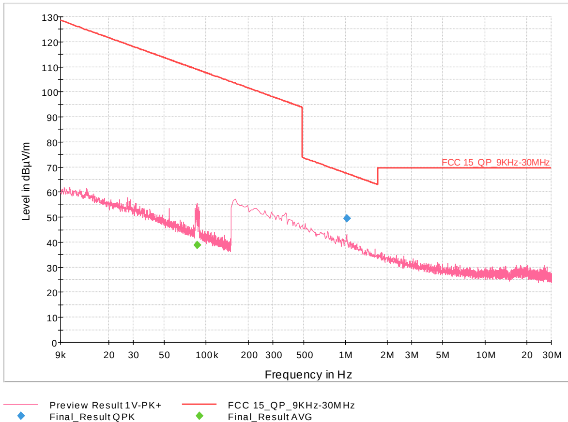
Figure 2. 9 kHz-30 MHz, 902.75 MHz, 90 Degrees
