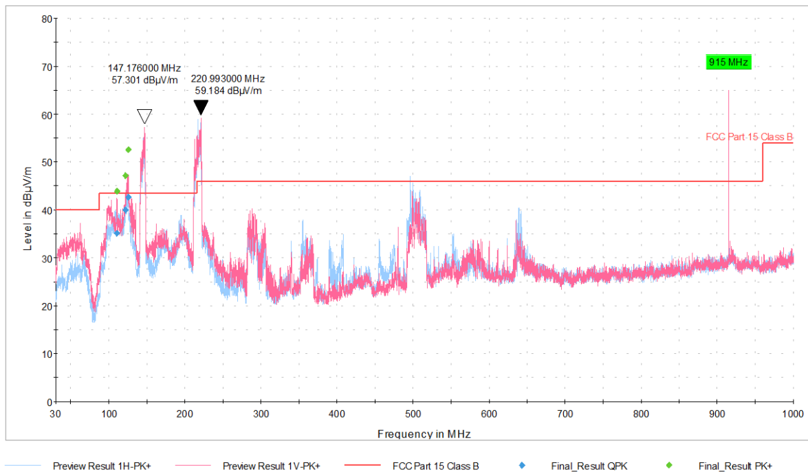
Figure 4. 30MHz-1GHz, 915 MHz
