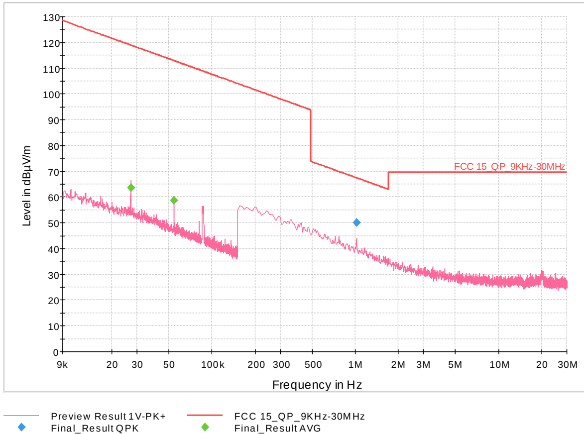
Figure 23. 9 kHz-30 MHz, 915 MHz, 0 Degrees
