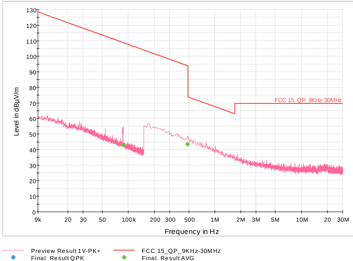
Figure 24. 9 kHz-30 MHz, 915 MHz, 90 Degrees
