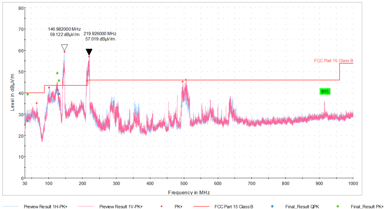
Figure 28. 30MHz-1GHz, 915 MHz
