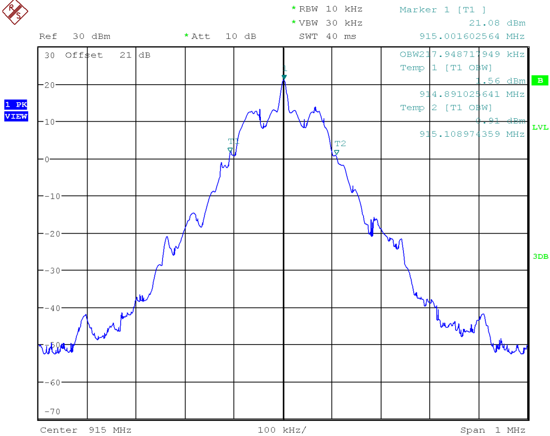
Figure 12. 915 MHz, 99% Bandwidth
