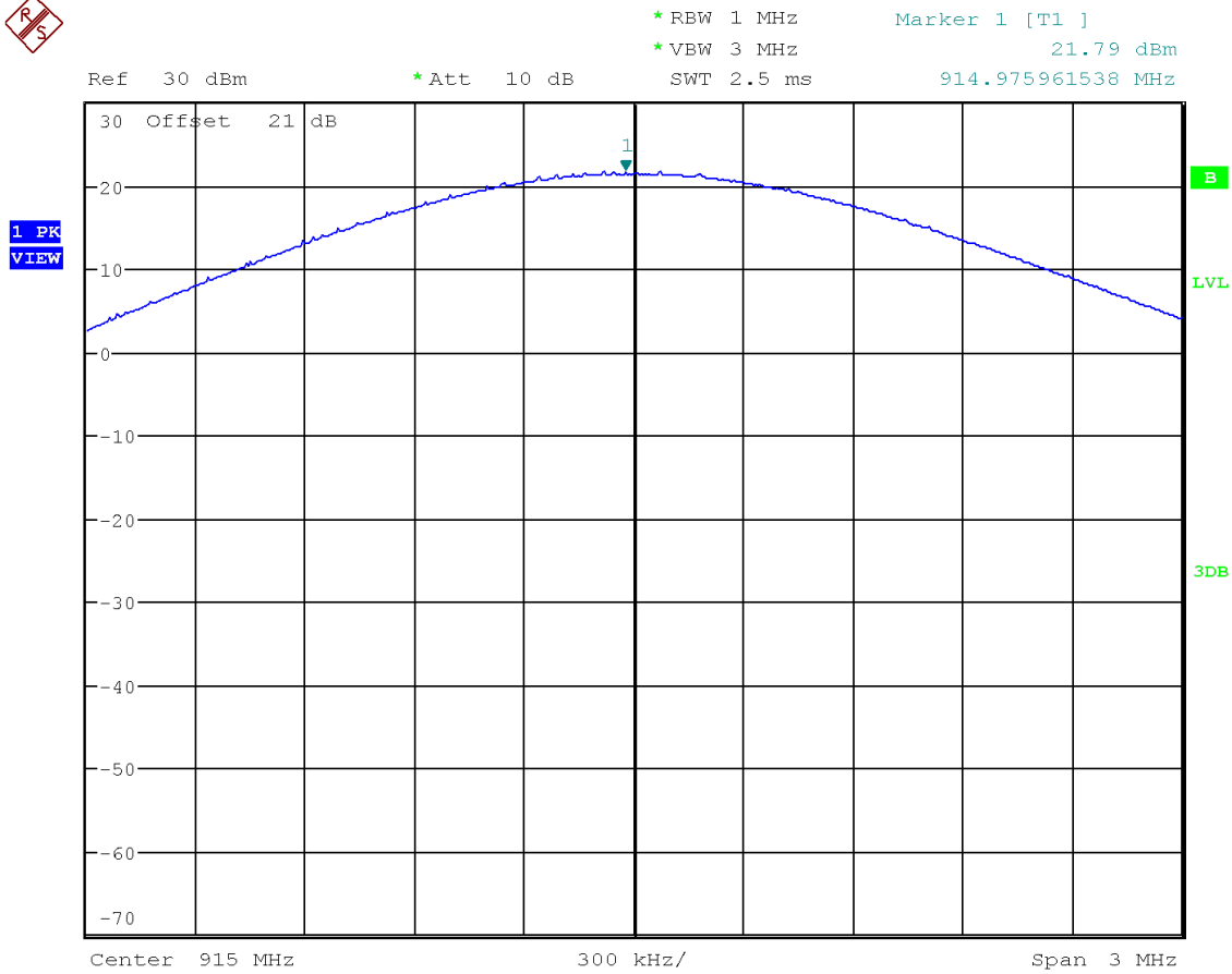
Figure 7. Maximum Conducted Power, 915 MHz
