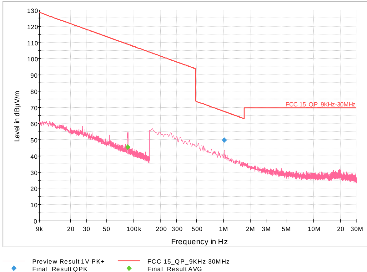
Figure 22. 9 kHz-30 MHz, 902.75 MHz, 90 Degrees
