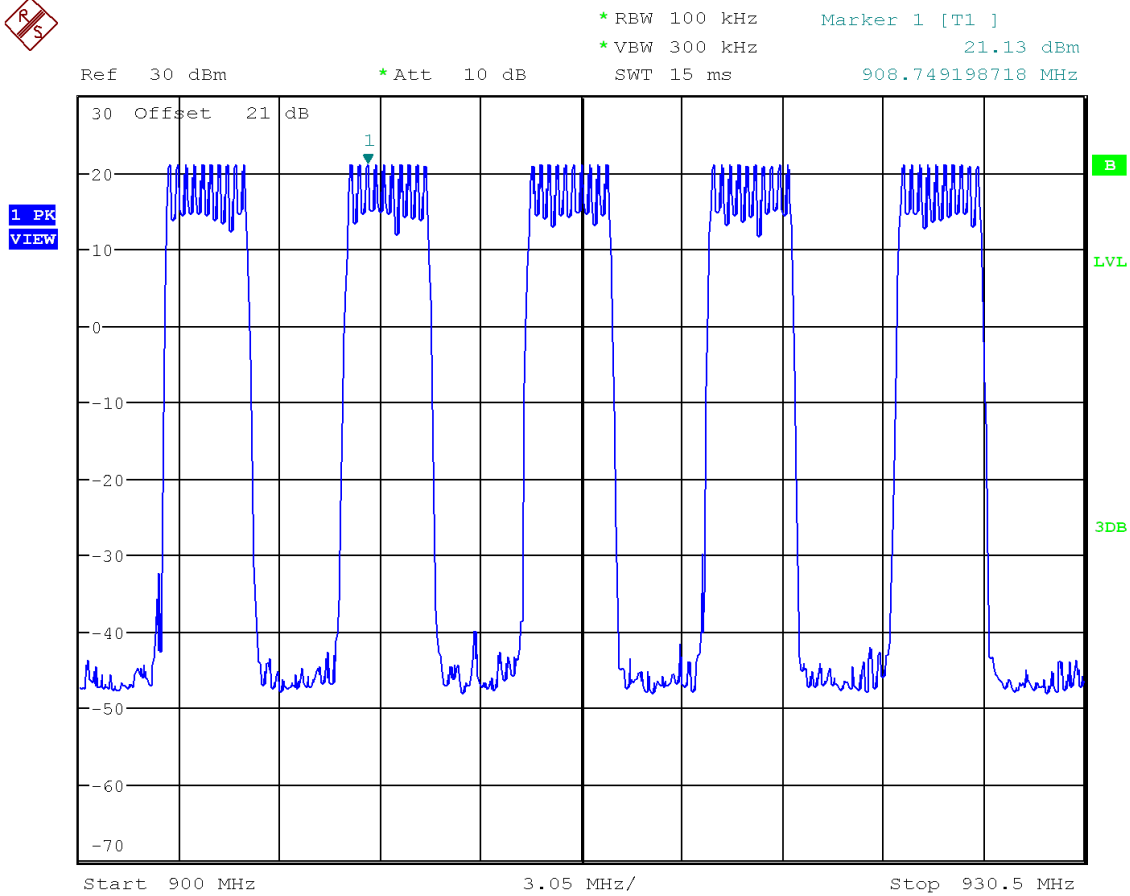
Figure 4. Number of Operating Channels
