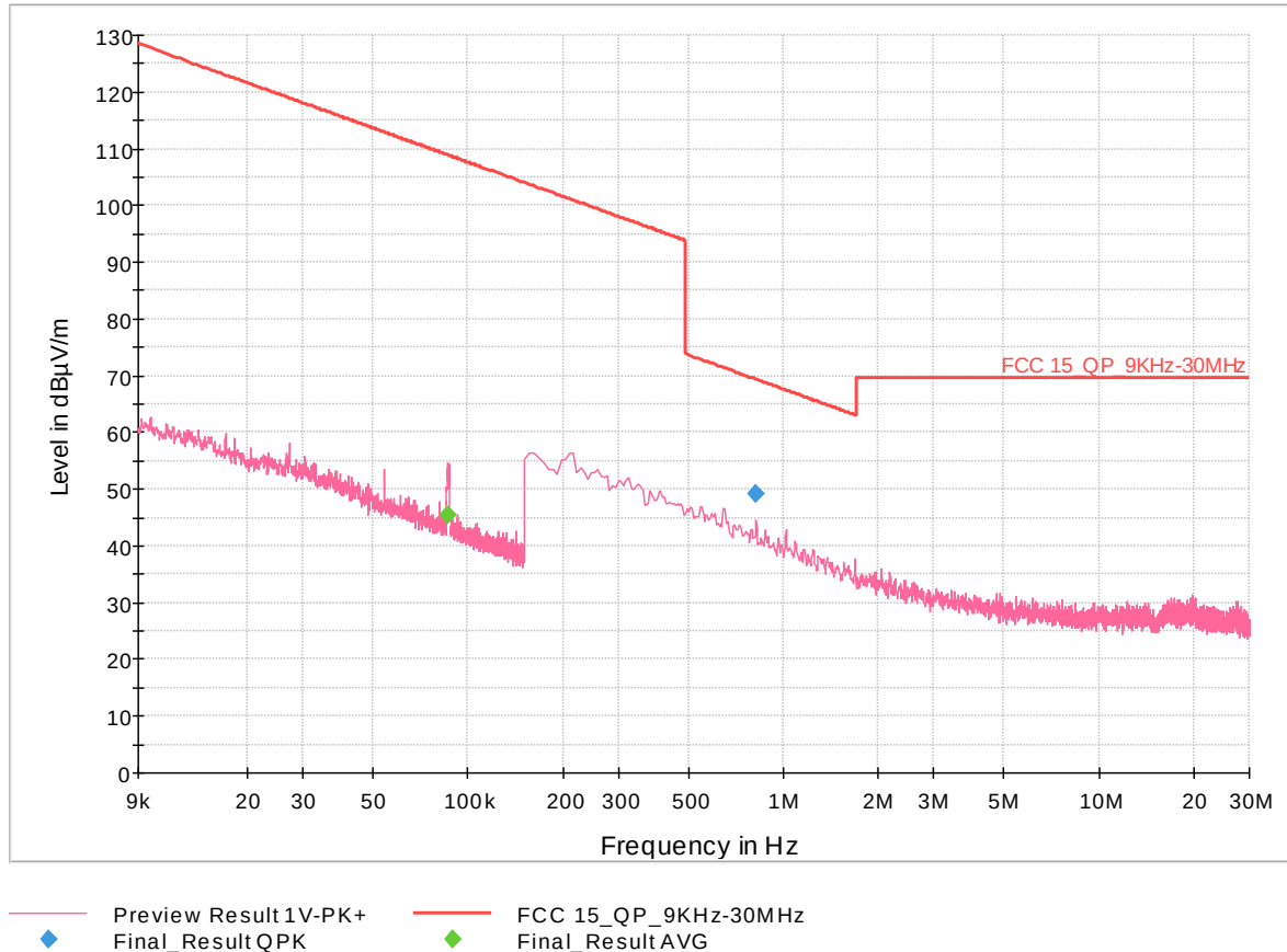
Figure 26. 9 kHz-30 MHz, 927.25 MHz, 90 Degrees
