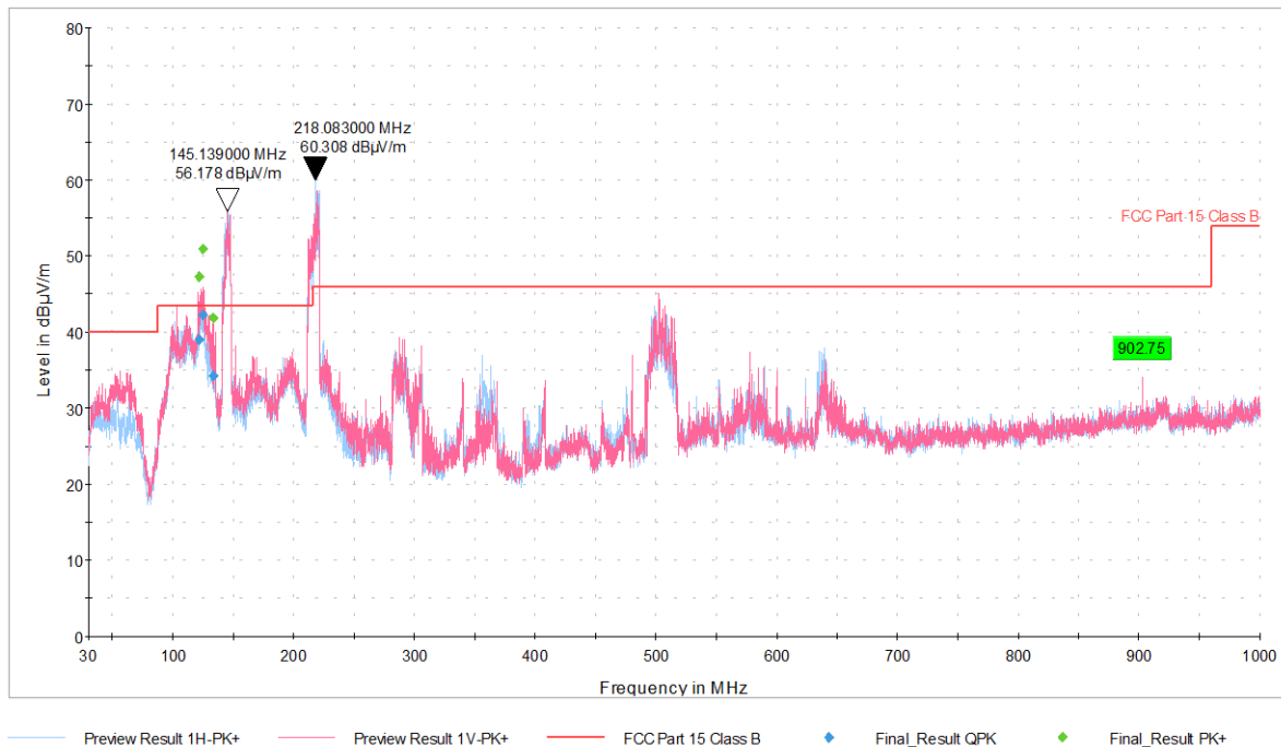
Figure 27. 30MHz-1GHz, 902.75 MHz
