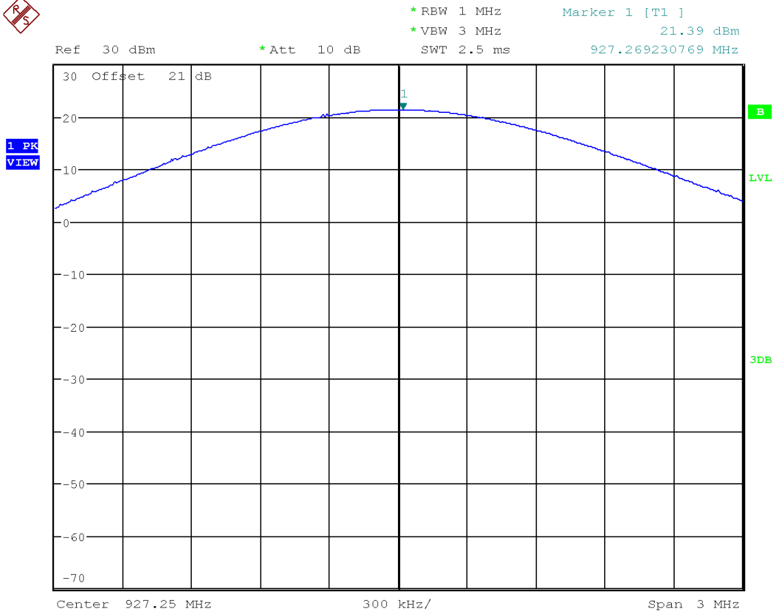
Figure 8. Maximum Conducted Power, 927.25 MHz
