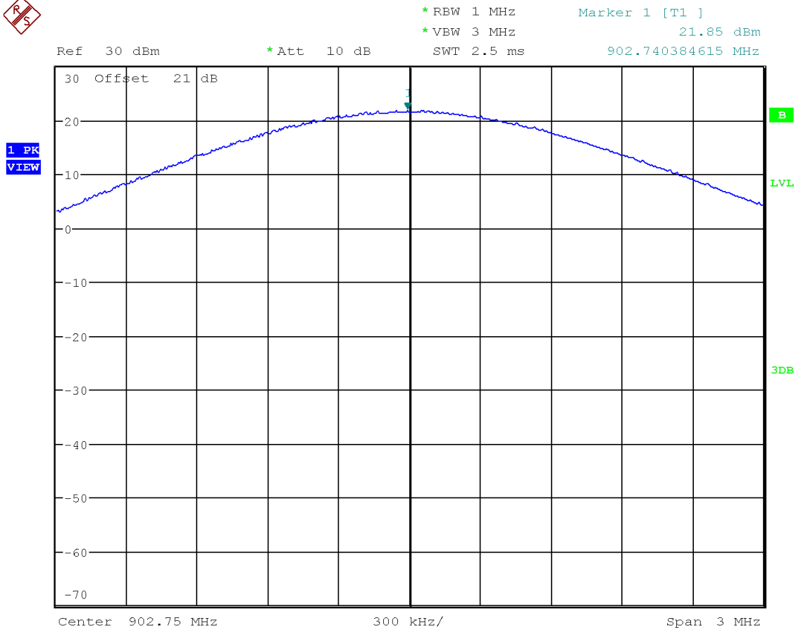
Figure 6. Maximum Conducted Power, 902.75 MHz
