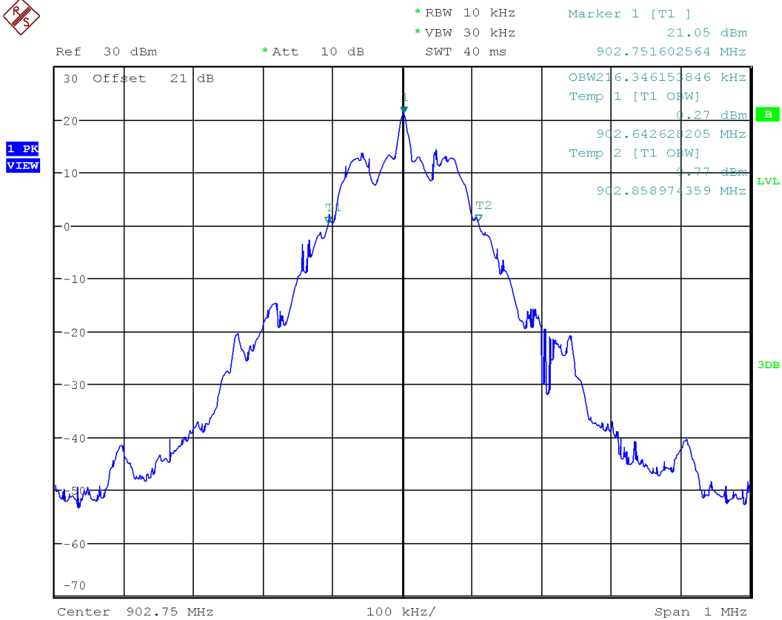
Figure 10. 902.75 MHz, 99% Bandwidth
