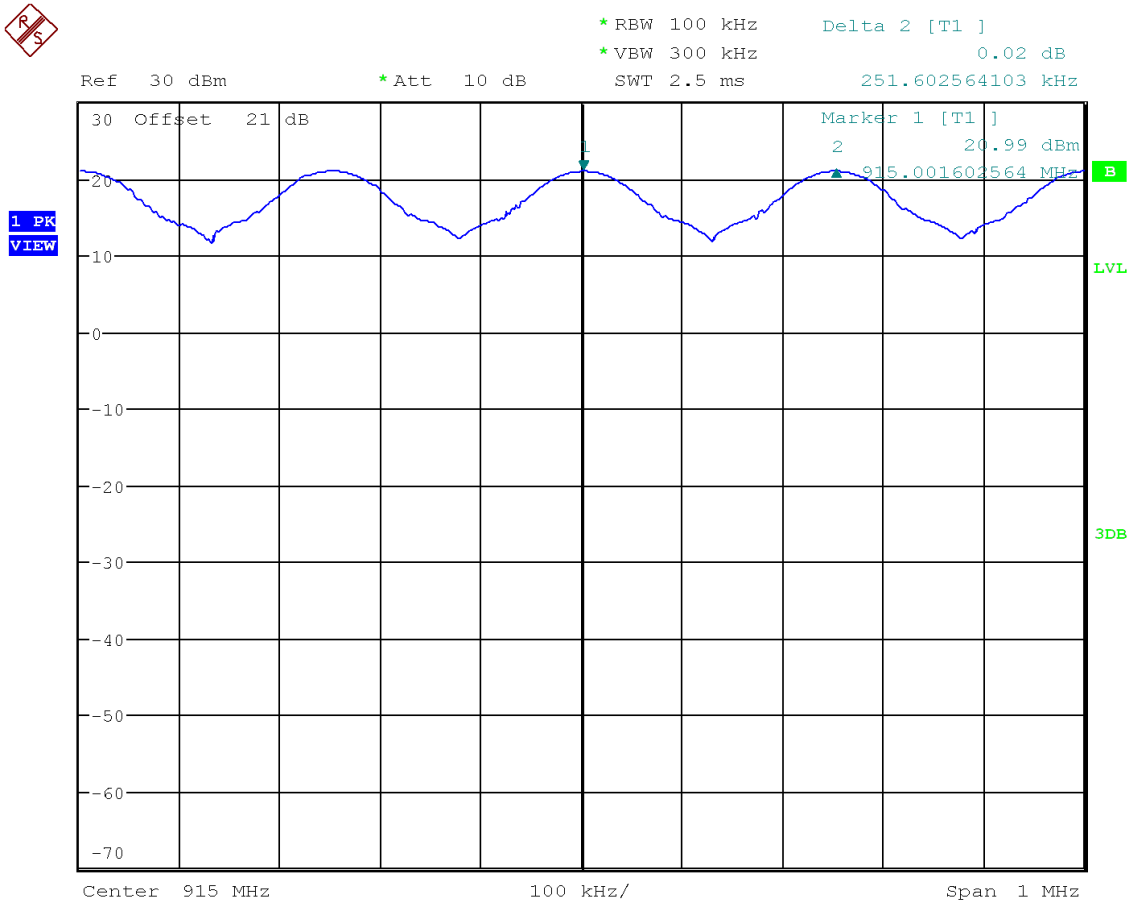
Figure 5. Channel Separation
