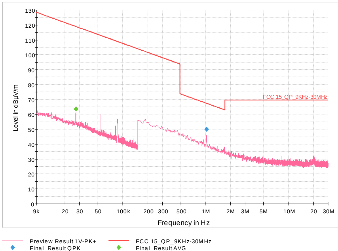
Figure 25. 9 kHz-30 MHz, 927.25 MHz, 0 Degrees
