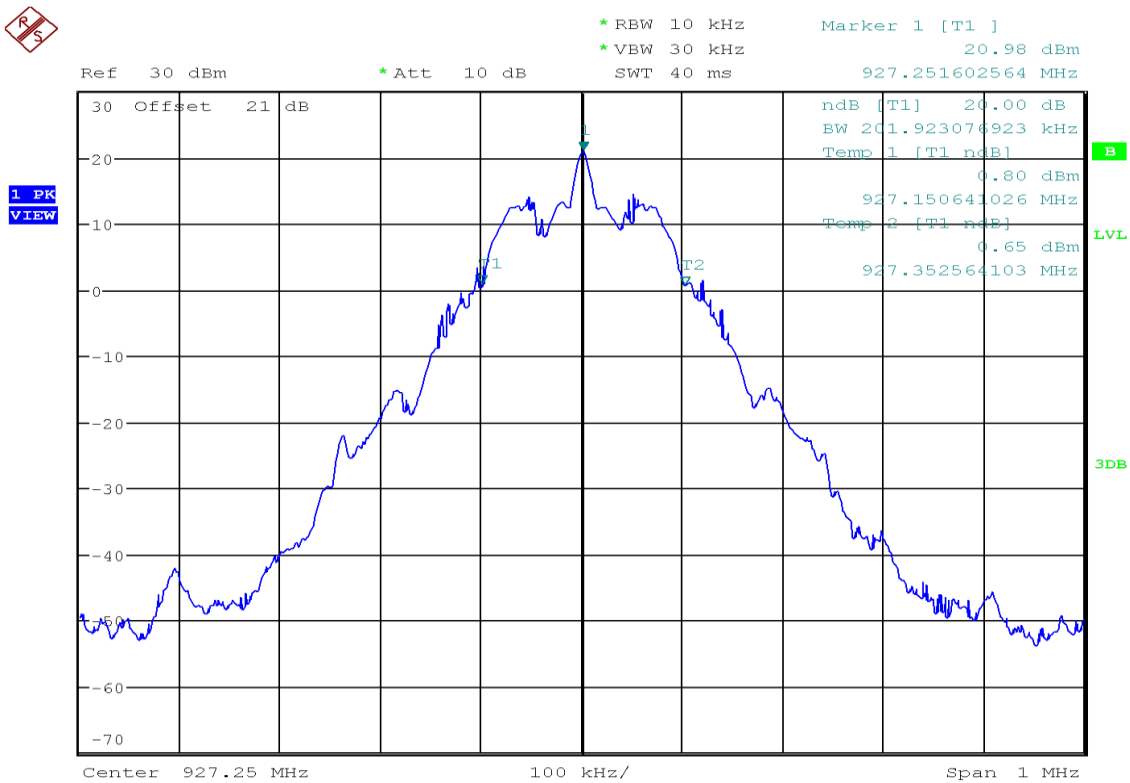
Figure 13. 927.25 MHz, 20dB Bandwidth
