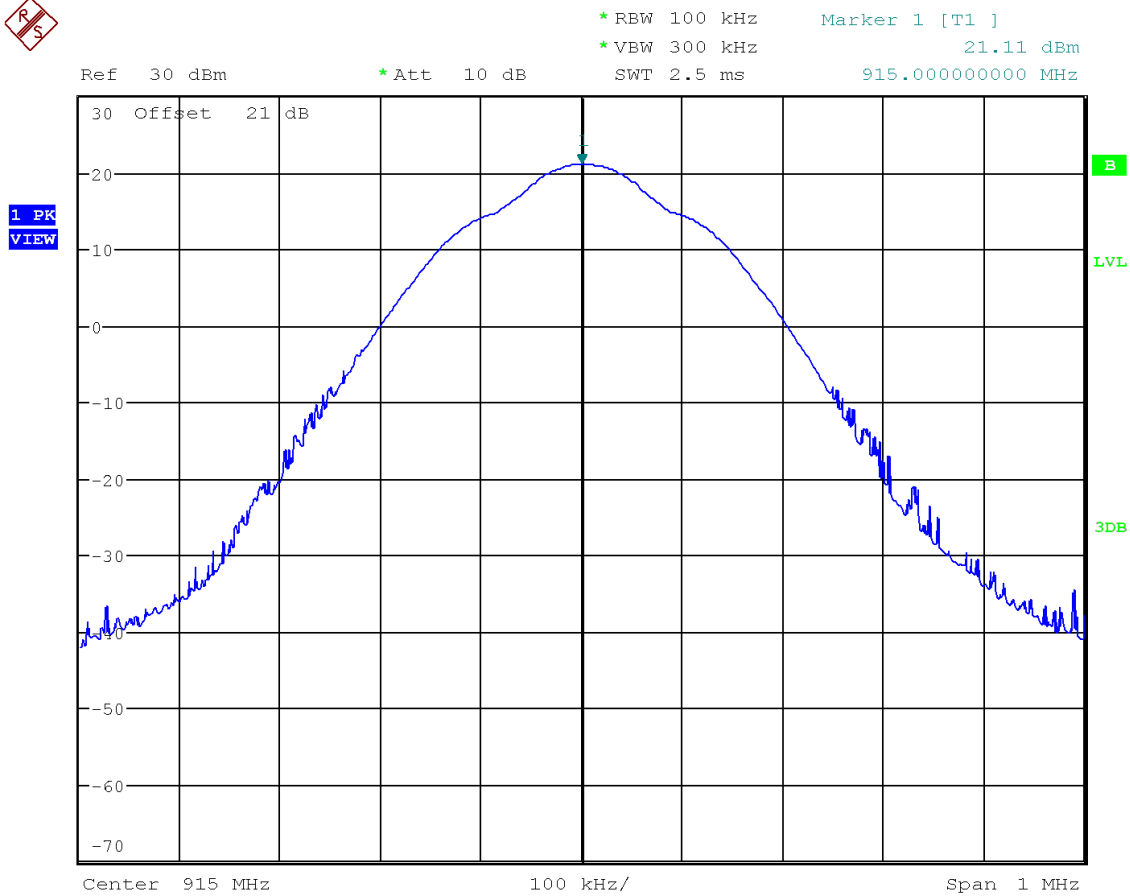
Figure 17. 915 MHz Reference
