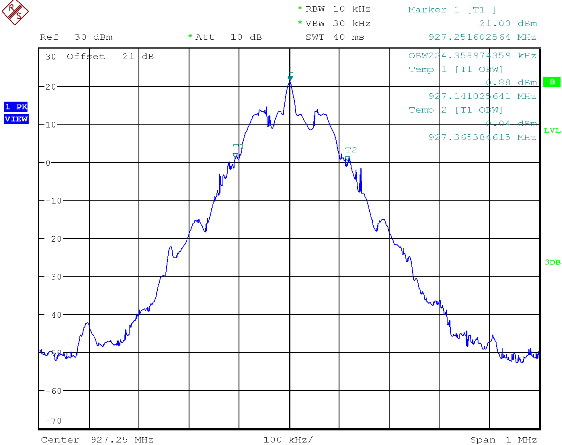
Figure 14 927.25 MHz, 99% Bandwidth
