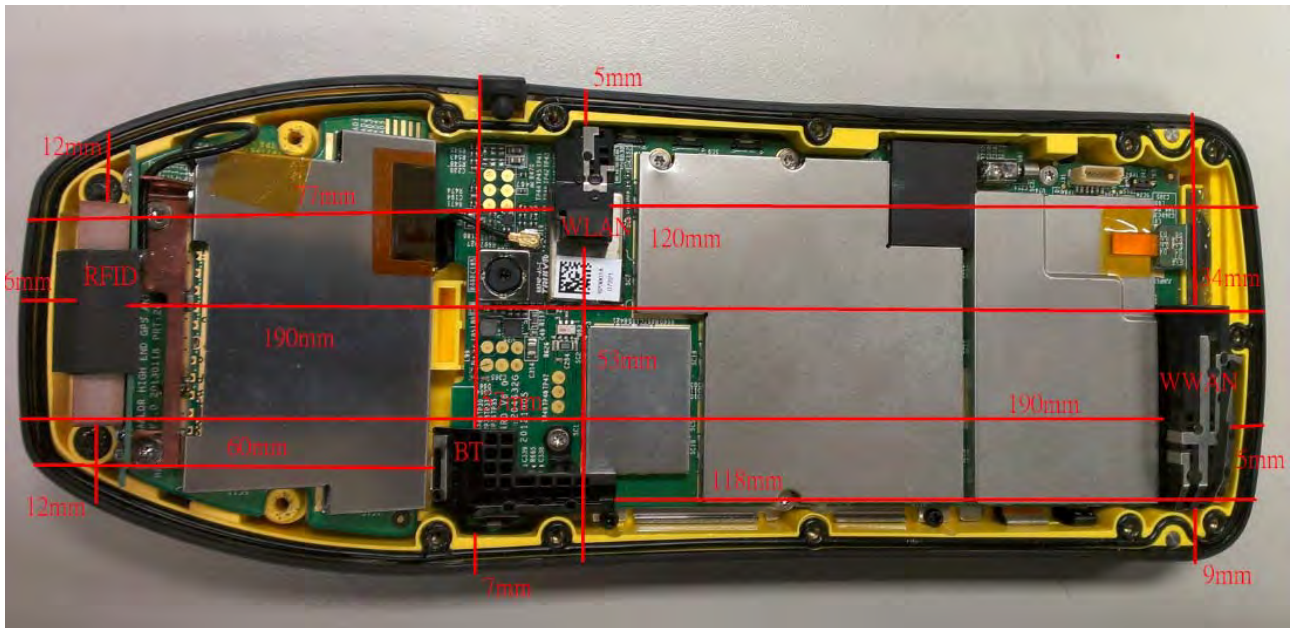
Fig.17 Antenna position of EUT
