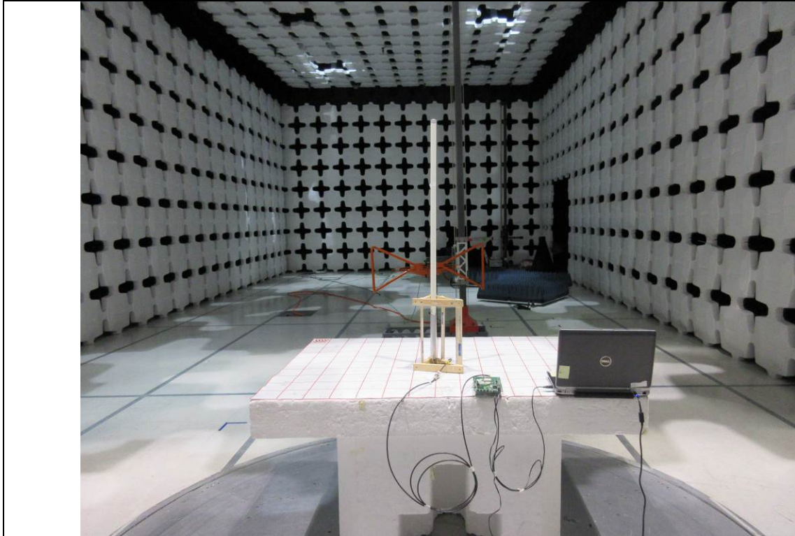
Radiated Emission Test below 1GHz Front View- Dipole Antenna
