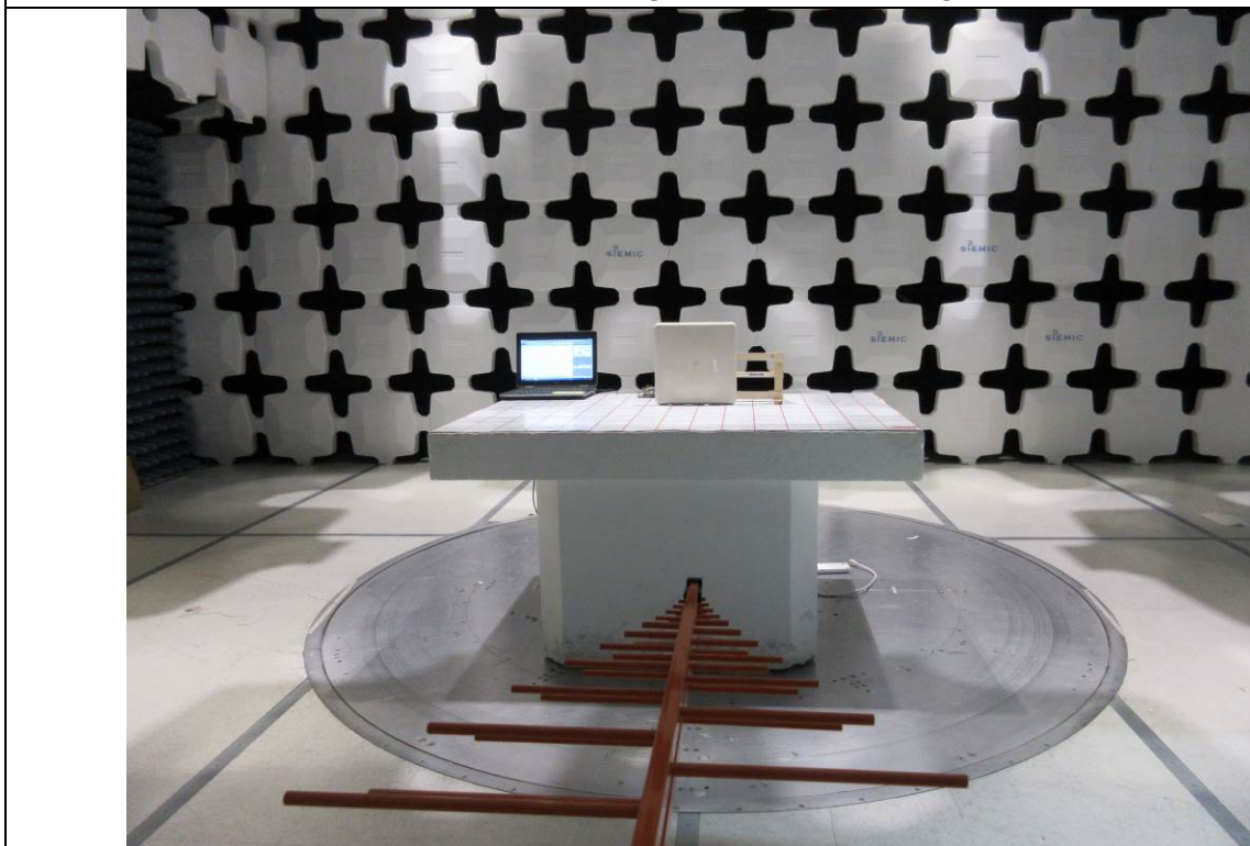
Radiated Emission Test below 1GHz Rear View- RHCP Patch Antenna
