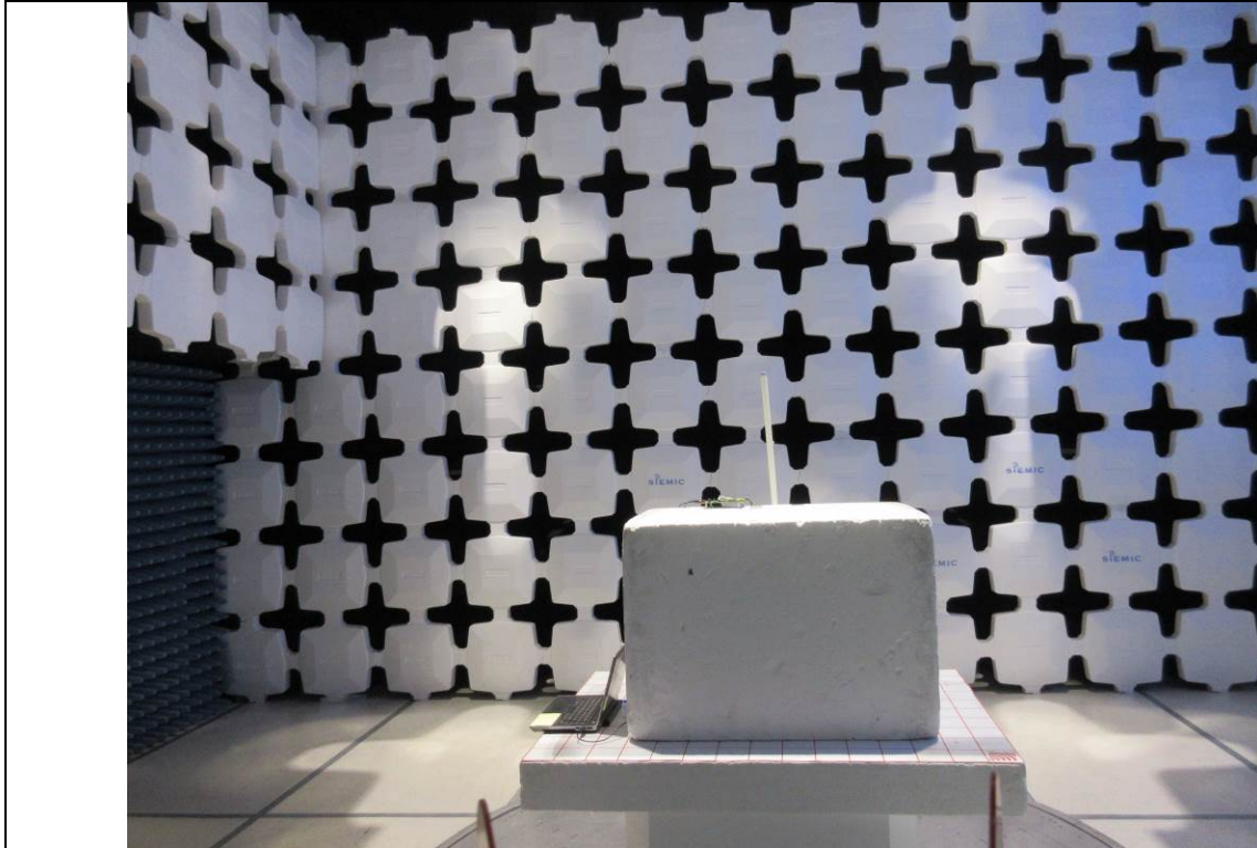
Radiated Emission Test above 1GHz Front View- Dipole Antenna
