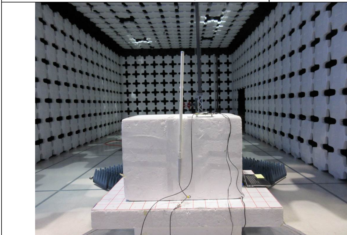
Radiated Emission Test above 1GHz Rear View- Dipole Antenna
