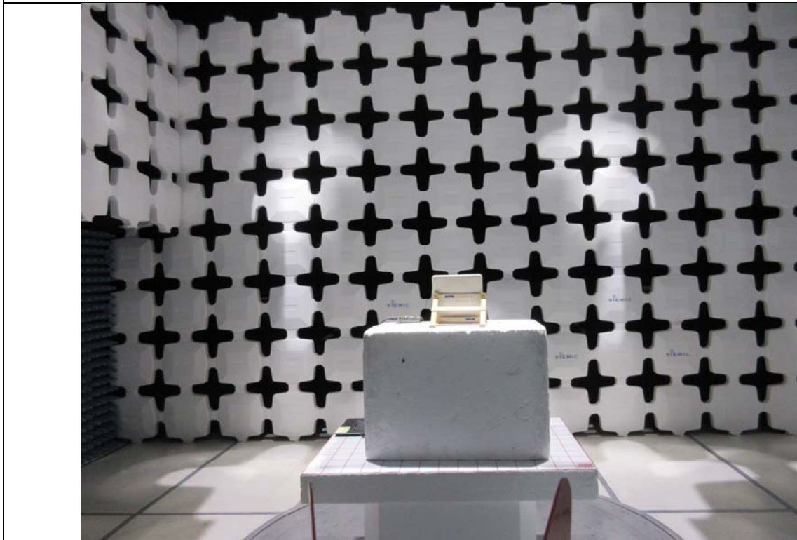
Radiated Emission Test above 1GHz Rear View- RHCP Patch Antenna
