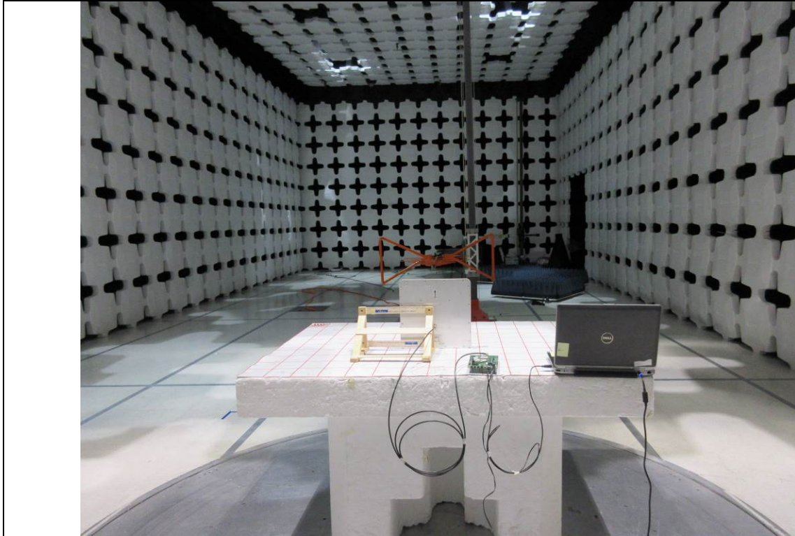
Radiated Emission Test below 1GHz Front View- RHCP Patch Antenna
