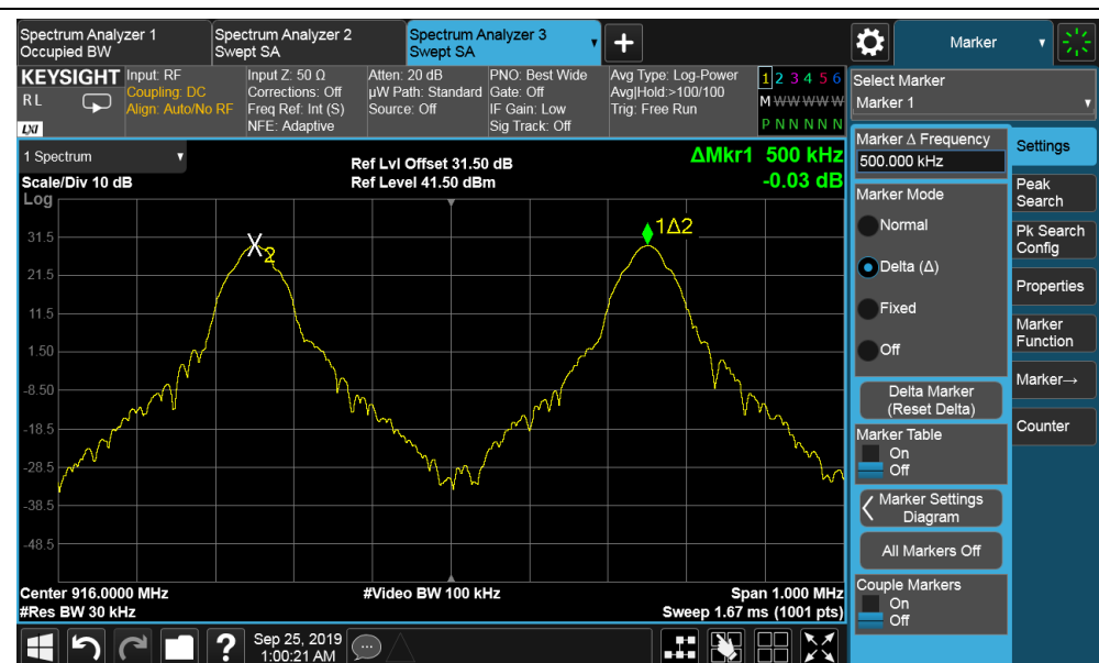
Middle Channel
