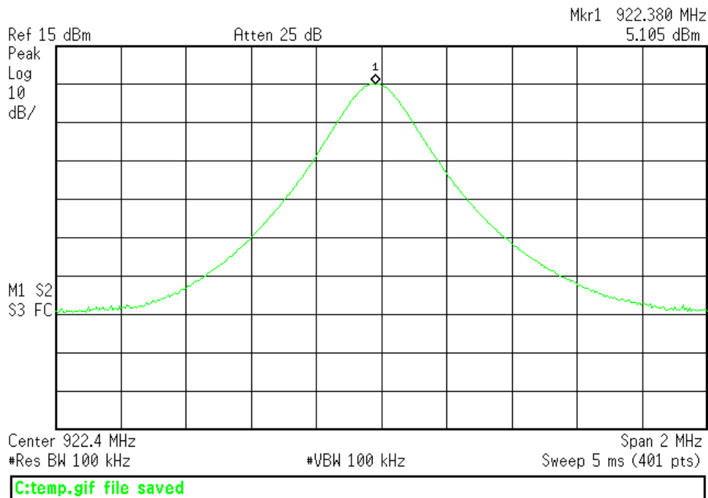
Output Power - Mid Channel
