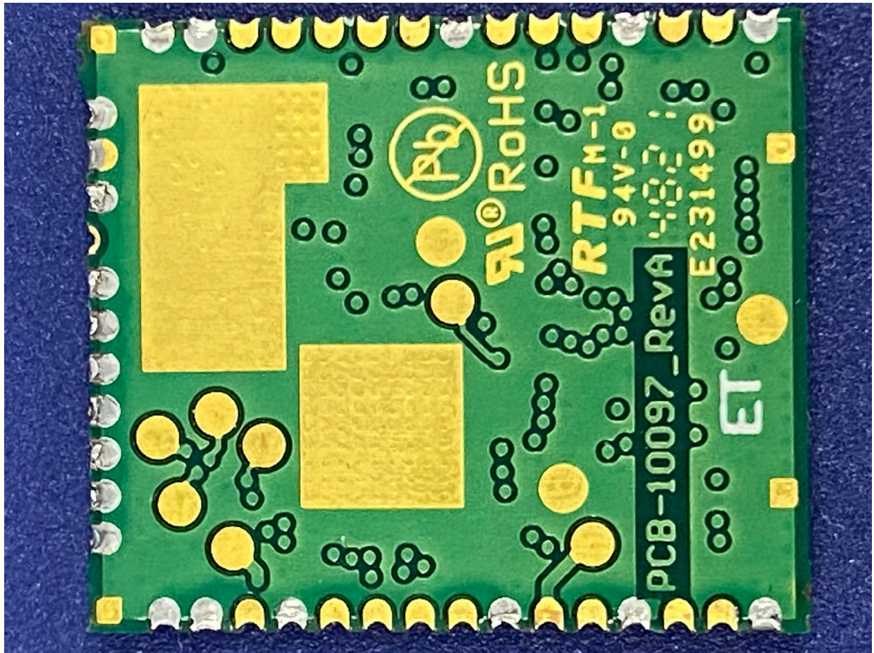
Bottom of PCB
