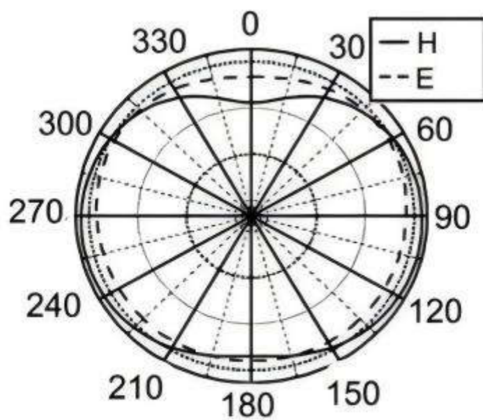
49.86 MHZ radiation pattern
