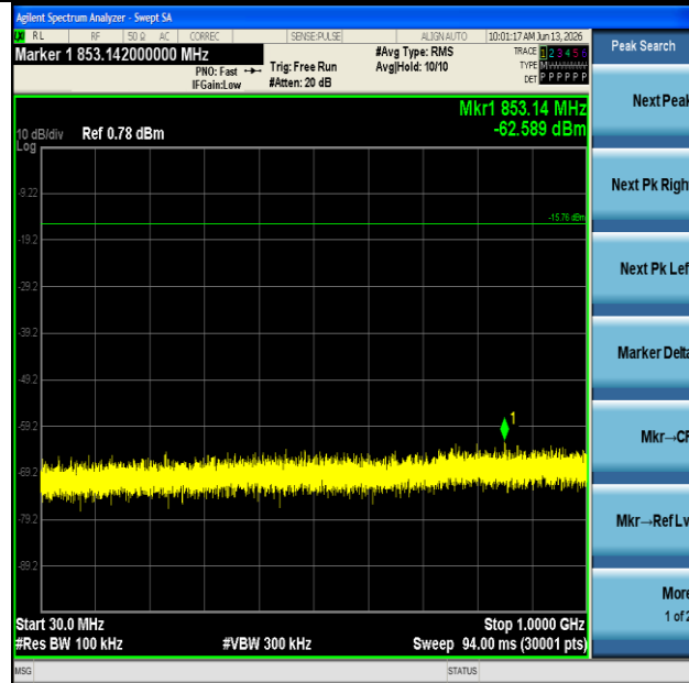
SRD-Ant1-2440-30~1000-PASS
