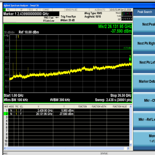
SRD-Ant1-2440-1000~26500-PASS
