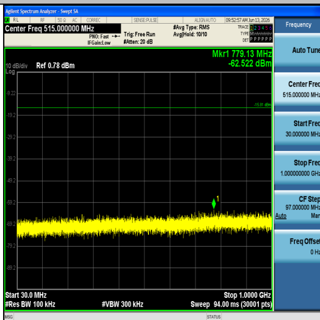
SRD-Ant1-2460-30~1000-PASS
