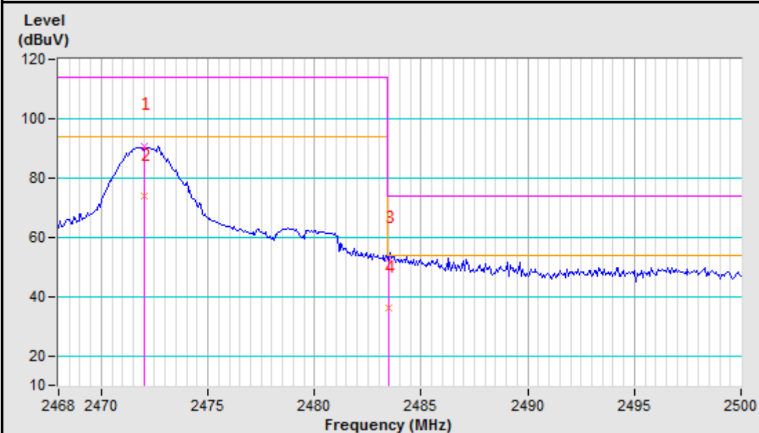
2472MHz Vertical
