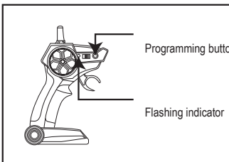
Fig 1. Hold down the programming button to enter programming mode
