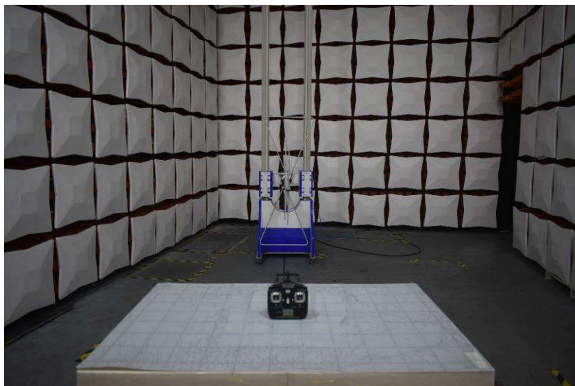
TX 30MHz~1GHz
