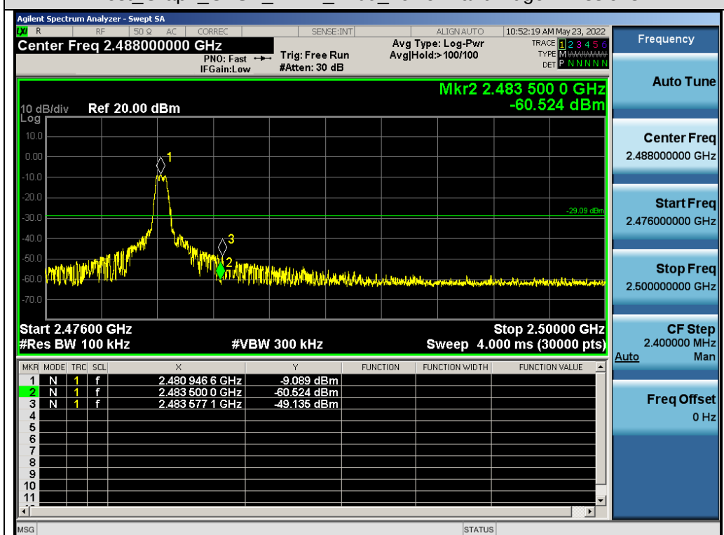
Test_Graph_GFSK_ANT1_2481_Higher Band Edge Emissions
