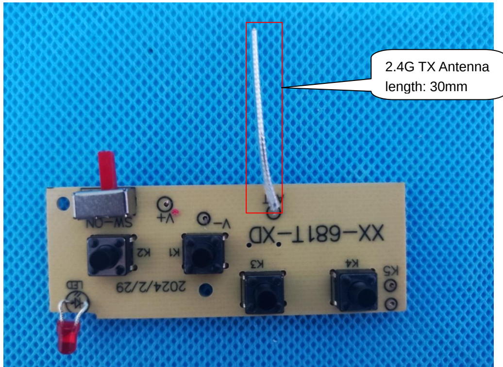
INTERNAL VIEW OF EUT (FIGURE 4)
