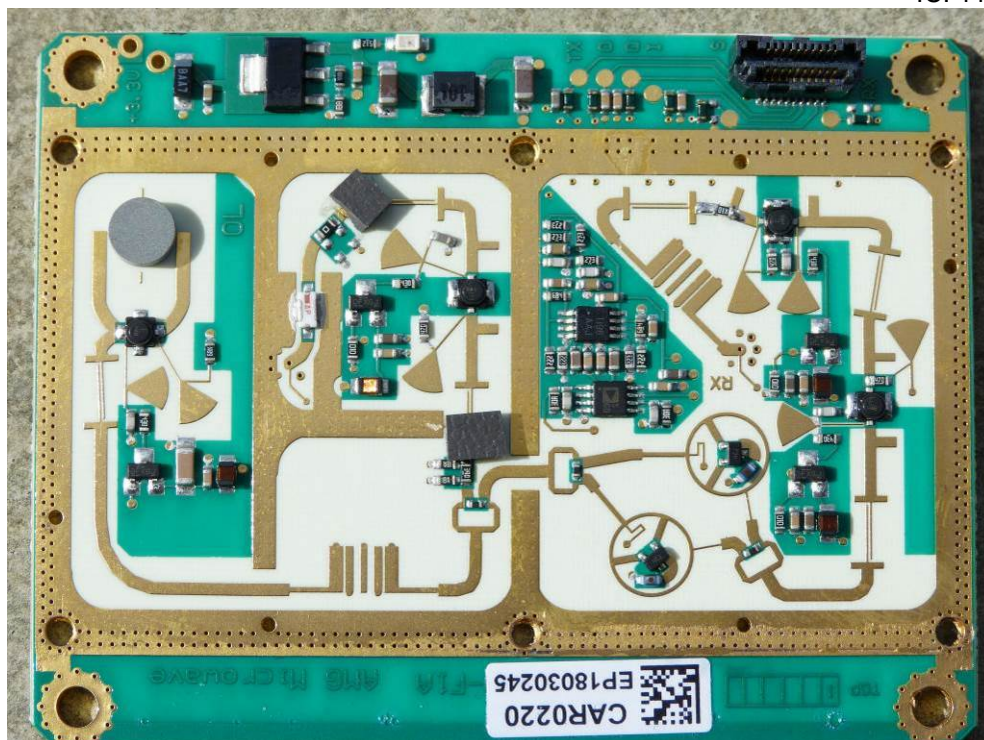
MW radar circuitry
