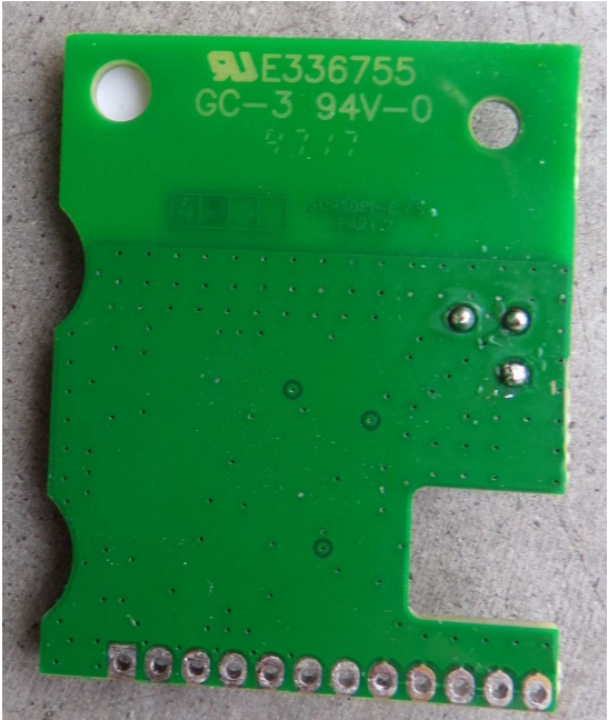
PIR detector board
