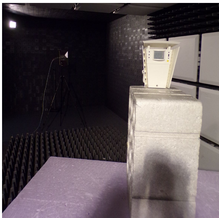
FAC setup (1GHz-18GHz / 3m)
