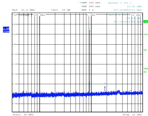
Figure 8.3-3: Conducted (TX 927 MHz)
