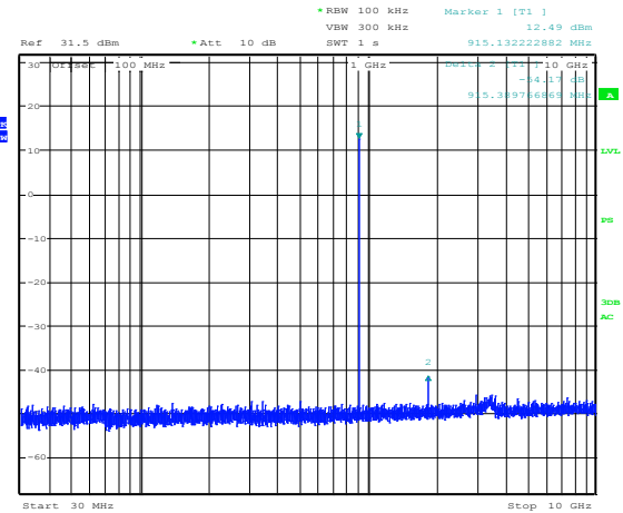
Figure 8.3-2: Conducted (TX 915 MHz)
