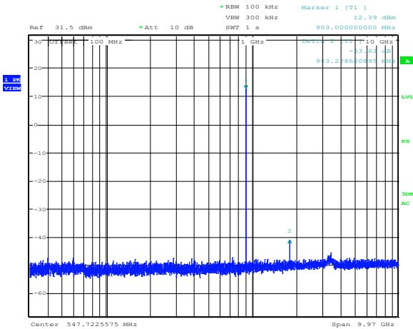
Figure 8.3-1: Conducted (TX 903 MHz)
