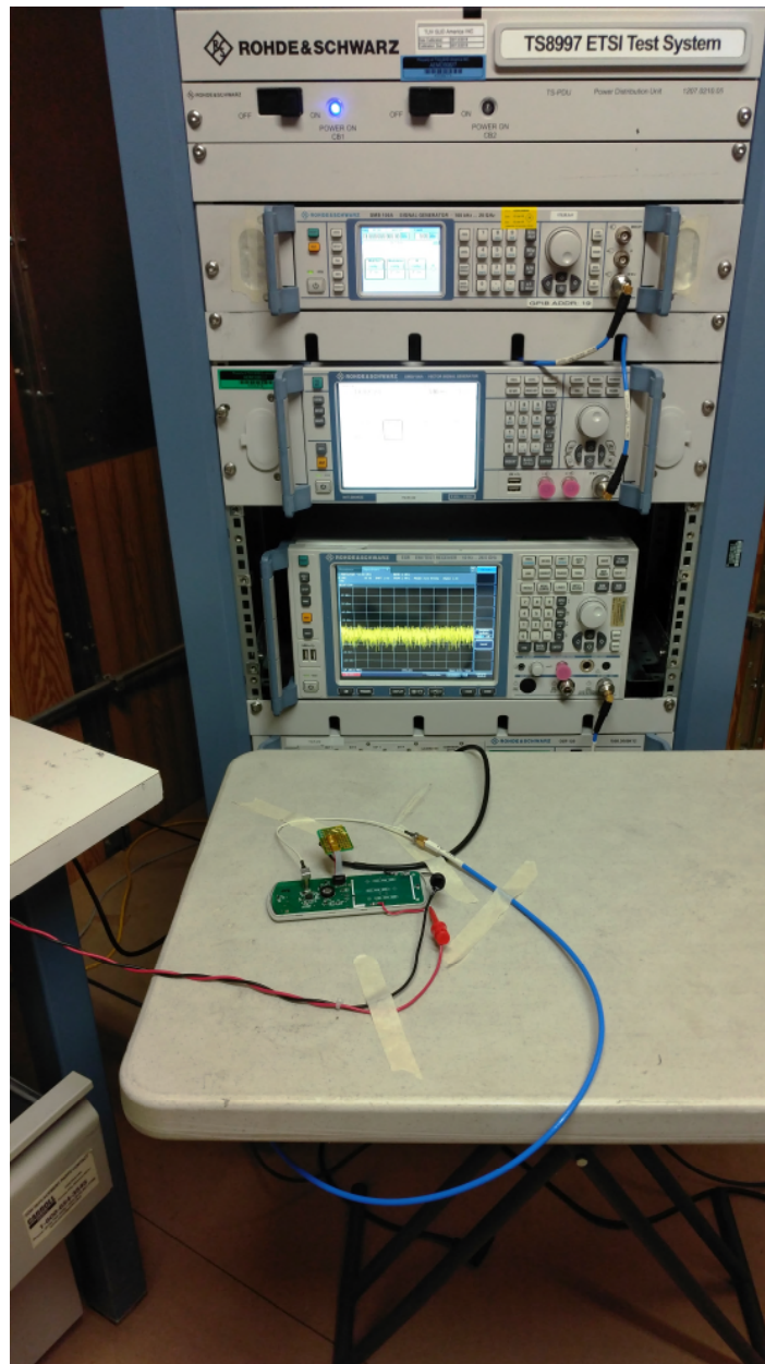
Figure 1: Equipment Under Test – Antenna Port Conducted Measurements
