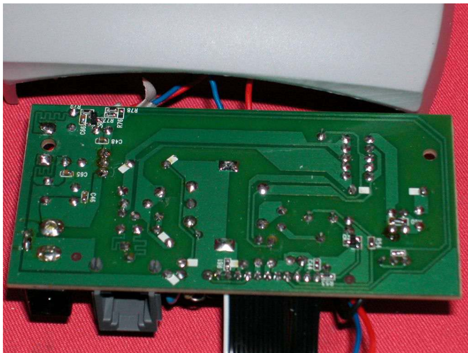
Base Line Interface PCB solder side
