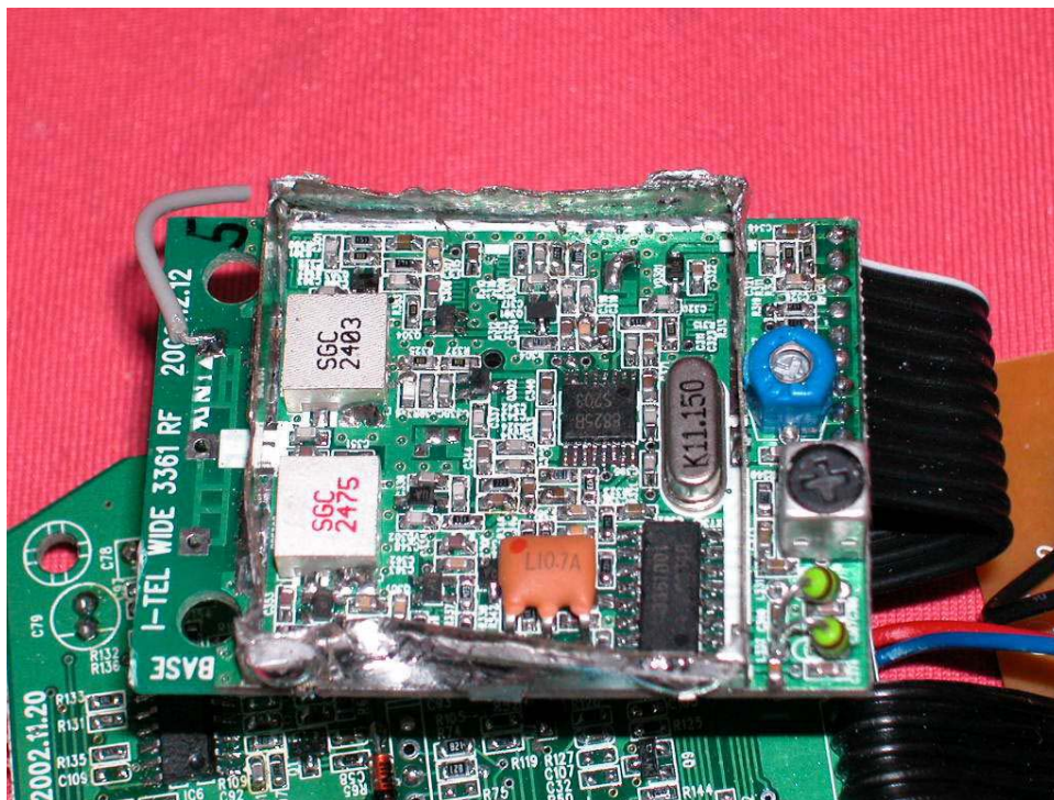
Base Oscillator PCB comp side (RF2)
