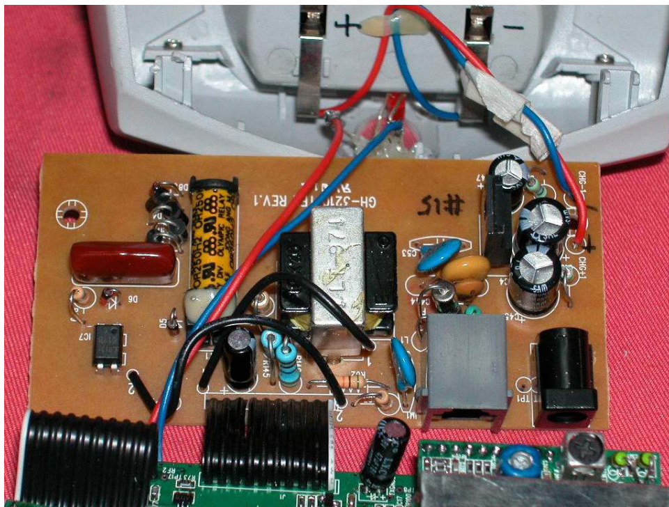
Base Line Interface PCB comp side
