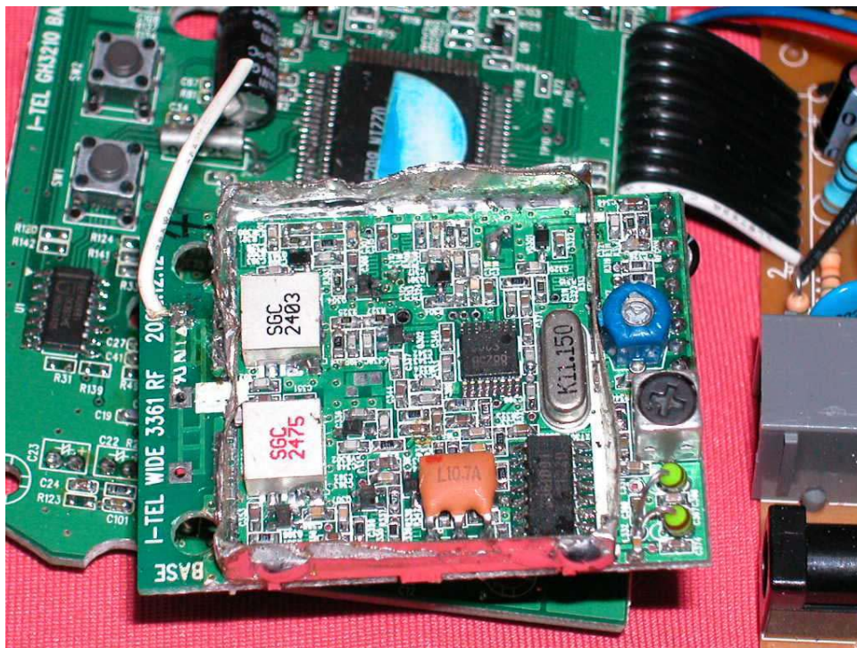
Base Oscillator PCB comp side (RF1)
