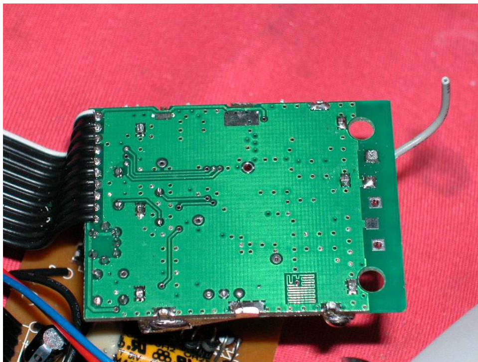
Base Oscillator PCB solder side (RF2)
