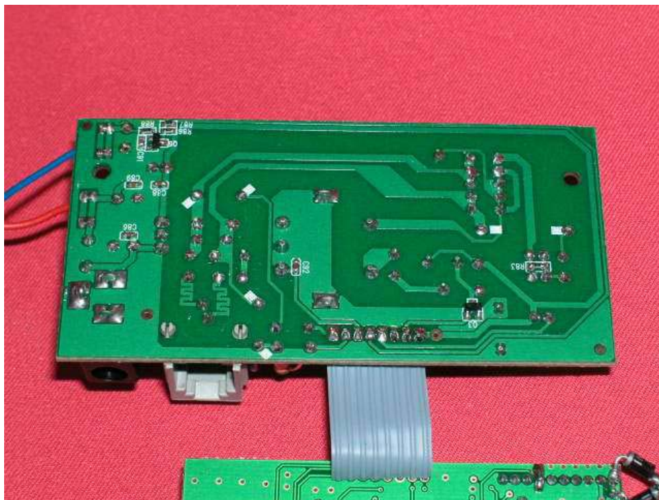
Base telephone line interface PCB solder side
