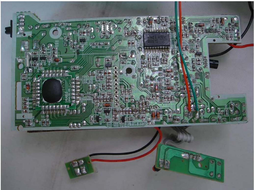
Main controller Rear
