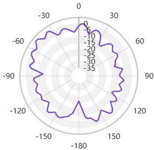
Free Space GAIN TOTAL (5820MHz) – YZ cut
