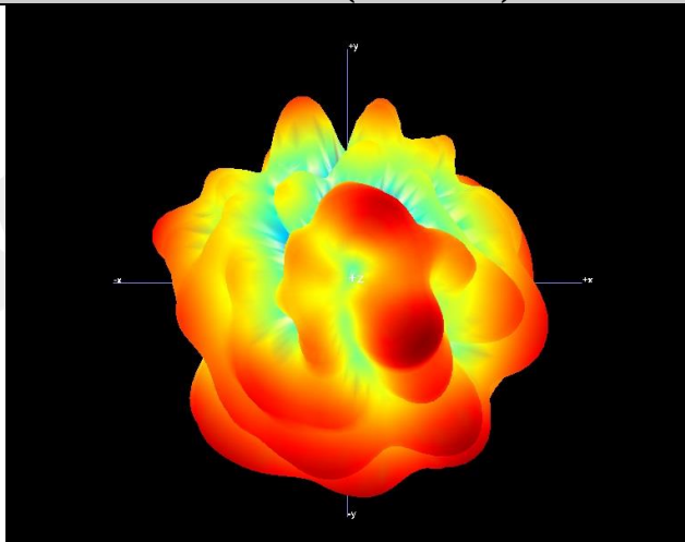
Free Space GAIN TOTAL (5500MHz) - 3D
