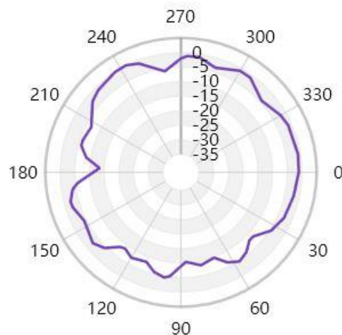
Free Space GAIN TOTAL (5500MHz) - YZ cut
