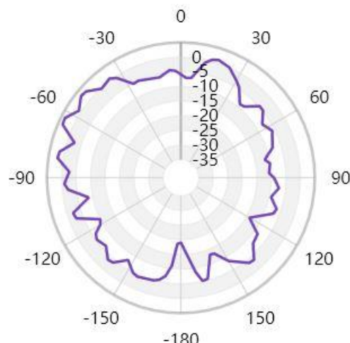
Free Space GAIN TOTAL (5500MHz) - YZ cut
