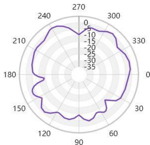
Free Space GAIN TOTAL (5820MHz) – XY cut
