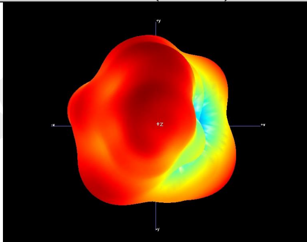
Free Space GAIN TOTAL (2440MHz) - 3D
