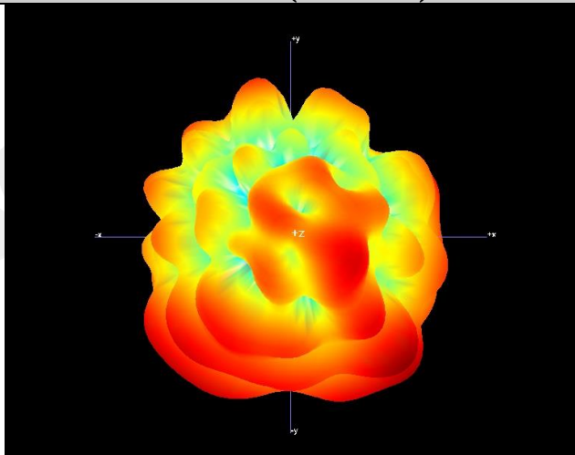
Free Space GAIN TOTAL (5820MHz) - 3D
