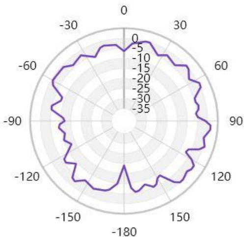
Free Space GAIN TOTAL (5500MHz) - XZ cut
