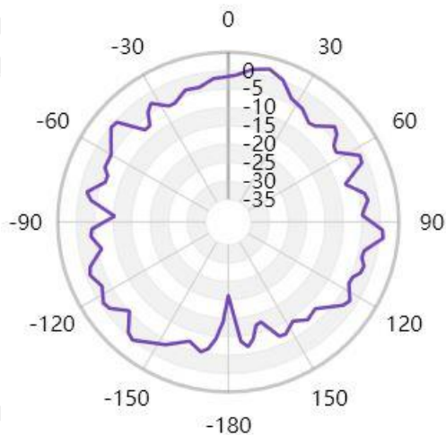
Free Space GAIN TOTAL (5820MHz) – XZ cut
