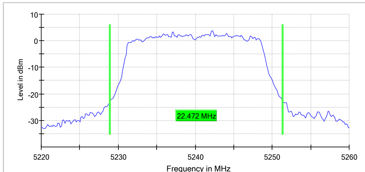
26 dB Bandwidth
