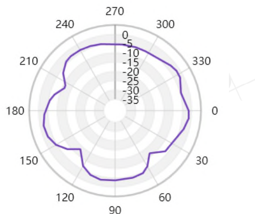
Free Space GAIN TOTAL (2440MHz) - XY cut
