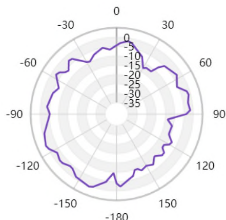
Free Space GAIN TOTAL (2440MHz) - YZ cut
