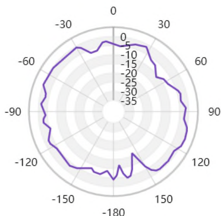
Free Space GAIN TOTAL (2440MHz) - XZ cut
