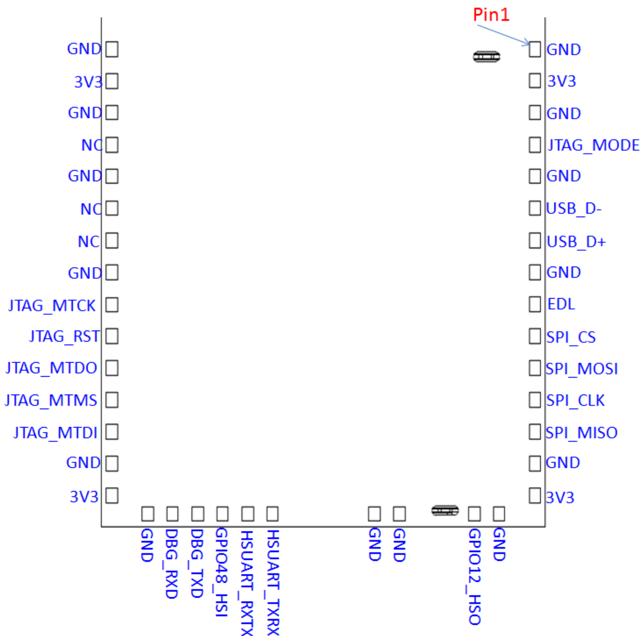
Pad diagram (Bottom View)
