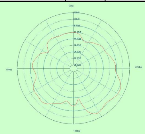
Free Space GAIN TOTAL (2480MHz) - YZ cut
