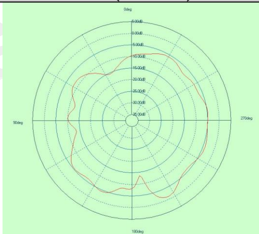
Free Space GAIN TOTAL (2480MHz) – XZ cut
