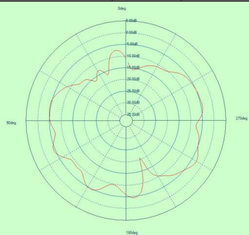
Free Space GAIN TOTAL (2480MHz) - XY cut
