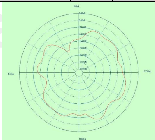
Free Space GAIN TOTAL (2440MHz) – XZ cut
