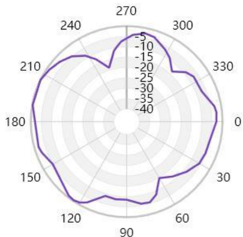
Free Space GAIN TOTAL (2440MHz) - XY cut
