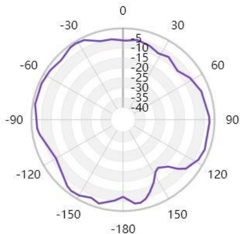
Free Space GAIN TOTAL (2440MHz) - XZ cut
