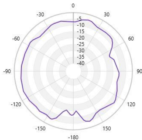
Free Space GAIN TOTAL (2480MHz) - YZ cut
