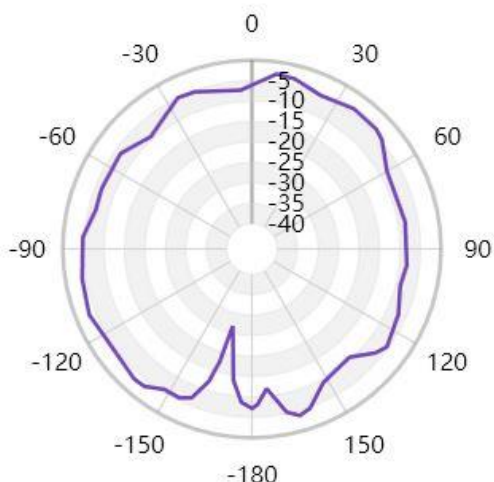
Free Space GAIN TOTAL (2440MHz) - YZ cut
