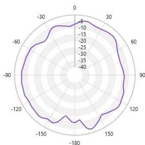
Free Space GAIN TOTAL (2440MHz) - YZ cut
