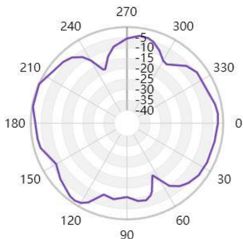
Free Space GAIN TOTAL (2480MHz) - XY cut
