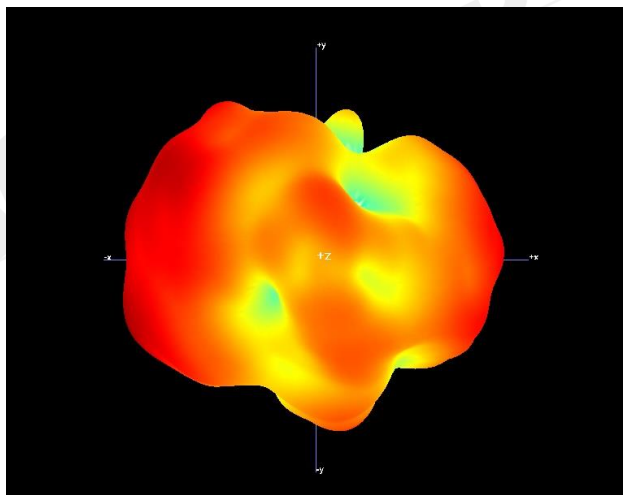
Free Space GAIN TOTAL (2480MHz) - 3D
