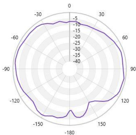
Free Space GAIN TOTAL (2480MHz) - XZ cut
