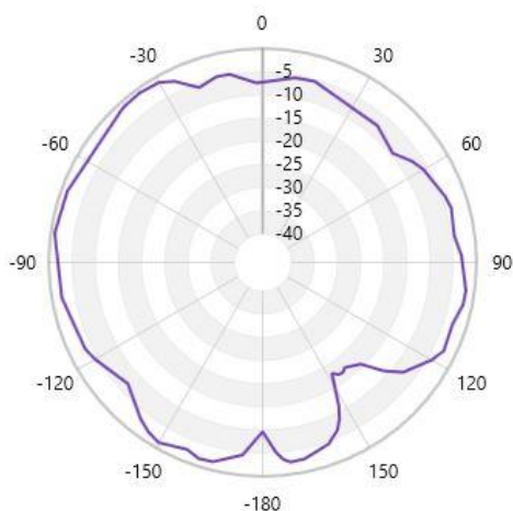
Free Space GAIN TOTAL (2440MHz) - XZ cut
