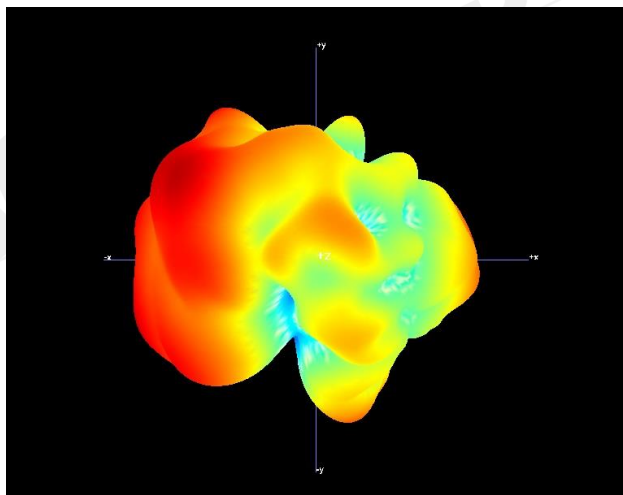
Free Space GAIN TOTAL (2440MHz) - 3D
