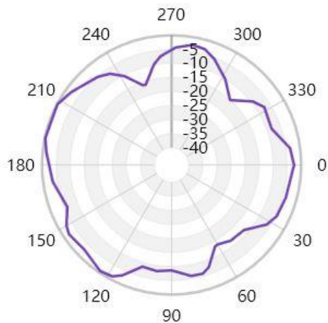
Free Space GAIN TOTAL (2440MHz) - XY cut
