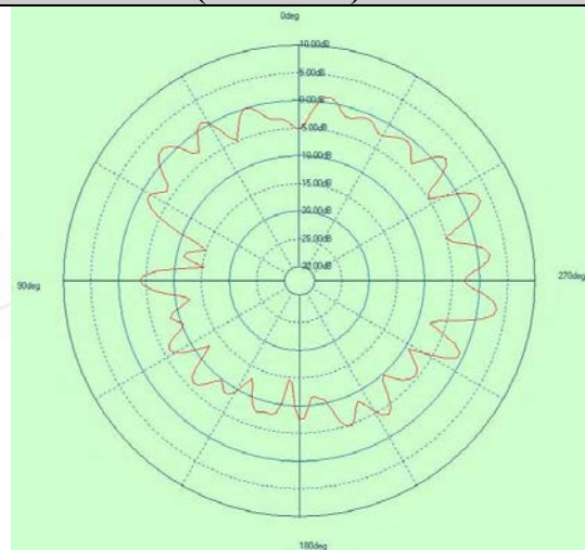
Free Space EIRP (5825MHz) - YZ cut
