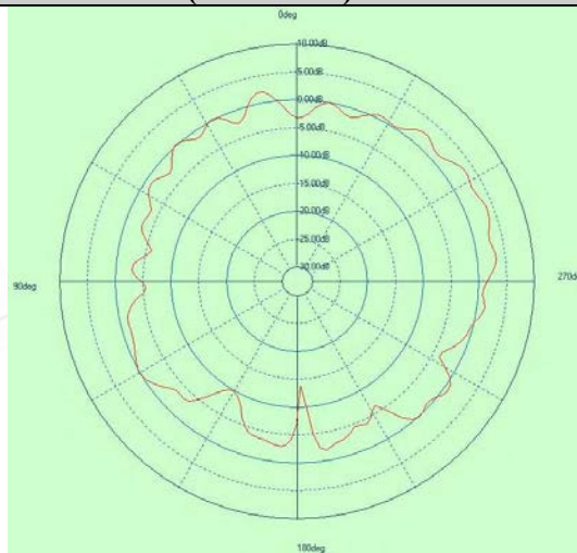
Free Space EIRP (2442MHz) – YZ cut
