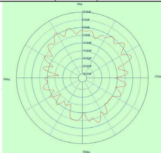
Free Space EIRP (5500MHz) - YZ cut
