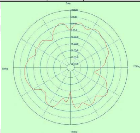
Free Space EIRP (2472MHz) - XZ cut
