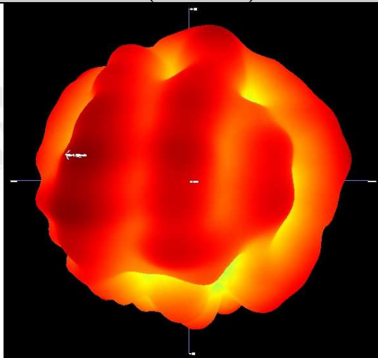
Free Space EIRP (2412MHz) - 3D
