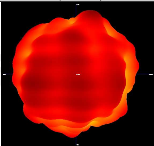
Free Space EIRP (2472MHz) - 3D
