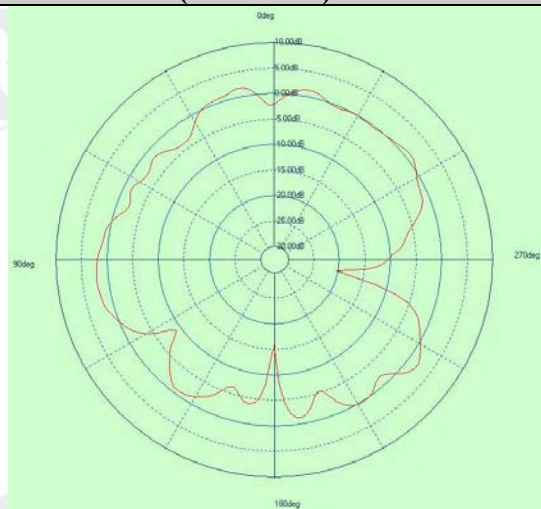
Free Space EIRP (2442MHz) - XZ cut
