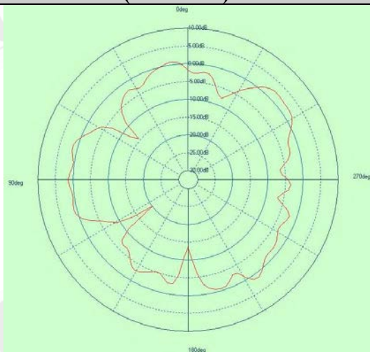
Free Space EIRP (2412MHz) - XZ cut
