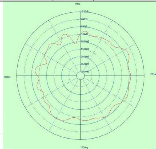
Free Space EIRP (2442MHz) - XY cut
