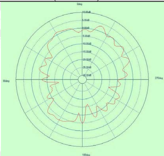
Free Space EIRP (5500MHz) - XZ cut
