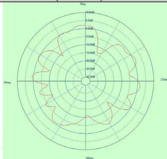
Free Space EIRP (2442MHz) - XY cut
