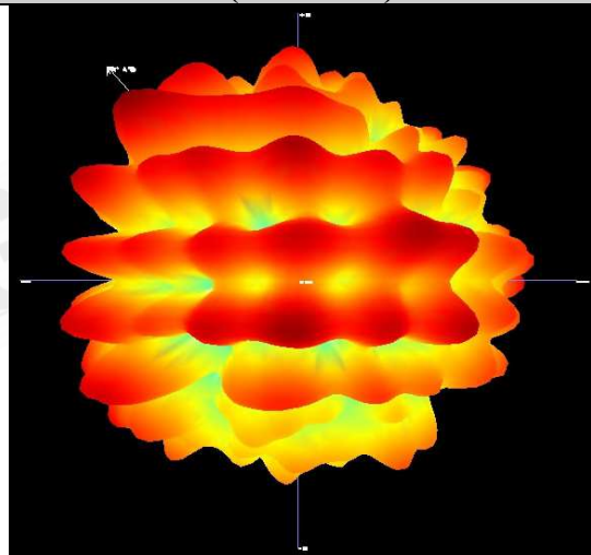
Free Space EIRP (5825MHz) - 3D
