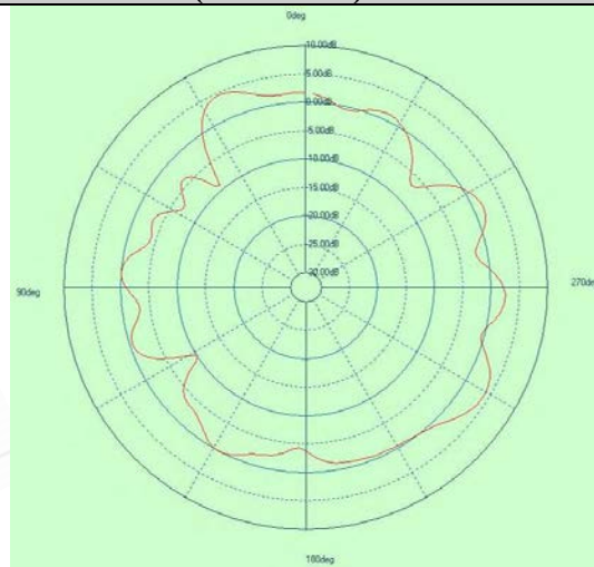
Free Space EIRP (2412MHz) - XY cut
