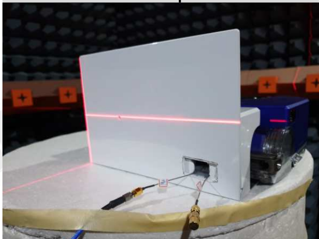
MAIN ANT with AUX ANT port terminated with 50 ohm, terminal with charging stand
