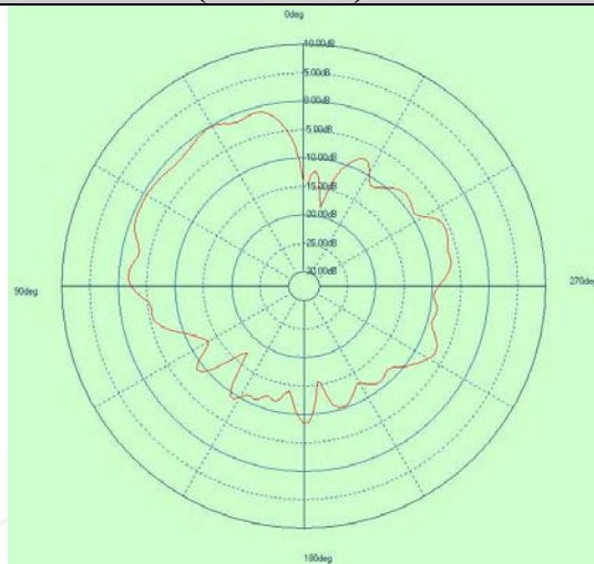
Free Space EIRP (5180MHz) – XY cut
