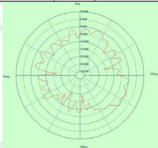
Free Space EIRP (5825MHz) - XZ cut
