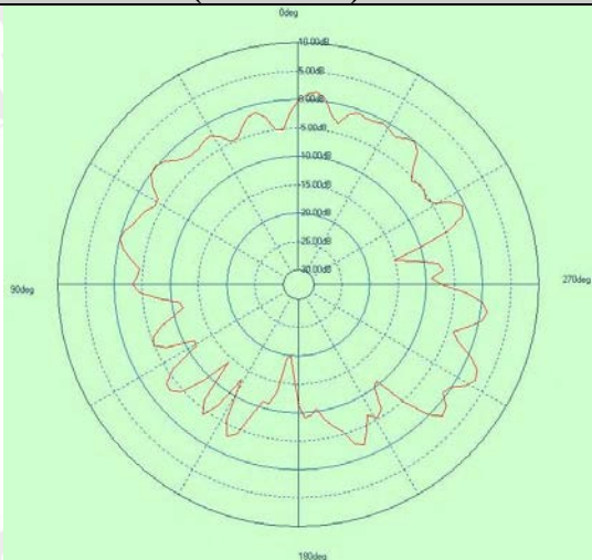
Free Space EIRP (5825MHz) - XZ cut
