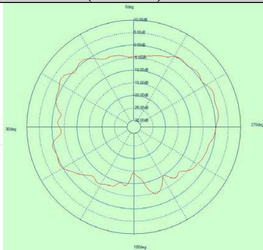
Free Space EIRP (2472MHz) - YZ cut
