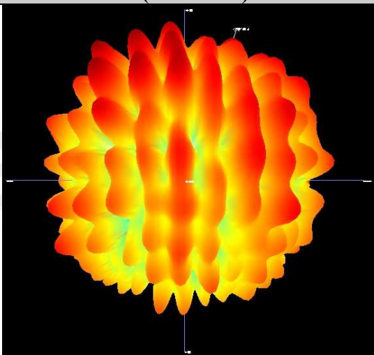
Free Space EIRP (5500MHz) - 3D
