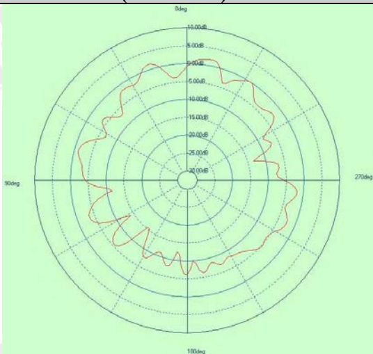
Free Space EIRP (5180MHz) - XZ cut
