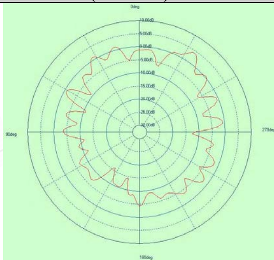
Free Space EIRP (5180MHz) - YZ cut
