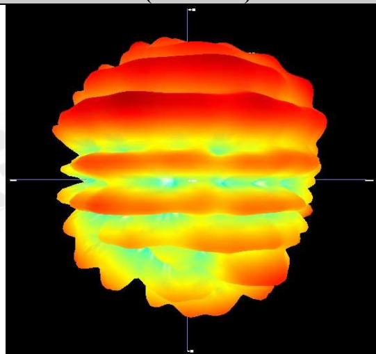
Free Space EIRP (5500MHz) - 3D
