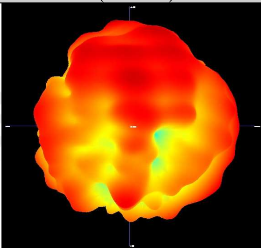
Free Space EIRP (2442MHz) - 3D
