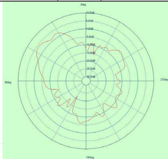
Free Space EIRP (5825MHz) - XY cut
