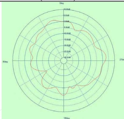
Free Space EIRP (2472MHz) – XY cut
