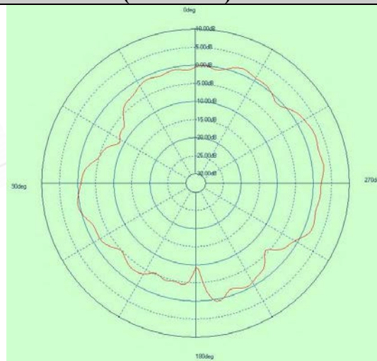
Free Space EIRP (2412MHz) - YZ cut
