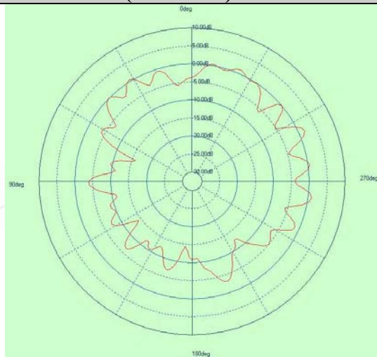
Free Space EIRP (5825MHz) - YZ cut
