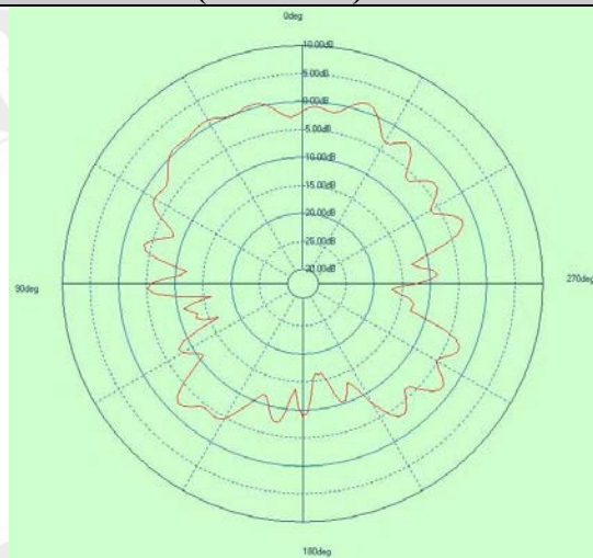
Free Space EIRP (5500MHz) - XZ cut
