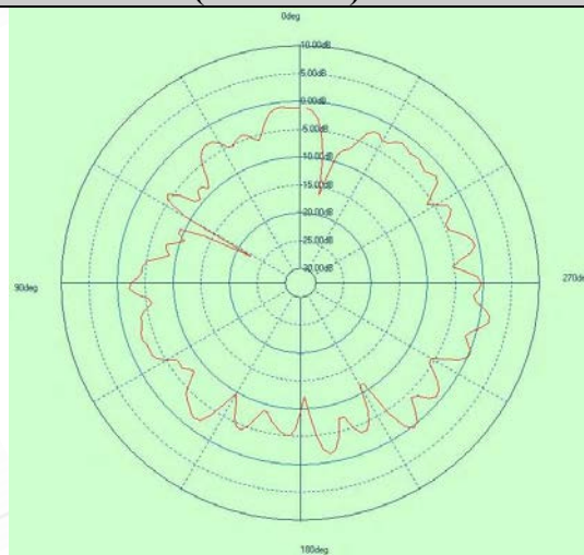
Free Space EIRP (5500MHz) - XY cut
