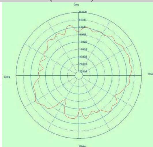
Free Space EIRP (2472MHz) – YZ cut
