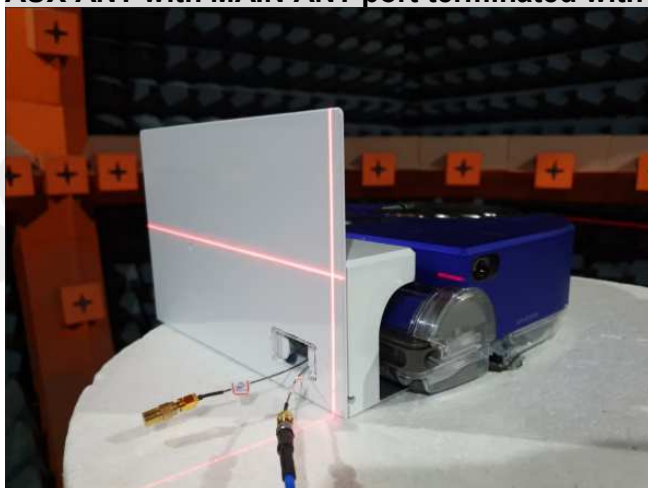
AUX ANT with MAIN ANT port terminated with 50 ohm, terminal with charging stand
