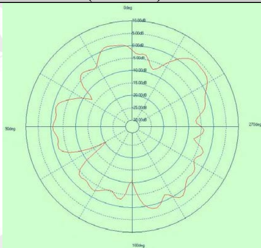
Free Space EIRP (2442MHz) - XZ cut
