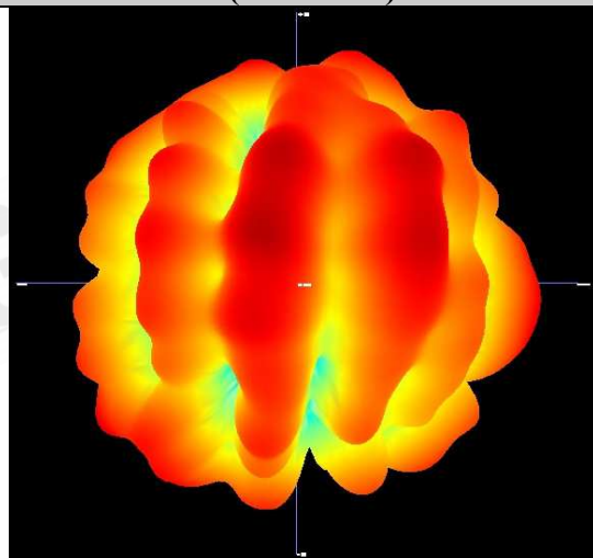
Free Space EIRP (2442MHz) - 3D
