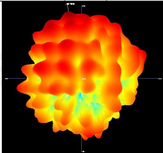
Free Space EIRP (5180MHz) - 3D
