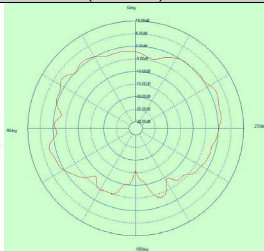
Free Space EIRP (2442MHz) - YZ cut
