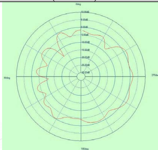
Free Space EIRP (2472MHz) - XY cut
