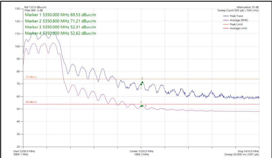
Figure 14 - HT20, 5300 MHz (CH60), Band Edge Frequency 5350 MHz
