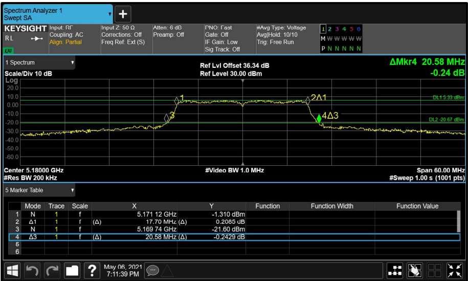
Figure 40 - Aux (B) 5180 MHz (CH36) 26 dB and 99% Bandwidth
