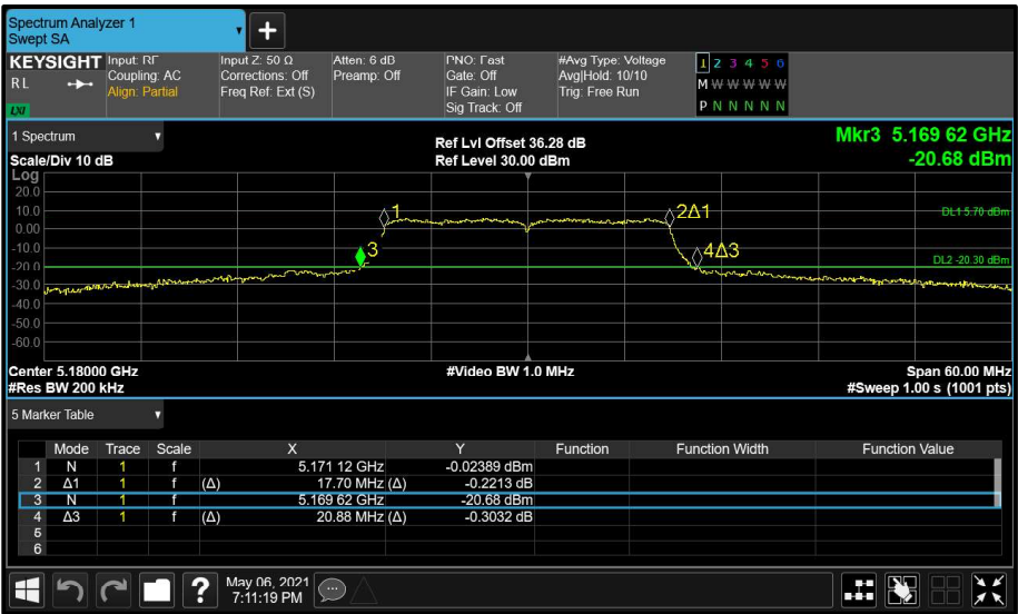
Figure 39 - Main (A) 5180 MHz (CH36) 26 dB and 99% Bandwidth
