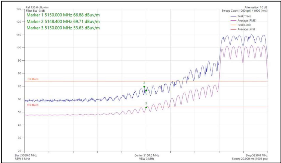
Figure 18 - HT40, 5230 MHz (CH46), Band Edge Frequency 5150 MHz
