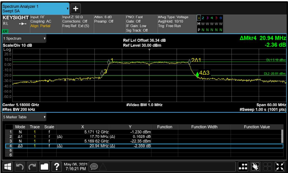
Figure 52 - Aux (B) 5180 MHz (CH36) 26 dB and 99% Bandwidth
