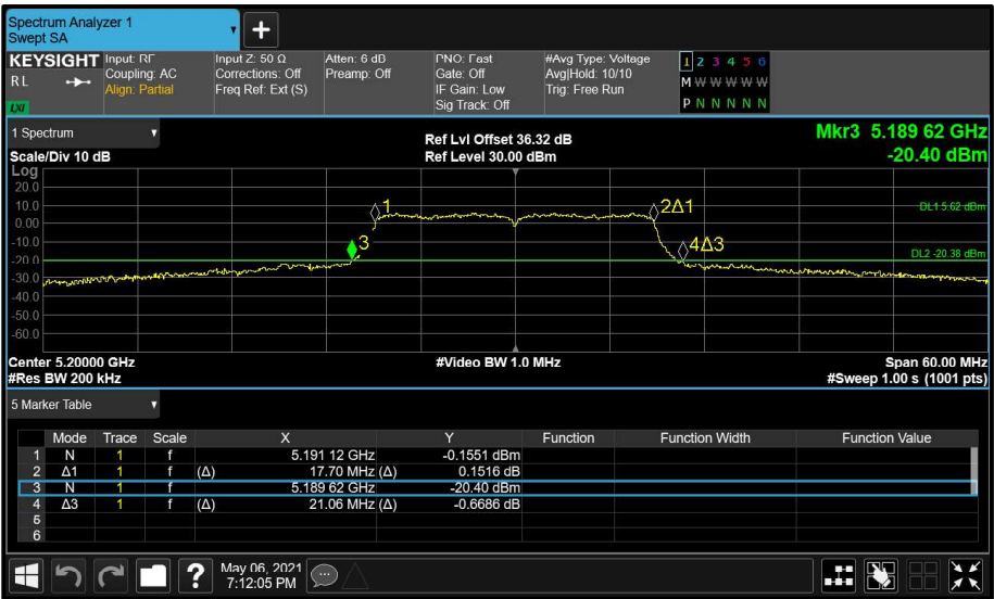
Figure 41 - Main (A) 5200 MHz (CH40) 26 dB and 99% Bandwidth
