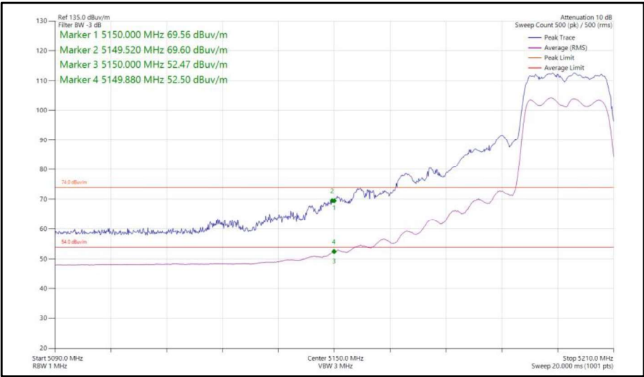
Figure 10 - HT20, 5200 MHz (CH40), Band Edge Frequency 5150 MHz
