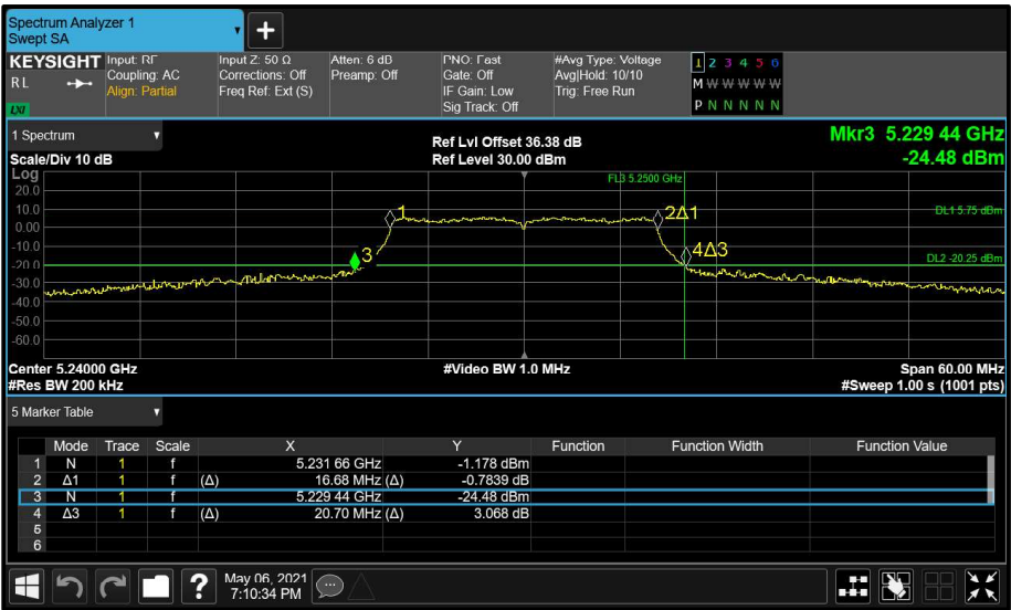
Figure 31 - Main (A) 5240 MHz (CH48) 26 dB and 99% Bandwidth
