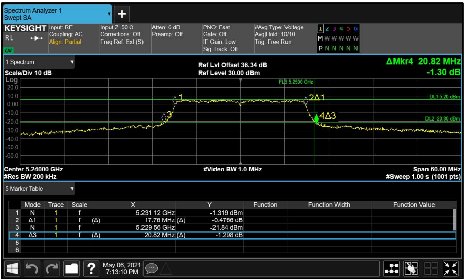
Figure 44 - Aux (B) 5240 MHz (CH48) 26 dB and 99% Bandwidth
