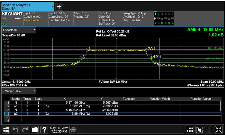
Figure 33 - Main (A) 5180 MHz (CH36) 26 dB and 99% Bandwidth
