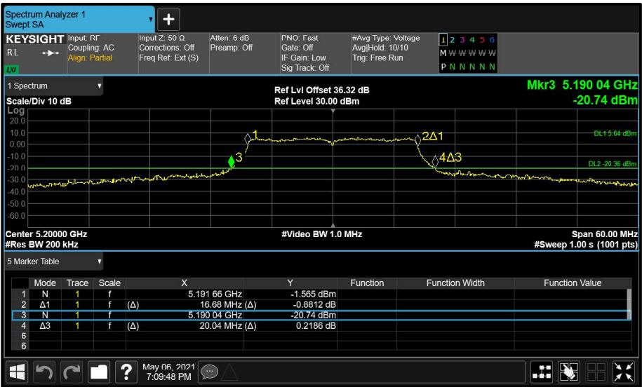
Figure 29 - Main (A) 5200 MHz (CH40) 26 dB and 99% Bandwidth
