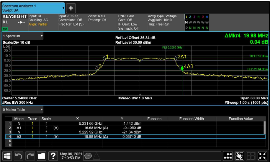
Figure 32 - Aux (B) 5240 MHz (CH48) 26 dB and 99% Bandwidth
