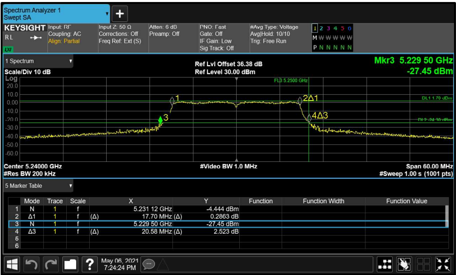
Figure 49 - Main (A) 5240 MHz (CH48) 26 dB and 99% Bandwidth
