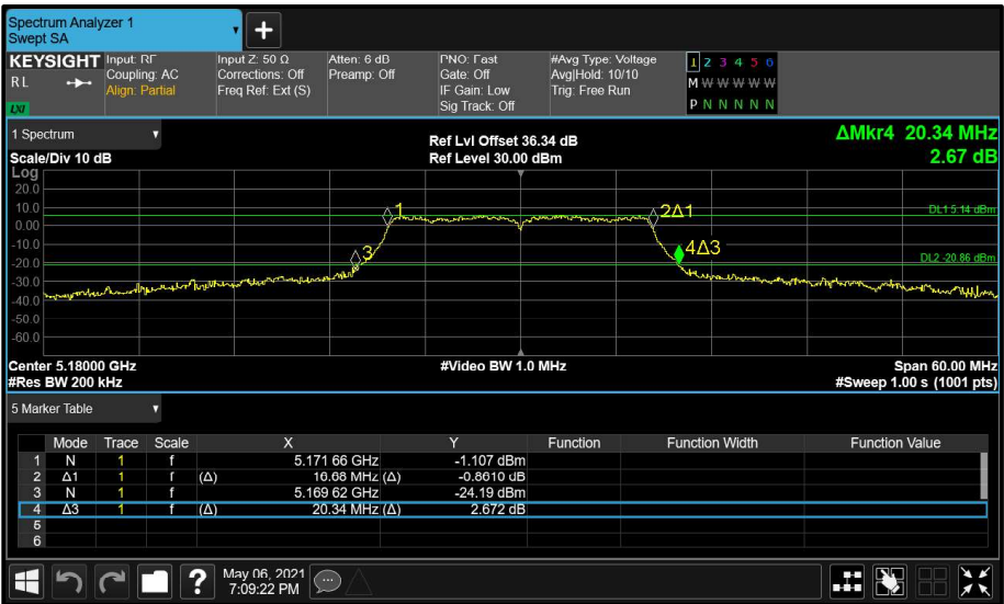
Figure 28 - Aux (B) 5180 MHz (CH36) 26 dB and 99% Bandwidth
