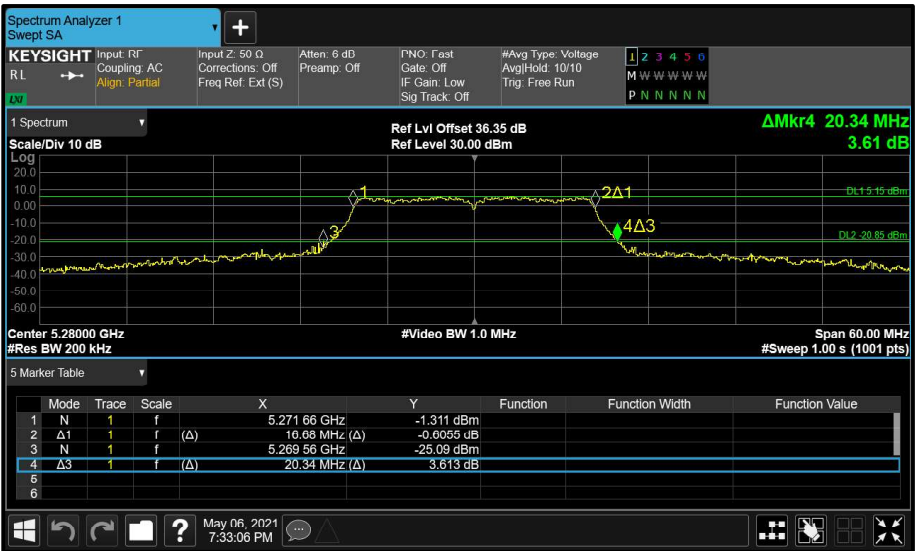
Figure 90 - Aux (B) 5280 MHz (CH56) 26 dB and 99% Bandwidth
