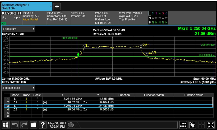
Figure 87 - Main (A) 5260 MHz (CH52) 26 dB and 99% Bandwidth
