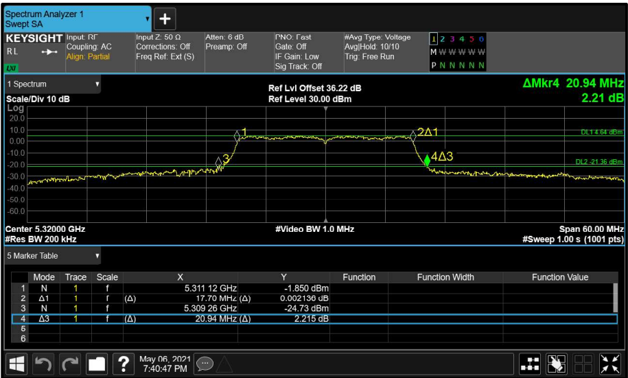
Figure 104 - Aux (B) 5320 MHz (CH64) 26 dB and 99% Bandwidth
