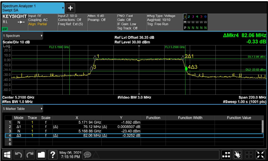
Figure 79 - Main (A) 5210 MHz (CH42) 26 dB and 99% Bandwidth
