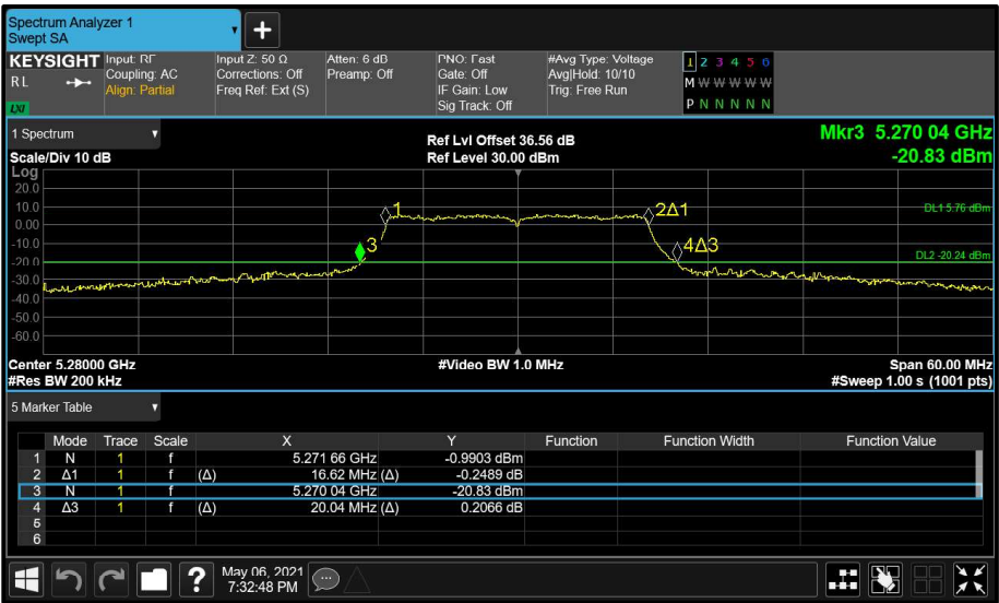
Figure 89 - Main (A) 5280 MHz (CH56) 26 dB and 99% Bandwidth
