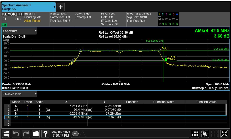
Figure 78 - Aux (B) 5230 MHz (CH46) 26 dB and 99% Bandwidth
