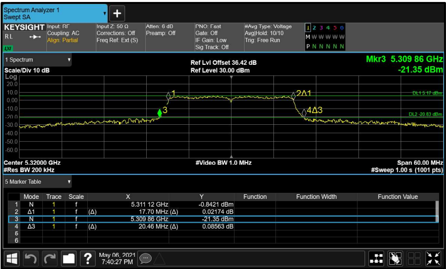
Figure 103 - Main (A) 5320 MHz (CH64) 26 dB and 99% Bandwidth
