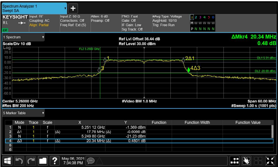
Figure 94 - Aux (B) 5260 MHz (CH52) 26 dB and 99% Bandwidth
