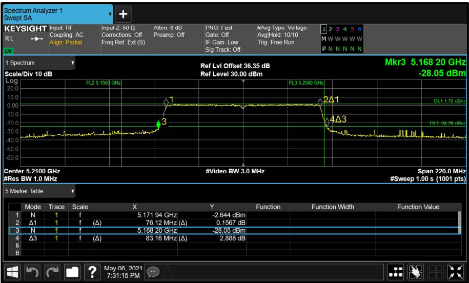
Figure 85 - Main (A) 5210 MHz (CH42) 26 dB and 99% Bandwidth
