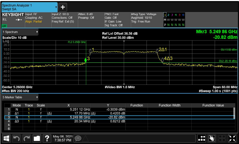
Figure 99 - Main (A) 5260 MHz (CH52) 26 dB and 99% Bandwidth
