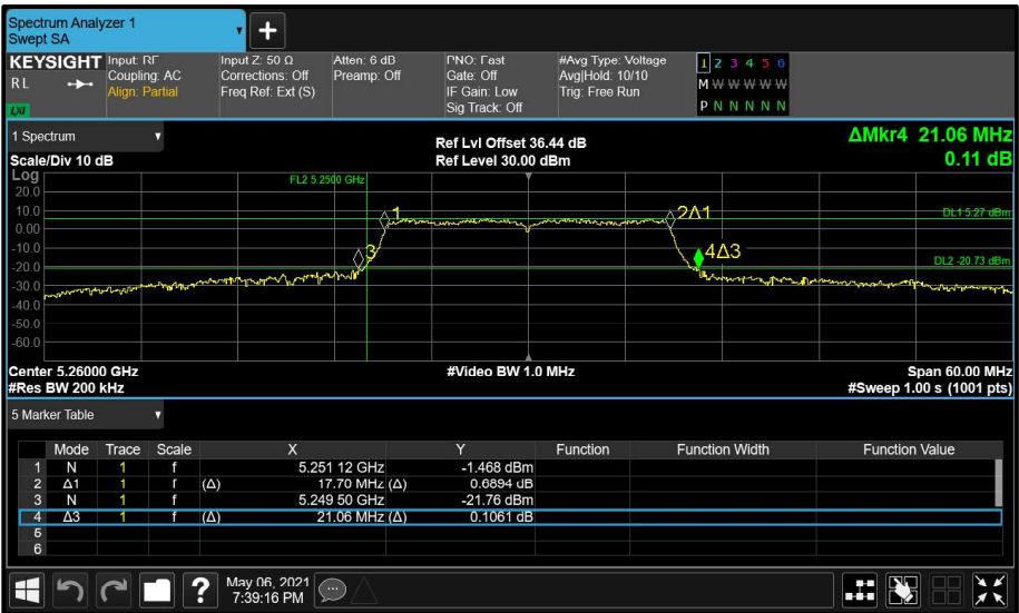
Figure 100 - Aux (B) 5260 MHz (CH52) 26 dB and 99% Bandwidth
