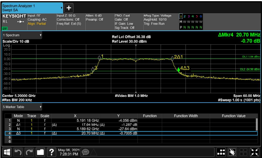
Figure 60 - Aux (B) 5200 MHz (CH40) 26 dB and 99% Bandwidth
