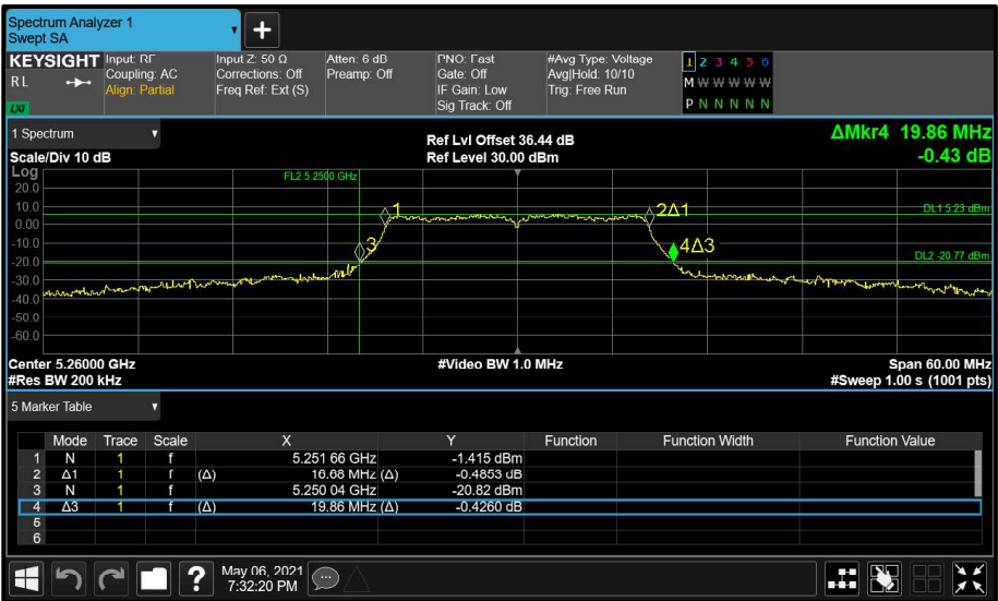
Figure 88 - Aux (B) 5260 MHz (CH52) 26 dB and 99% Bandwidth
