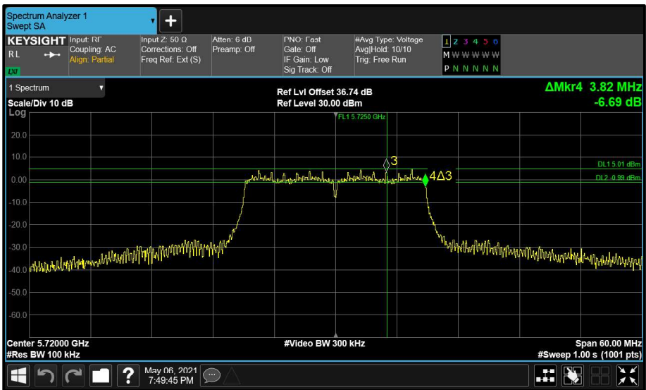
Figure 186 - Main (A) 5720 MHz (CH144) 6 dB Bandwidth
