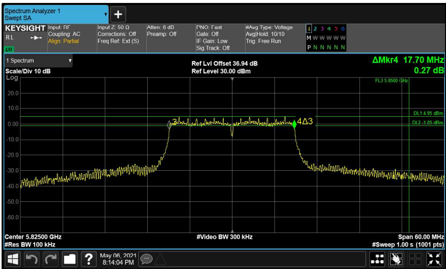
Figure 198 - Main (A) 5825 MHz (CH165) 6 dB Bandwidth
