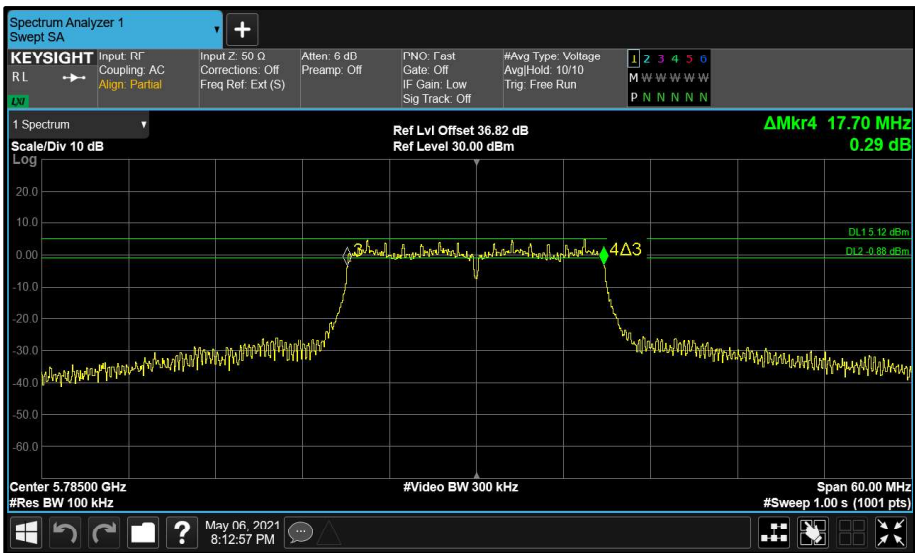
Figure 194 - Main (A) 5785 MHz (CH157) 6 dB Bandwidth
