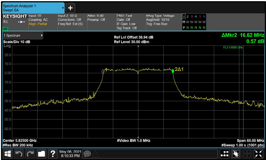
Figure 181 - Main (A) 5825 MHz (CH165) 99% Bandwidth
