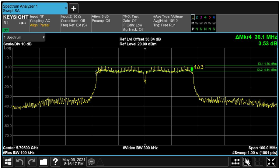
Figure 226 - Main (A) 5795 MHz (CH159) 6 dB Bandwidth
