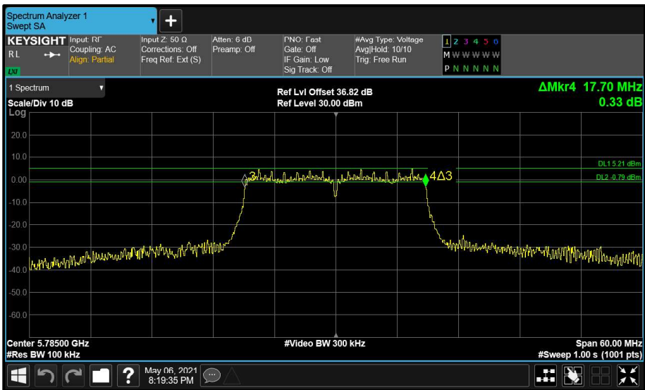
Figure 210 - Main (A) 5785 MHz (CH157) 6 dB Bandwidth
