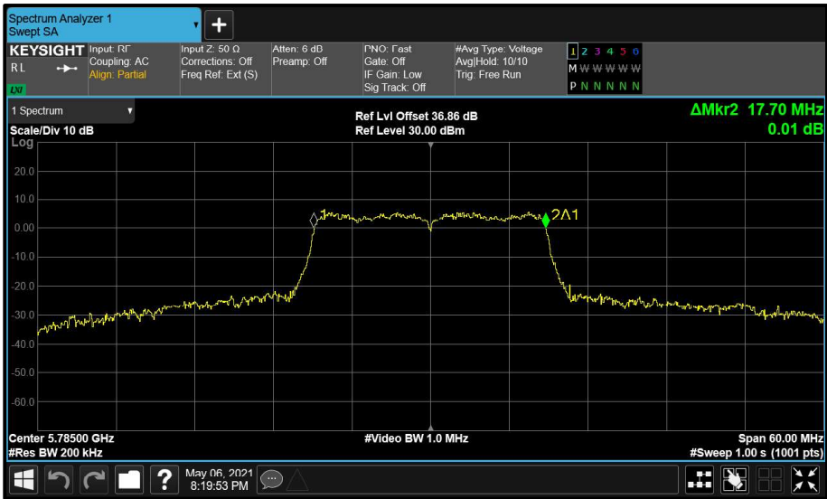
Figure 211 - Aux (B) 5785 MHz (CH157) 99% Bandwidth
