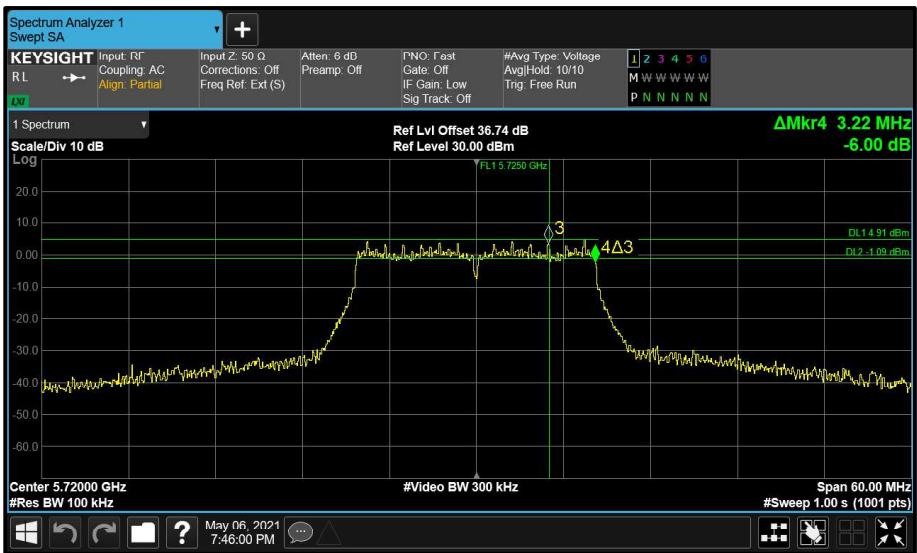
Figure 170 - Main (A) 5720 MHz (CH144) 6 dB Bandwidth
