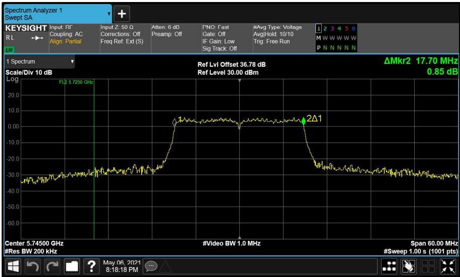
Figure 205 - Main (A) 5745 MHz (CH149) 99% Bandwidth
