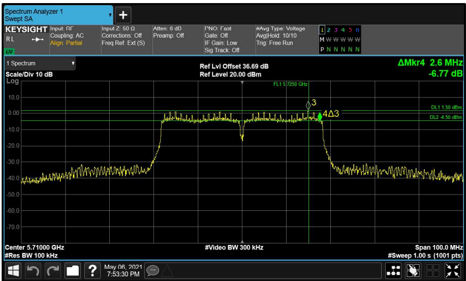
Figure 218 - Main (A) 5710 MHz (CH142) 6 dB Bandwidth
