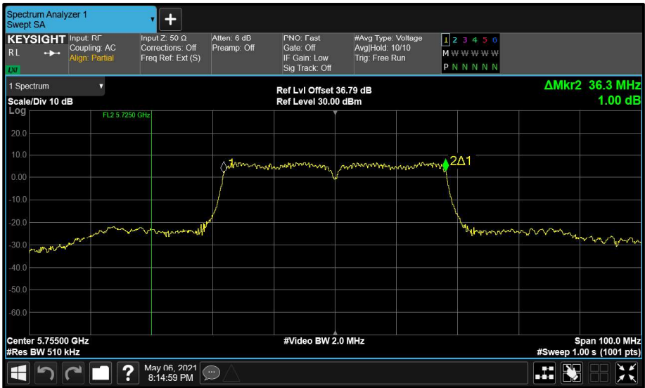
Figure 221 - Main (A) 5755 MHz (CH151) 99% Bandwidth
