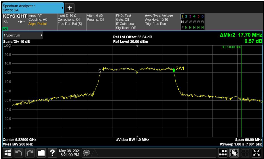
Figure 215 - Aux (B) 5825 MHz (CH165) 99% Bandwidth
