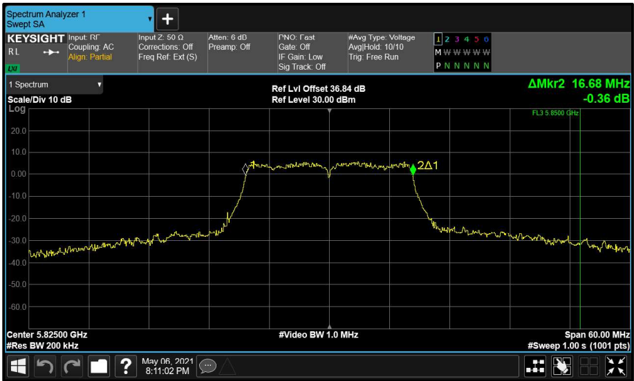
Figure 183 - Aux (B) 5825 MHz (CH165) 99% Bandwidth
