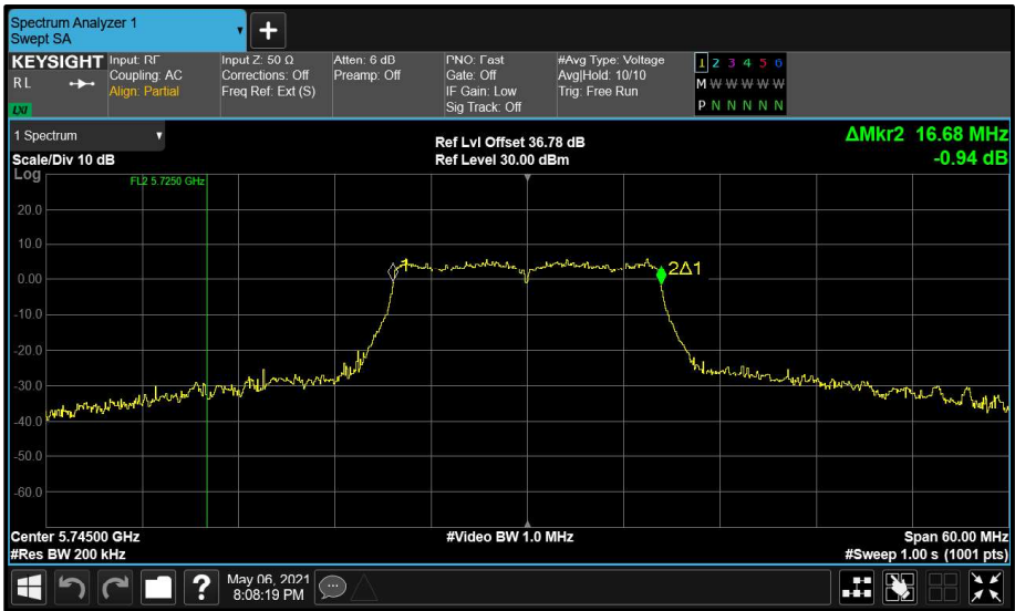
Figure 173 - Main (A) 5745 MHz (CH149) 99% Bandwidth
