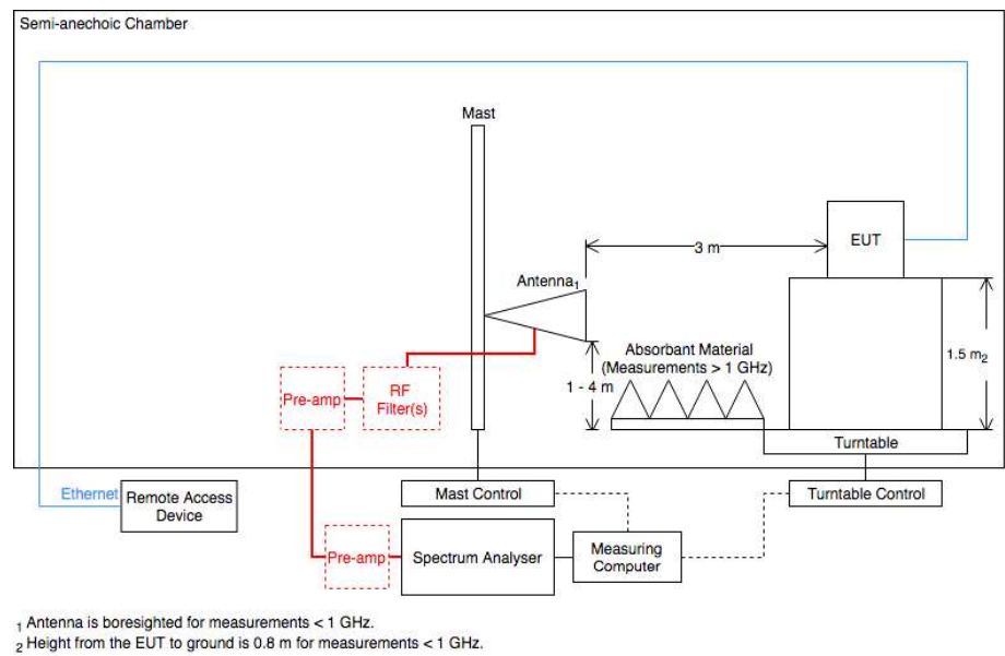
Figure 283 - Radiated Emissions Test Setup Diagram
