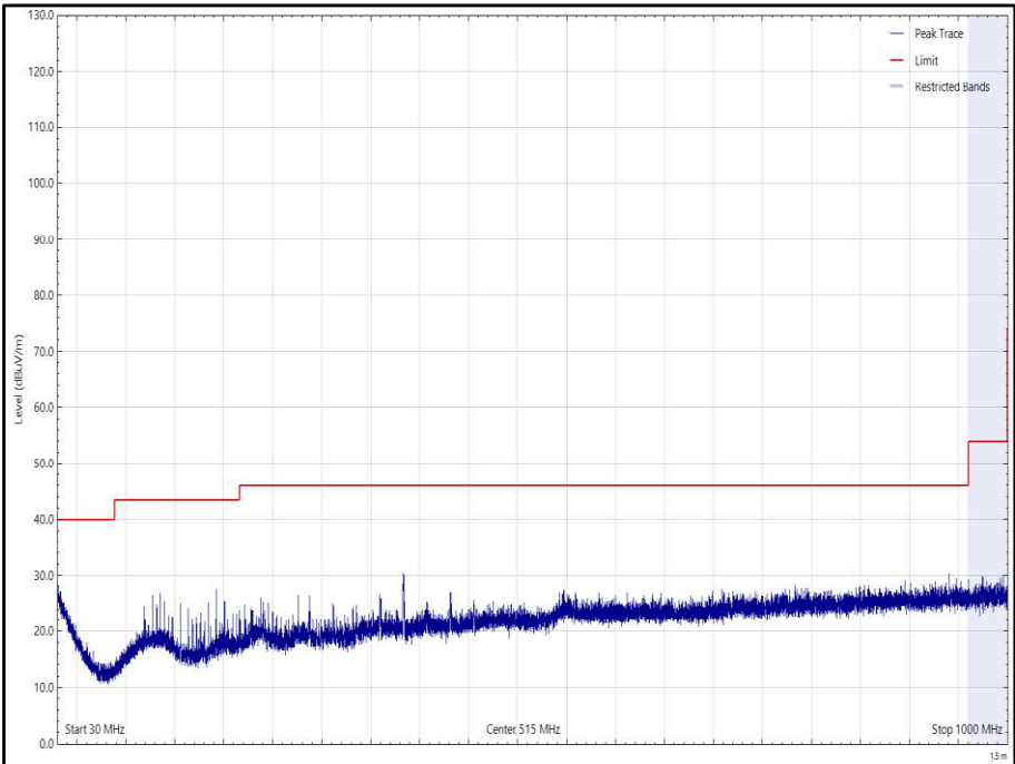
Figure 296 - 802.11a - 6 Mbps, 5240 MHz, 30 MHz to 1 GHz, Horizontal (Peak)
