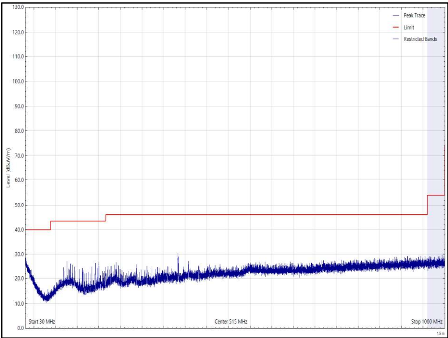
Figure 284 - 802.11a - 6 Mbps, 5180 MHz, 30 MHz to 1 GHz, Horizontal (Peak)
