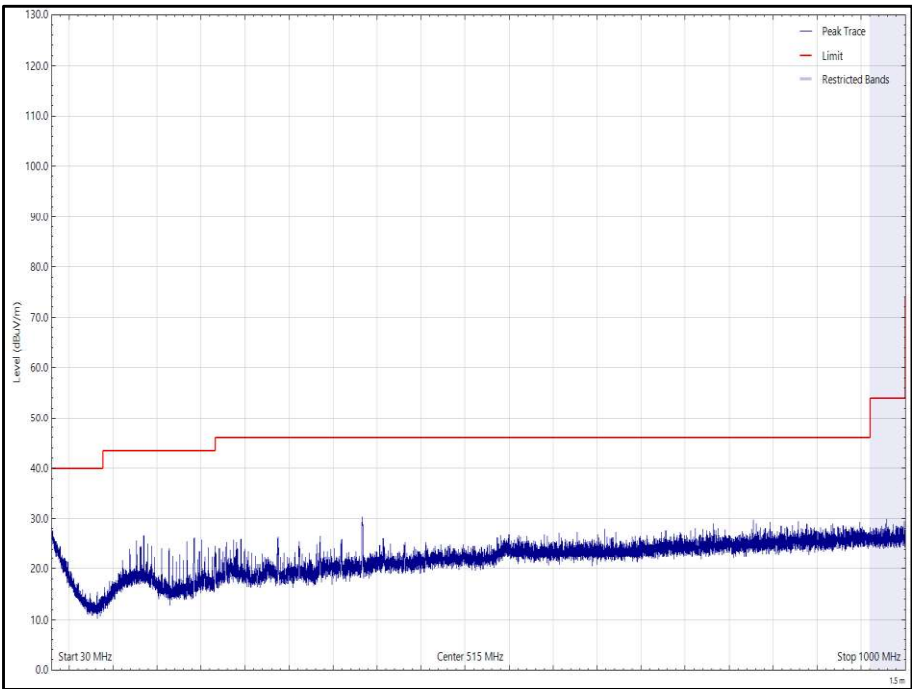
Figure 302 - 802.11a - 6 Mbps, 5260 MHz, 30 MHz to 1 GHz, Horizontal (Peak)
