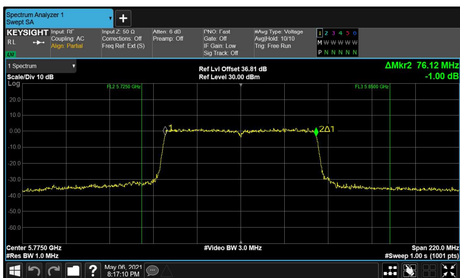
Figure 245 - Main (A) 5775 MHz (CH155) 99% Bandwidth
