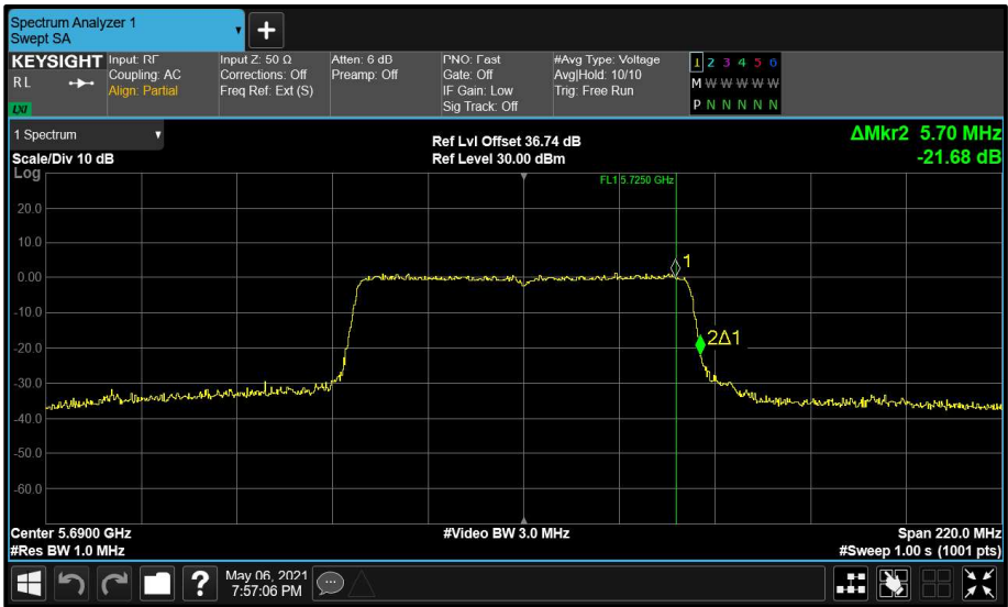
Figure 243 - Aux (B) 5690 MHz (CH138) 99% Bandwidth
