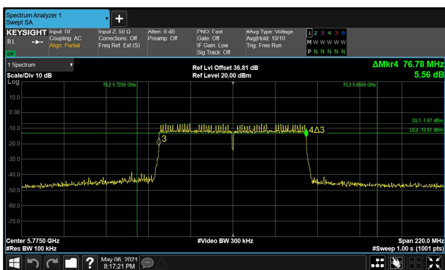
Figure 246 - Main (A) 5775 MHz (CH155) 6 dB Bandwidth
