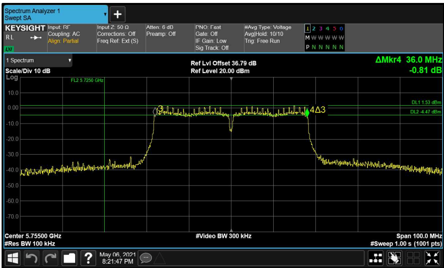
Figure 234 - Main (A) 5755 MHz (CH151) 6 dB Bandwidth
