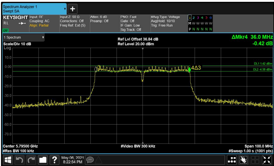
Figure 238 - Main (A) 5795 MHz (CH159) 6 dB Bandwidth
