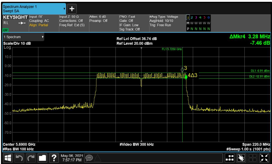
Figure 244 - Aux (B) 5690 MHz (CH138) 6 dB Bandwidth
