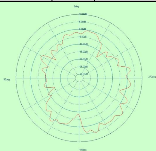
Free Space EIRP (5180MHz) – YZ cut
