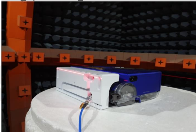
WIFI_A, with WIFI_B/BT terminated with 50ohms, dock
