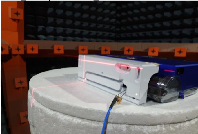
WIFI_B/BT, with WIFI_A terminated with 50ohms, dock
