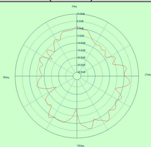
Free Space EIRP (5500MHz) – YZ cut
