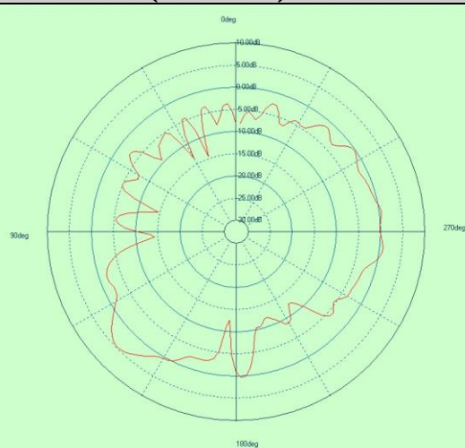
Free Space EIRP (5180MHz) – XY cut
