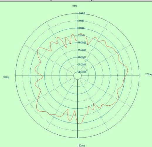
Free Space EIRP (5500MHz) – XY cut
