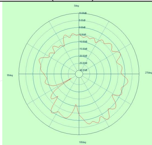
Free Space EIRP (5825MHz) - YZ cut
