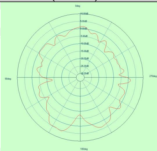
Free Space EIRP (5500MHz) – XZ cut
