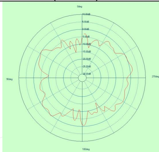
Free Space EIRP (5825MHz) - XY cut
