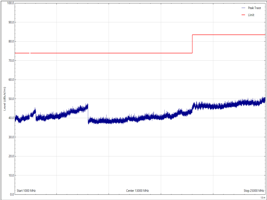
Figure 40 - 2440 MHz – 1 GHz to 25 GHz, Horizontal - Peak
