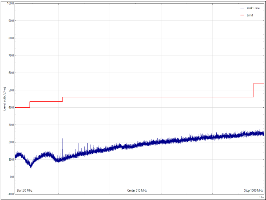
Figure 51 - 2402 MHz, 30 MHz to 1 GHz, Vertical
