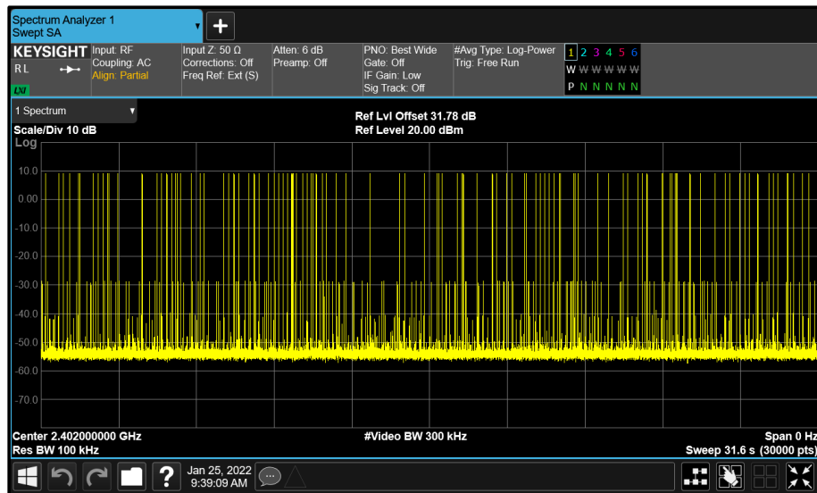
Figure 8 - GFSK - 2402 MHz Accumulated Transmit Time
