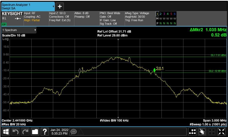
Figure 17 - R Cup (A) 2441 MHz (CH39) 20 dB Bandwidth
