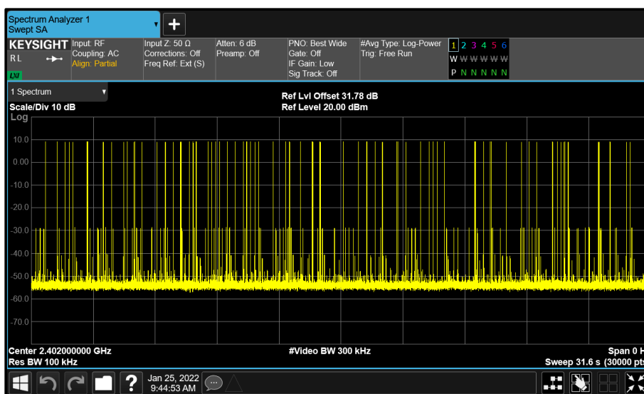
Figure 9 - GFSK - 2402 MHz Accumulated Transmit Time
