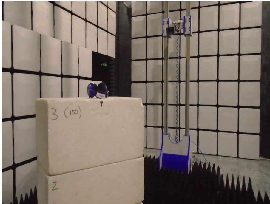
Figure 68 - Test Setup - 1 GHz to 18 GHz
