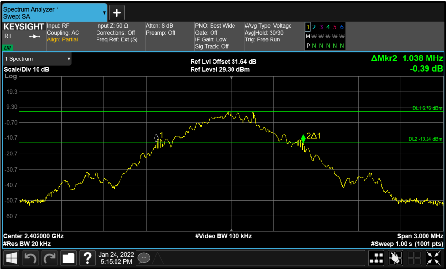
Figure 16 - R Cup (A) 2402 MHz (CH0) 20 dB Bandwidth
