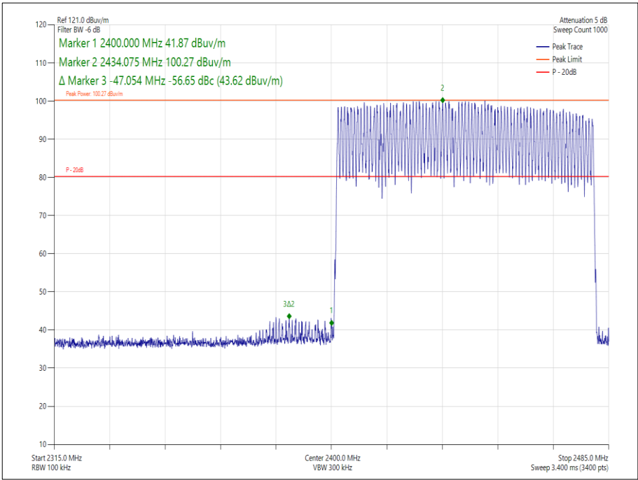
Figure 28 - Hopping - GFSK/DH5 - 2402 MHz - Measured Frequency 2400.0 MHz
