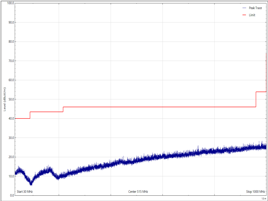
Figure 44 - 2480 MHz, 30 MHz to 1 GHz, Horizontal
