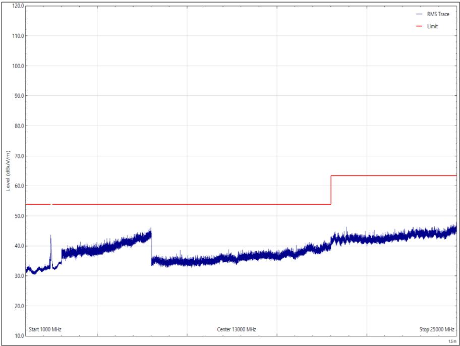
Figure 55 - 2402 MHz, 1 GHz to 25 GHz, Vertical - Average
