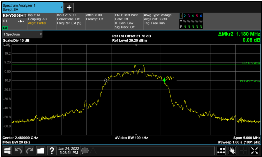
Figure 21 - R Cup (A) 2480 MHz (CH78) 20 dB Bandwidth
