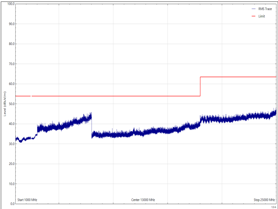
Figure 48 - 2480 MHz – 1 GHz to 25 GHz, Horizontal - Average
