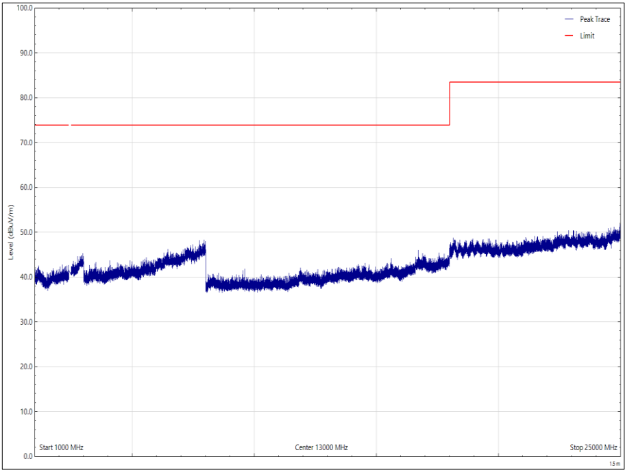
Figure 35 - 2402 MHz, 1 GHz to 25 GHz, Vertical - Peak
