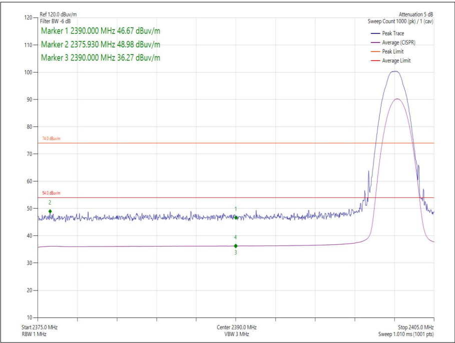
Figure 2 - \pi/4 DQPSK/2DH5 - 2402 MHz – Band Edge Frequency 2390.0 MHz
