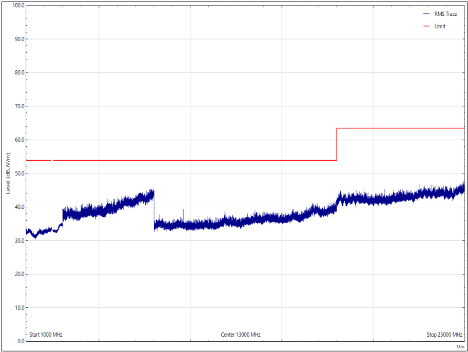
Figure 36 - 2402 MHz, 1 GHz to 25 GHz, Horizontal - Average
