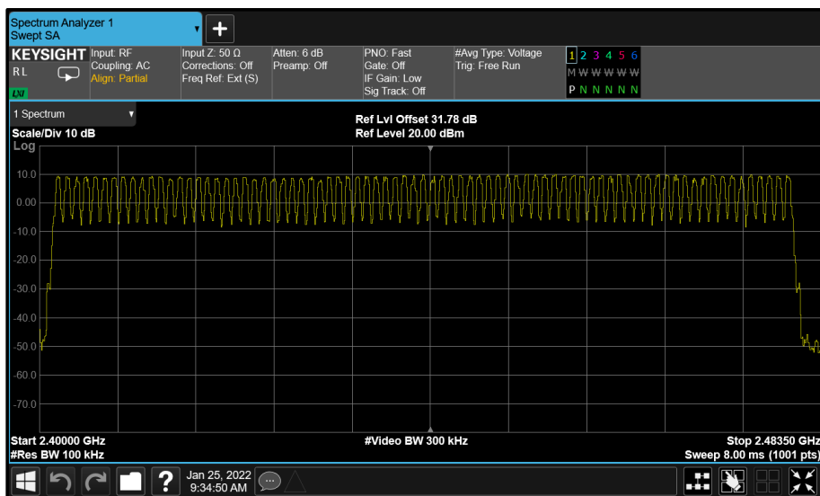
Figure 13 - GFSK (DH1) - Number of Hopping Channels
