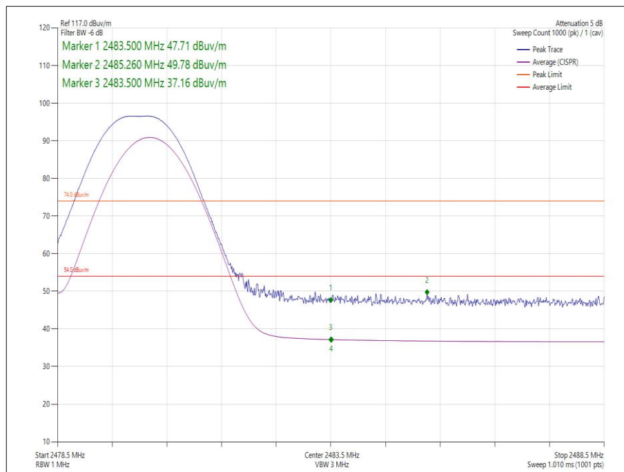
Figure 4 - GFSK/DH5 - 2480 MHz – Band Edge Frequency 2483.5 MHz
