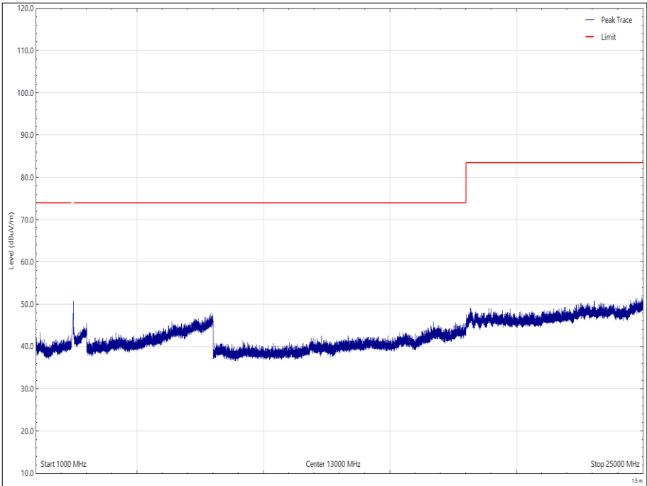
Figure 65 - 2480 MHz - 1 GHz to 25 GHz, Vertical - Peak
