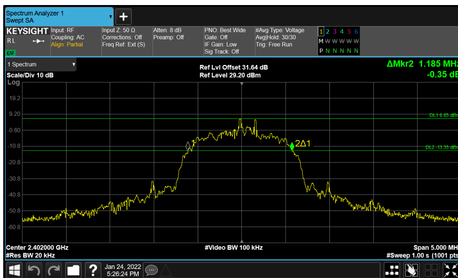
Figure 19 - R Cup (A) 2402 MHz (CH0) 20 dB Bandwidth
