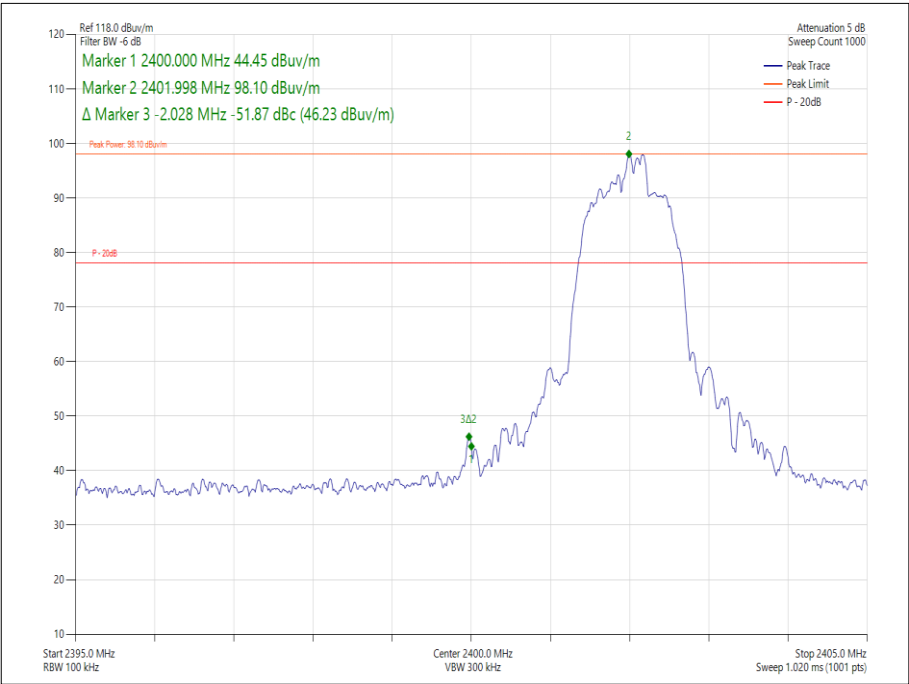
Figure 27 - Static - 8-DPSK/3DH5 - 2402 MHz - Measured Frequency 2400.0 MHz
