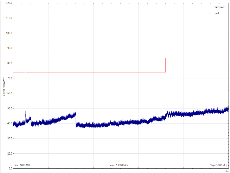
Figure 53 - 2402 MHz, 1 GHz to 25 GHz, Vertical - Peak
