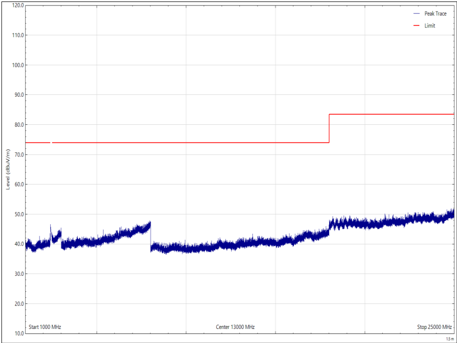
Figure 52 - 2402 MHz, 1 GHz to 25 GHz, Horizontal - Peak
