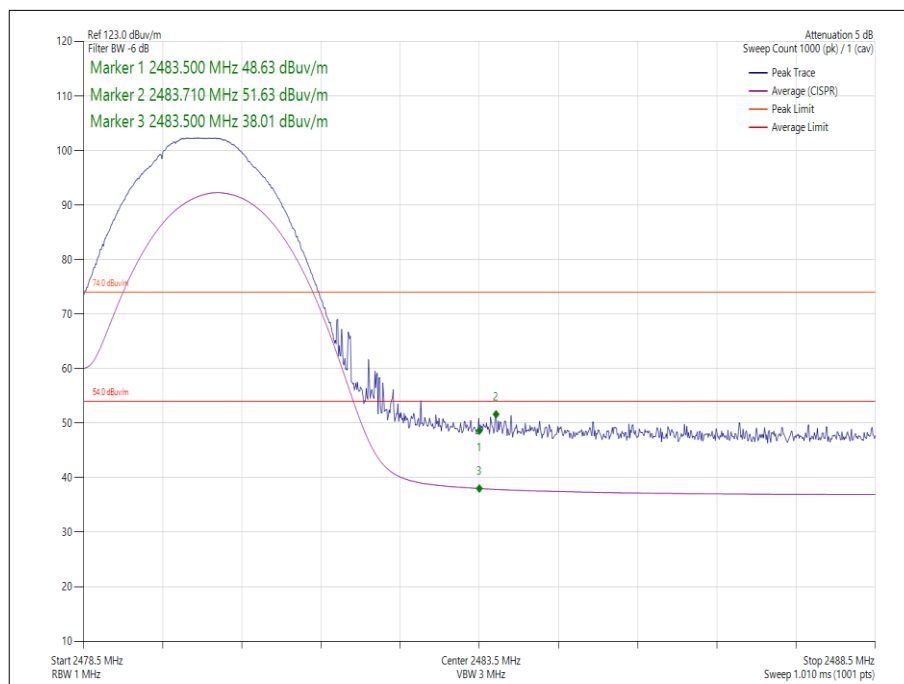
Figure 5 - \pi/4 DQPSK/2DH5 - 2480 MHz – Band Edge Frequency 2483.5 MHz
