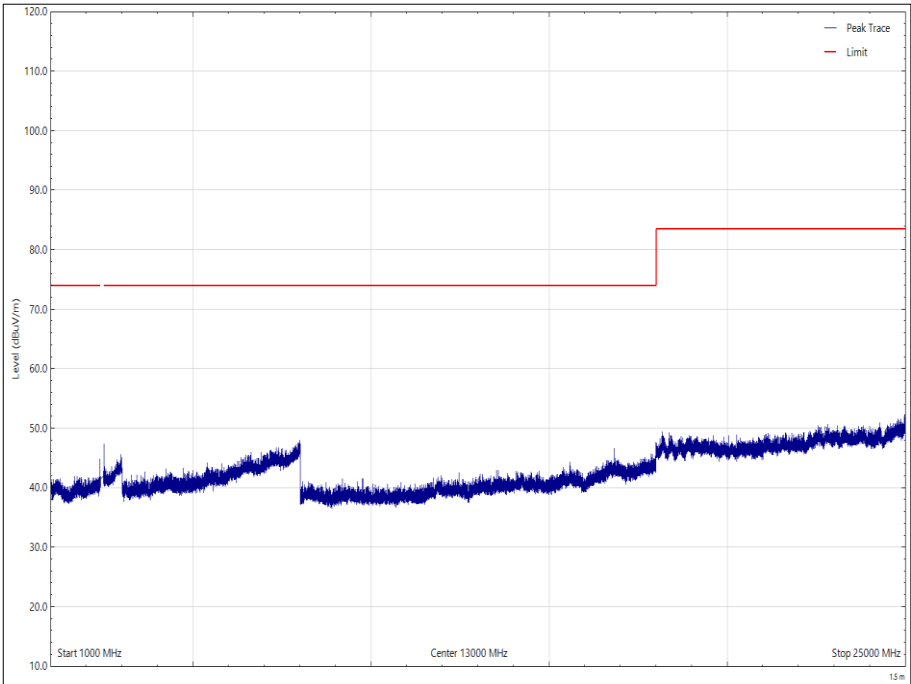
Figure 59 - 2440 MHz - 1 GHz to 25 GHz, Vertical - Peak
