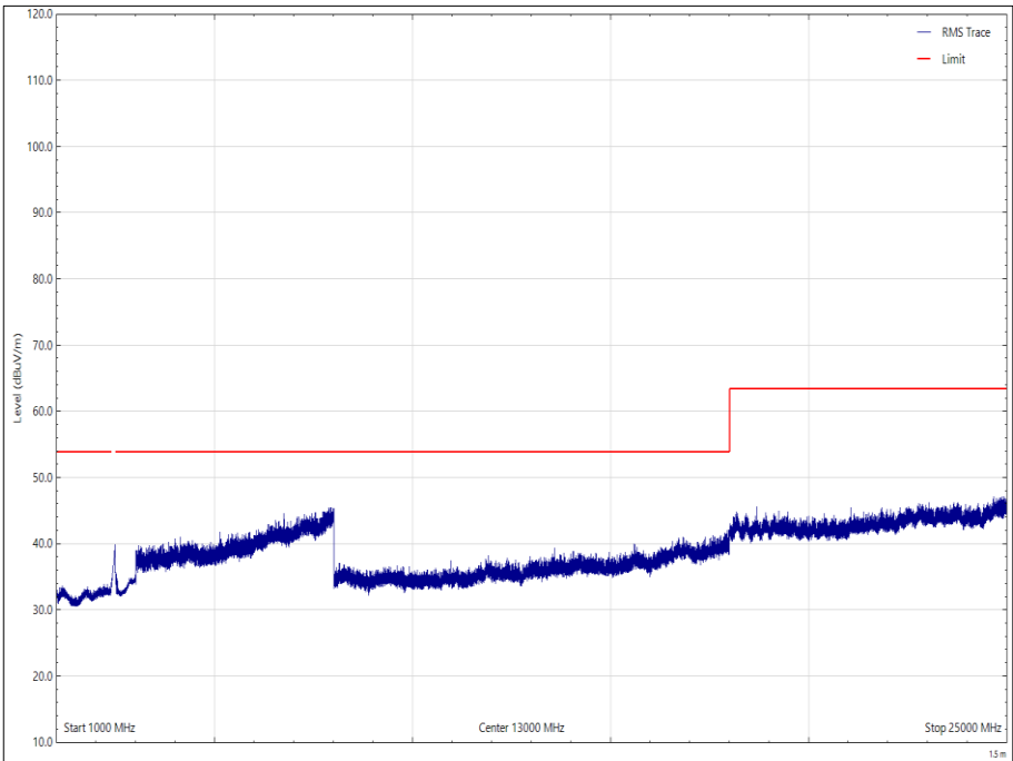
Figure 66 - 2480 MHz - 1 GHz to 25 GHz, Horizontal - Average
