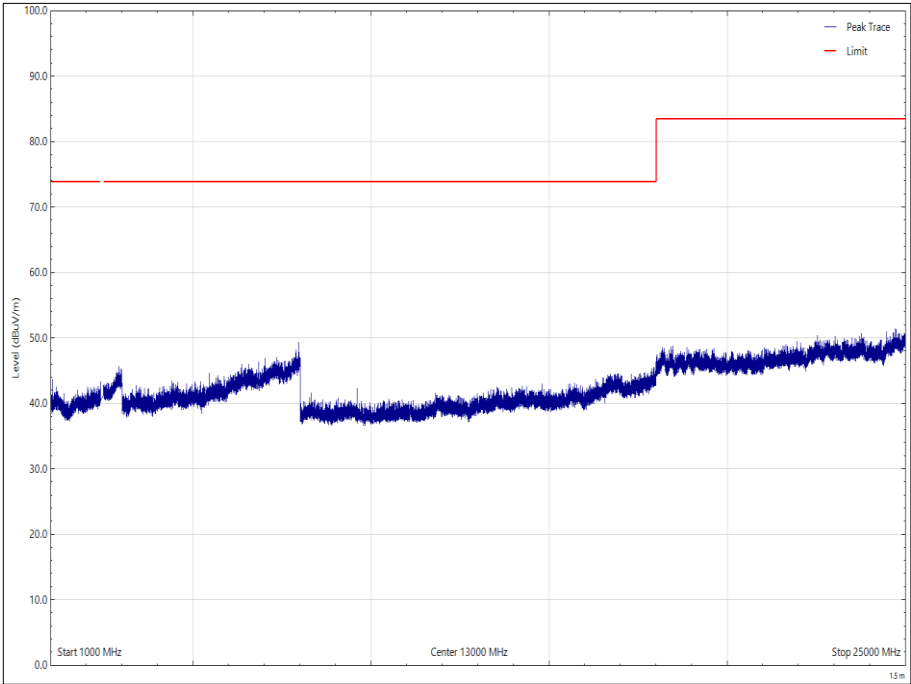
Figure 34 - 2402 MHz, 1 GHz to 25 GHz, Horizontal - Peak
