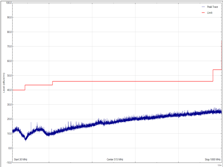
Figure 57 - 2440 MHz, 30 MHz to 1 GHz, Vertical
