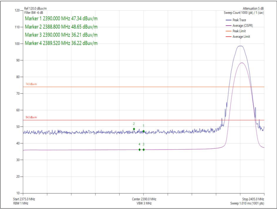
Figure 3 - 8-DPSK/3DH5 - 2402 MHz – Band Edge Frequency 2390.0 MHz
