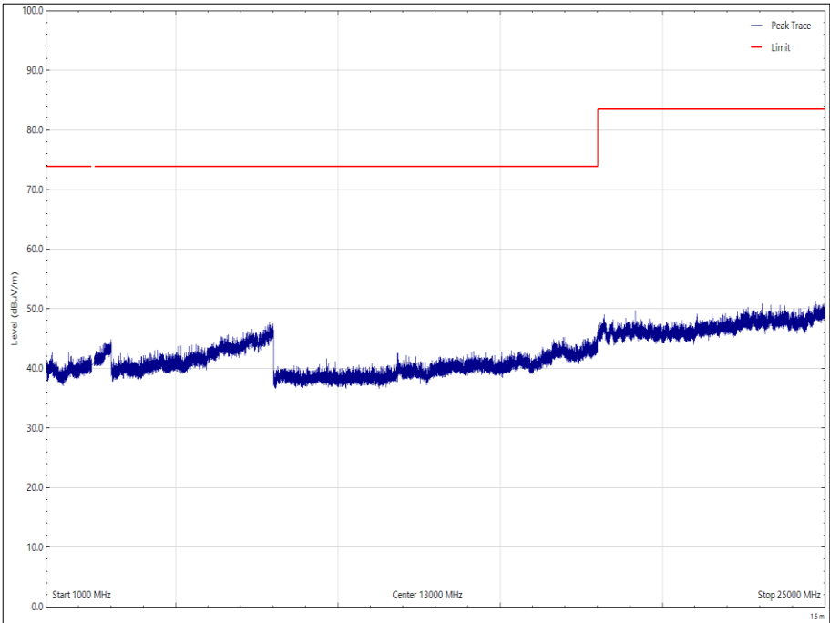
Figure 47 - 2480 MHz – 1 GHz to 25 GHz, Vertical - Peak
