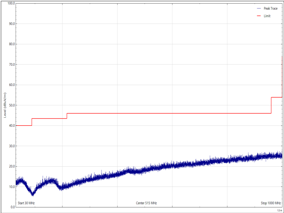
Figure 38 - 2440 MHz, 30 MHz to 1 GHz, Horizontal
