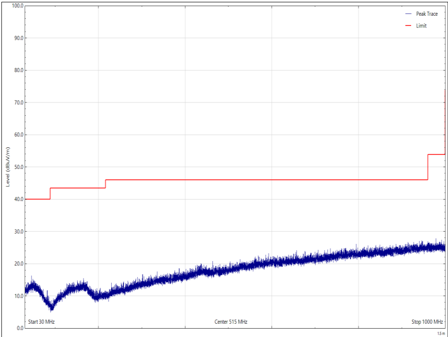
Figure 39 - 2440 MHz, 30 MHz to 1 GHz, Vertical
