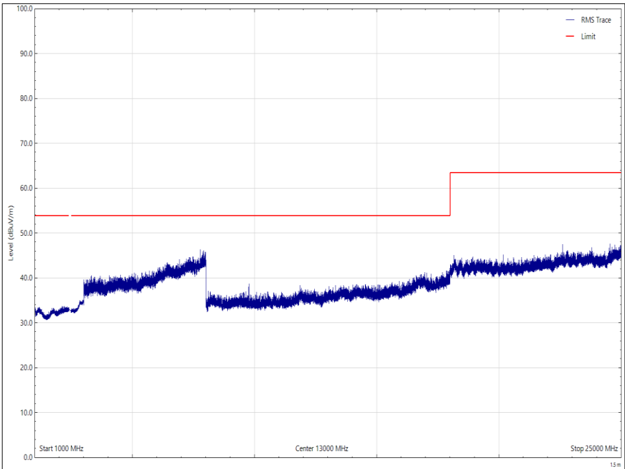
Figure 42 - 2440 MHz – 1 GHz to 25 GHz, Horizontal - Average
