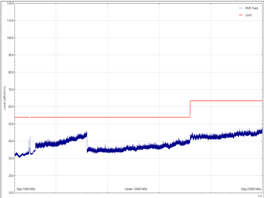
Figure 61 - 2440 MHz - 1 GHz to 25 GHz, Vertical - Average
