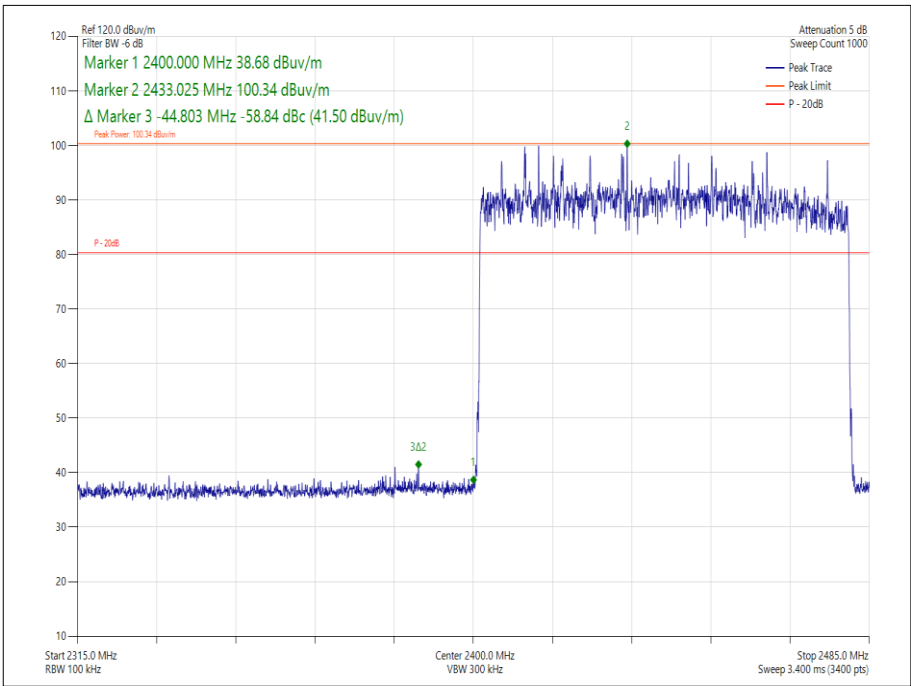
Figure 29 - Hopping - \pi/4 DQPSK/2DH5 - 2402 MHz - Measured Frequency 2400.0 MHz
