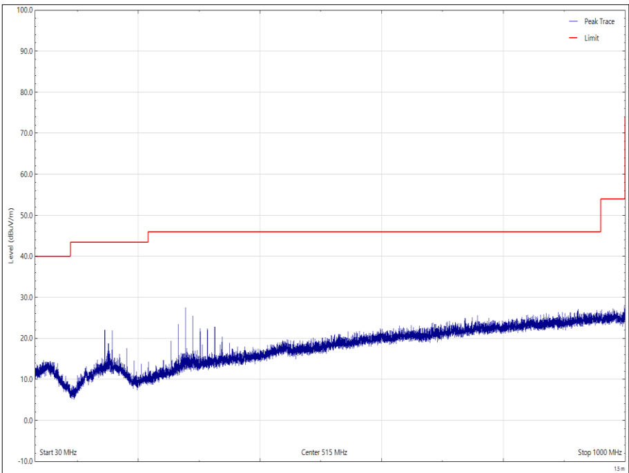
Figure 50 - 2402 MHz, 30 MHz to 1 GHz, Horizontal
