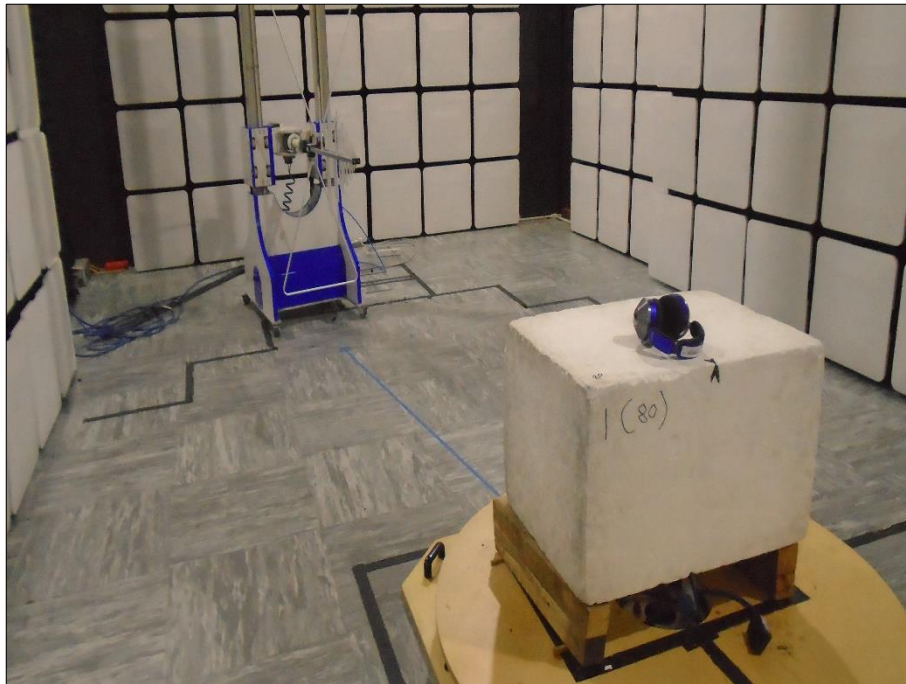
Figure 70 - Test Setup - 30 MHz to 1 GHz
