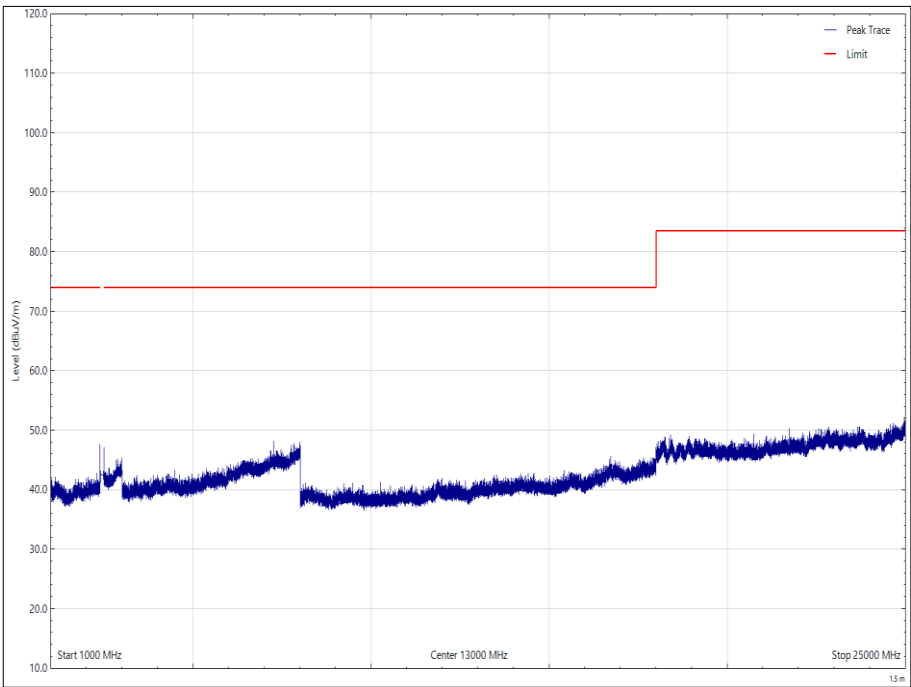
Figure 58 - 2440 MHz - 1 GHz to 25 GHz, Horizontal - Peak
