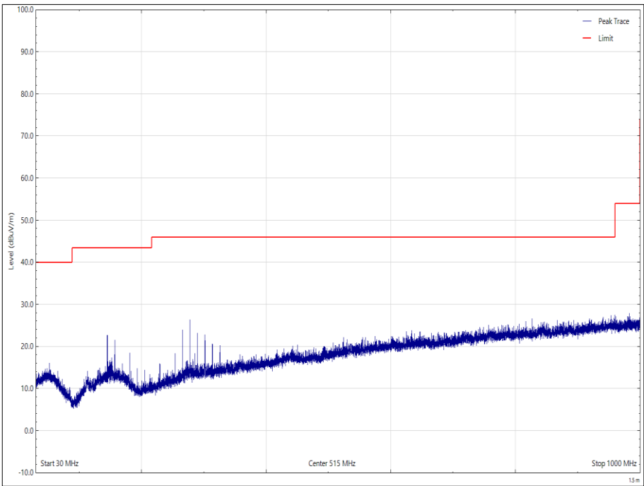
Figure 62 - 2480 MHz, 30 MHz to 1 GHz, Horizontal
