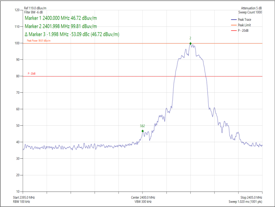
Figure 26 - Static - \pi/4 DQPSK/2DH5 - 2402 MHz - Measured Frequency 2400.0 MHz
