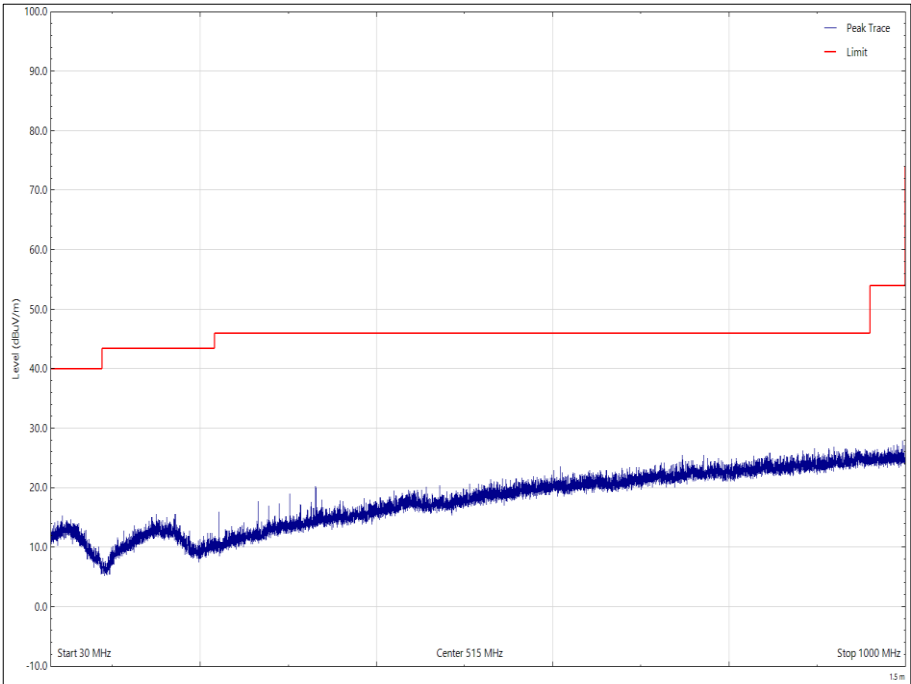
Figure 63 - 2480 MHz, 30 MHz to 1 GHz, Vertical
