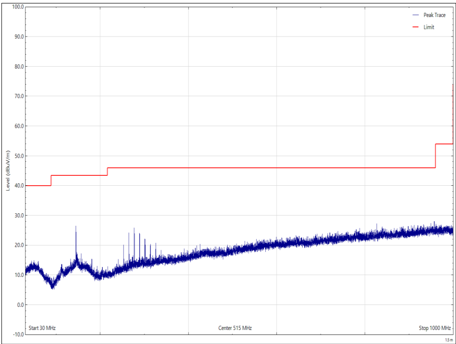
Figure 56 - 2440 MHz, 30 MHz to 1 GHz, Horizontal
