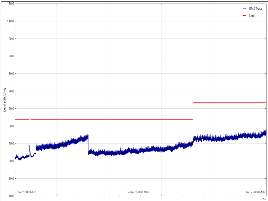
Figure 54 - 2402 MHz, 1 GHz to 25 GHz, Horizontal - Average
