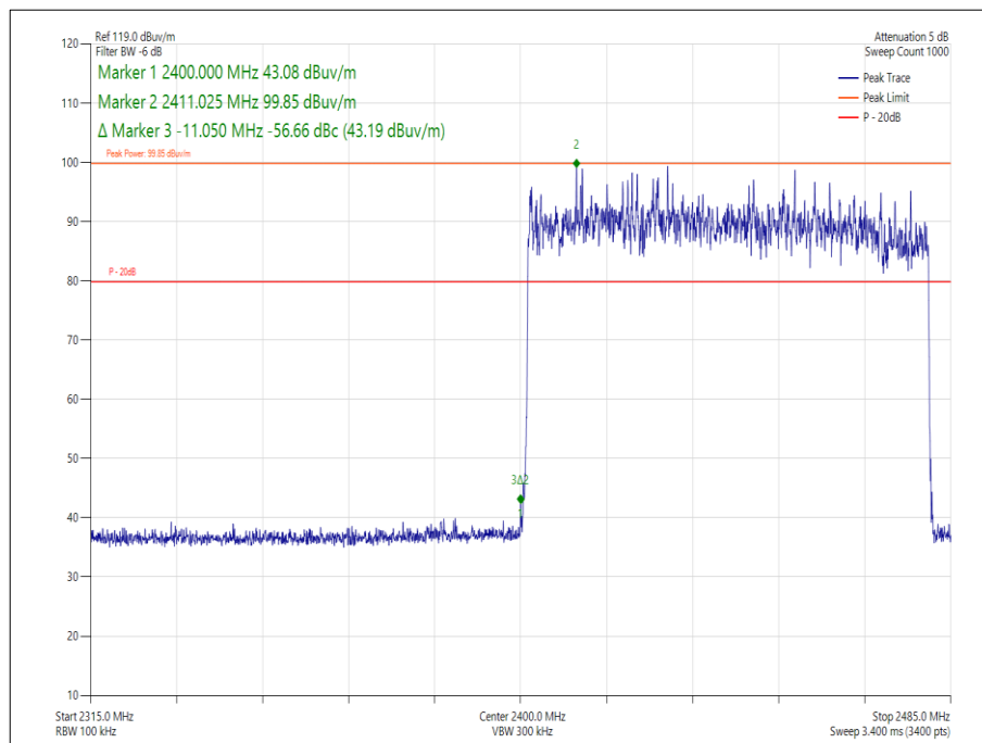
Figure 30 - Hopping - 8-DPSK/3DH5 - 2402 MHz - Measured Frequency 2400.0 MHz
