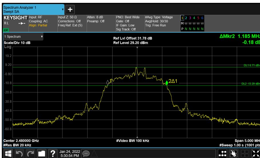
Figure 24 - R Cup (A) 2480 MHz (CH78) 20 dB Bandwidth
