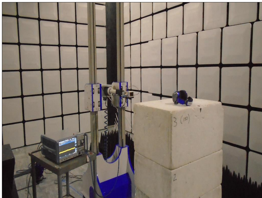
Figure 69 - Test Setup - 18 GHz to 25 GHz
