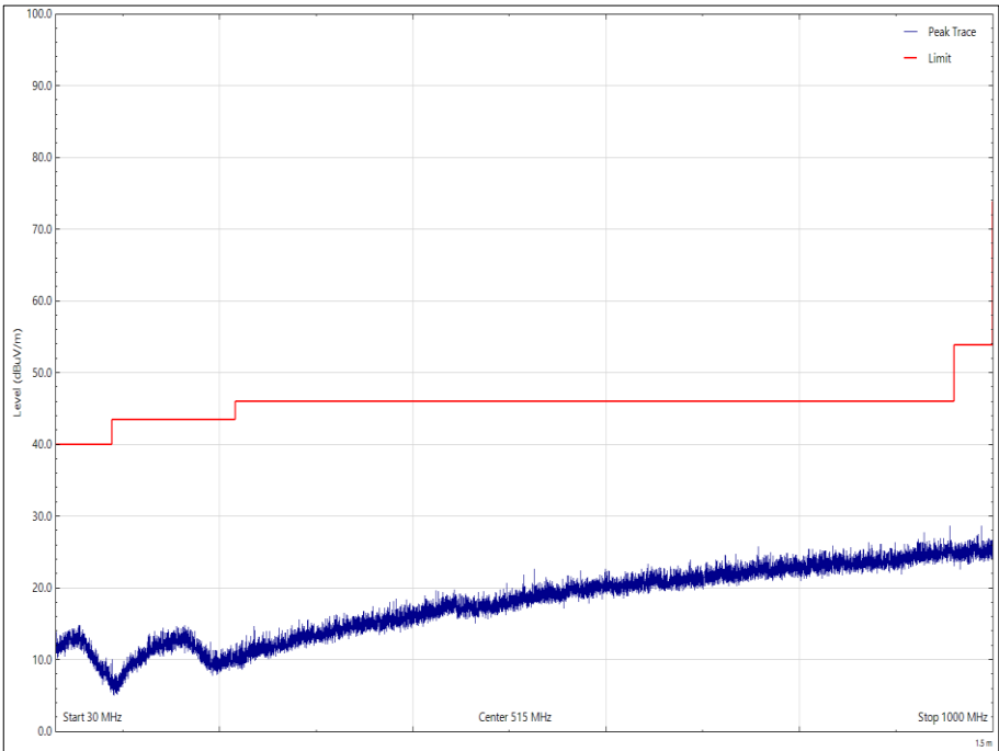
Figure 32 - 2402 MHz, 30 MHz to 1 GHz, Horizontal
