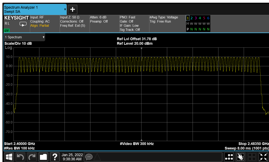
Figure 14 - GFSK (DH3) - Number of Hopping Channels
