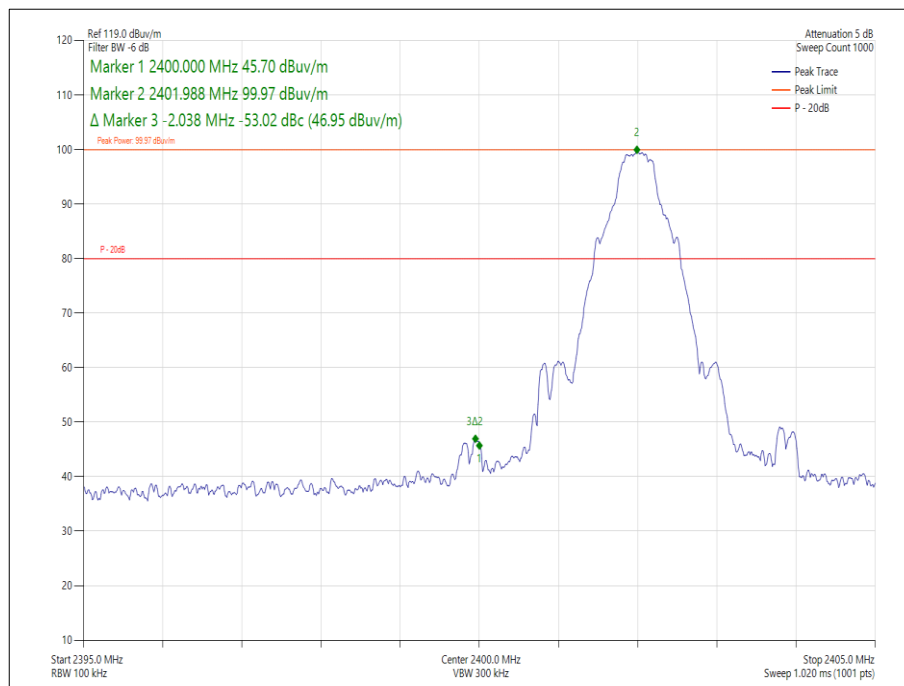
Figure 25 - Static - GFSK/DH5 - 2402 MHz - Measured Frequency 2400.0 MHz
