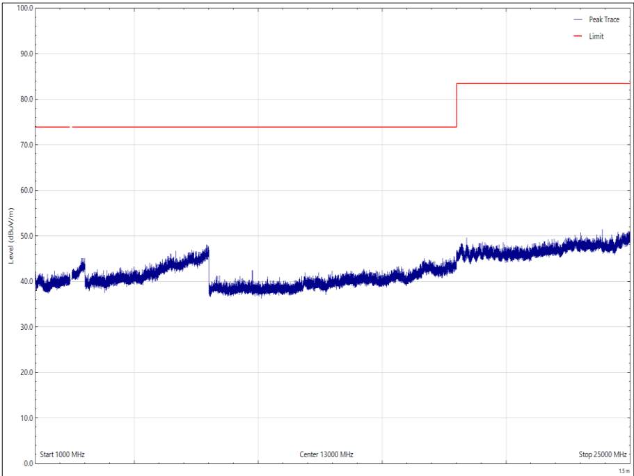
Figure 41 - 2440 MHz – 1 GHz to 25 GHz, Vertical - Peak
