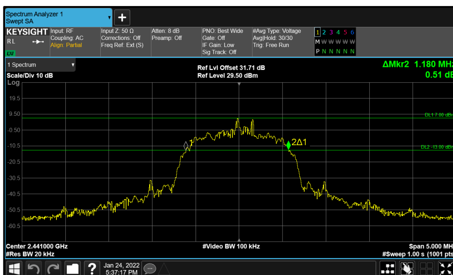
Figure 20 - R Cup (A) 2441 MHz (CH39) 20 dB Bandwidth
