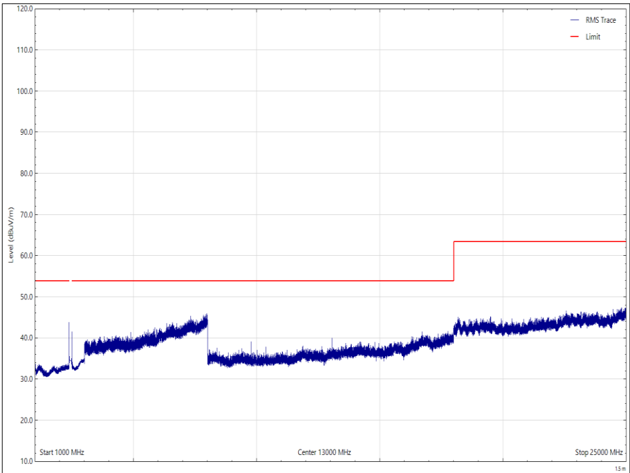
Figure 60 - 2440 MHz - 1 GHz to 25 GHz, Horizontal - Average
