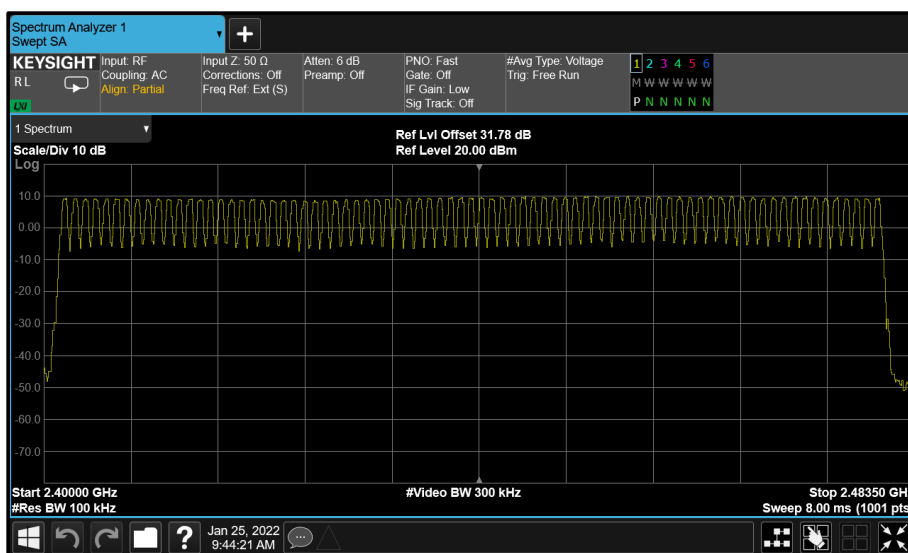
Figure 15 - GFSK (DH5) - Number of Hopping Channels
