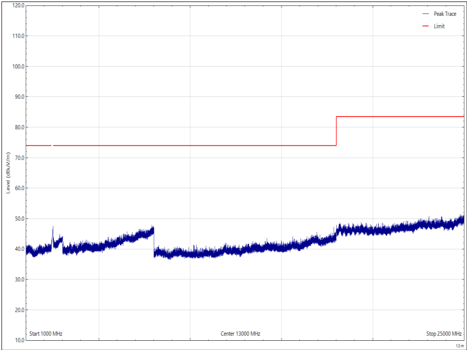
Figure 64 - 2480 MHz - 1 GHz to 25 GHz, Horizontal – Peak
