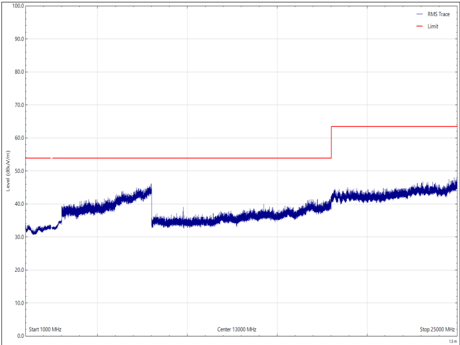
Figure 43 - 2440 MHz – 1 GHz to 25 GHz, Vertical - Average
