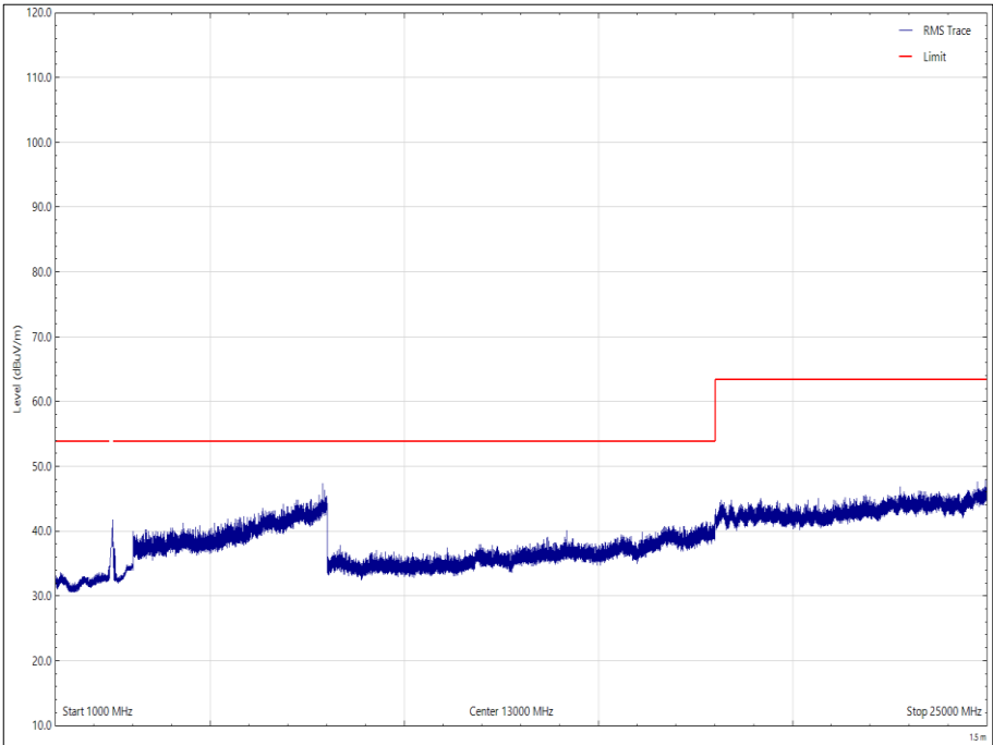
Figure 67 - 2480 MHz - 1 GHz to 25 GHz, Vertical - Average
