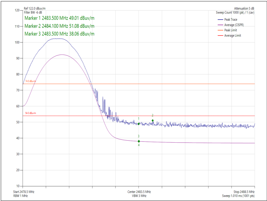
Figure 6 - 8-DPSK/3DH5 - 2480 MHz – Band Edge Frequency 2483.5 MHz
