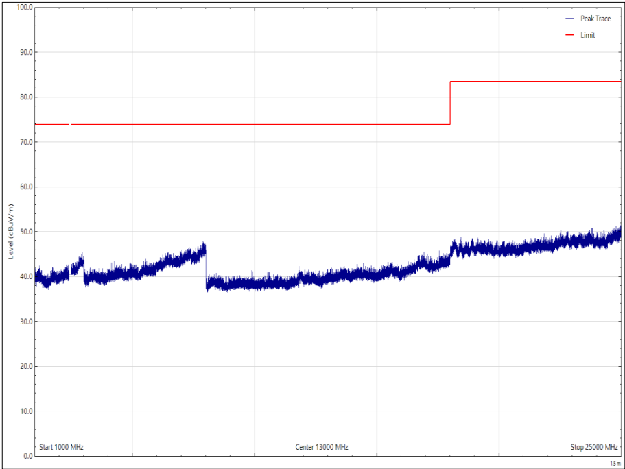
Figure 46 - 2480 MHz – 1 GHz to 25 GHz, Horizontal - Peak
