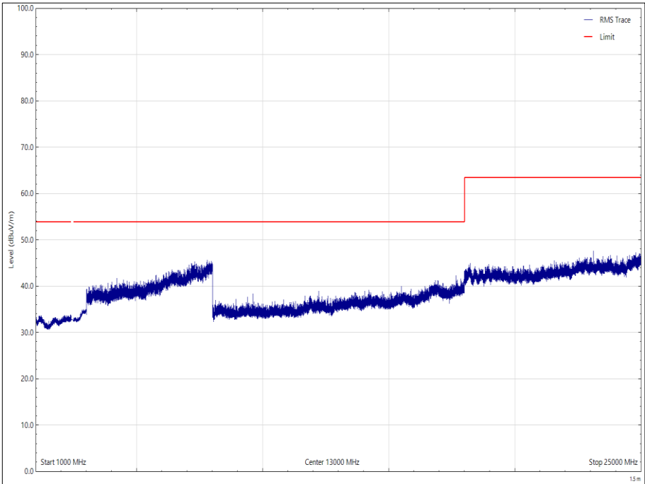
Figure 37 - 2402 MHz, 1 GHz to 25 GHz, Vertical - Average
