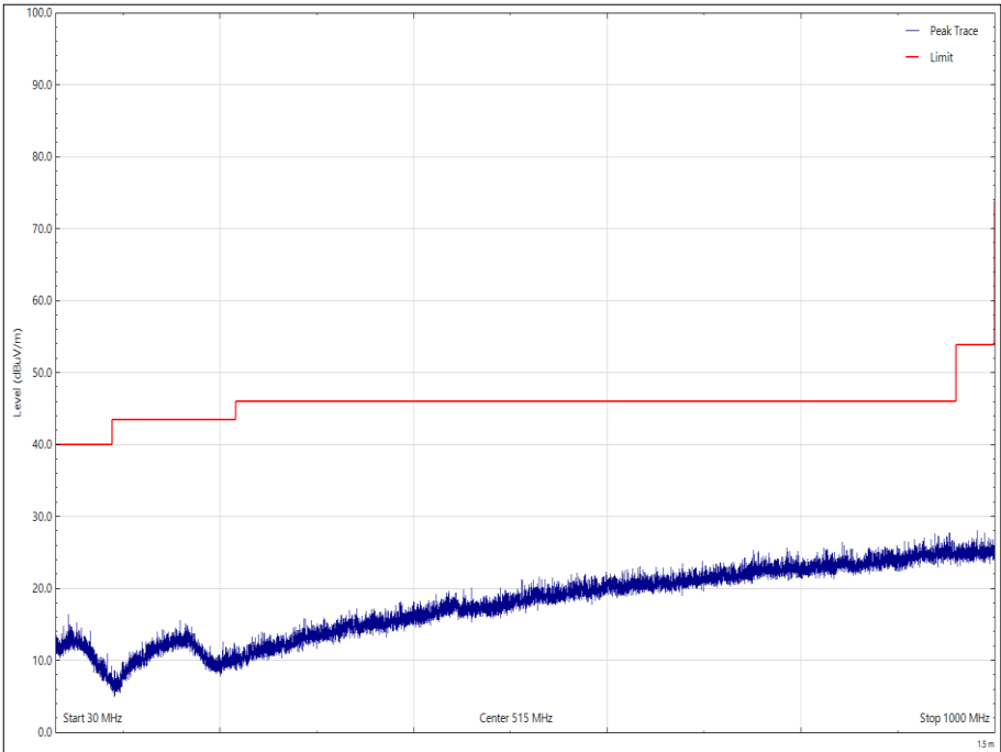
Figure 45 - 2480 MHz, 30 MHz to 1 GHz, Vertical
