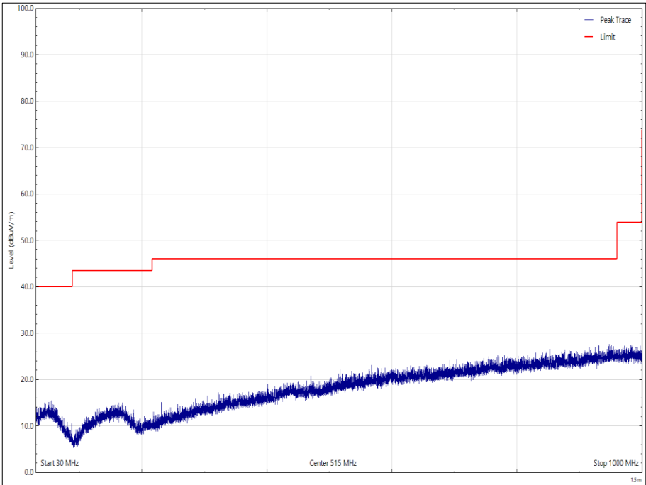
Figure 33 - 2402 MHz, 30 MHz to 1 GHz, Vertical
