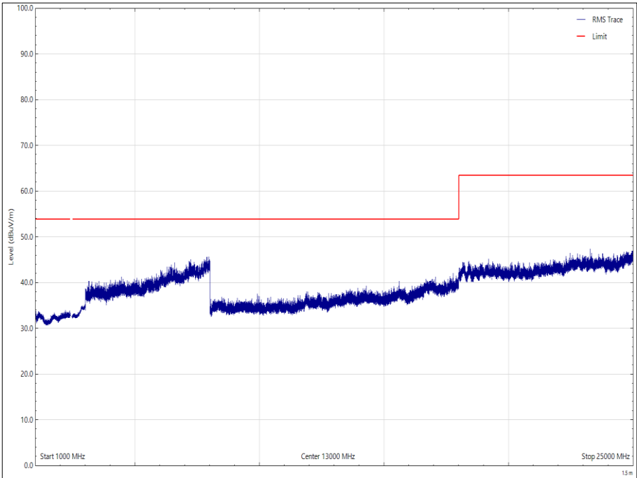
Figure 49 - 2480 MHz – 1 GHz to 25 GHz, Vertical - Average
