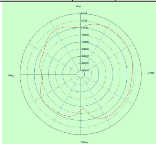
Free Space GAIN TOTAL (2440MHz) - XY cut
