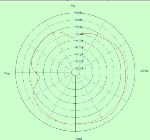
Free Space GAIN TOTAL (2402MHz) – XY cut
