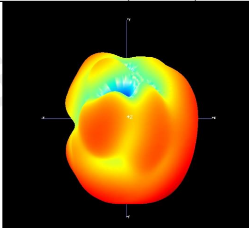
Free Space GAIN TOTAL (2402MHz) - 3D
