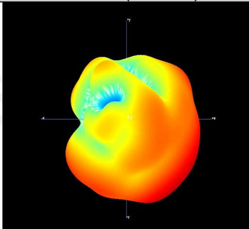
Free Space GAIN TOTAL (2480MHz) - 3D
