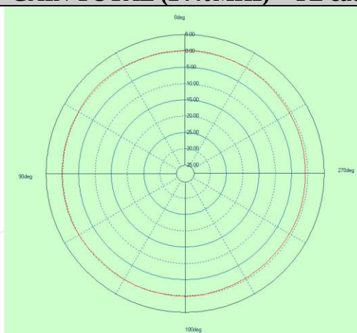
Free Space GAIN TOTAL (2440MHz) - YZ cut
