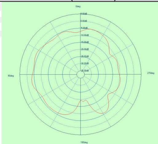
Free Space GAIN TOTAL (2402MHz) - XZ cut
