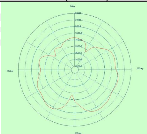
Free Space GAIN TOTAL (2440MHz) - XZ cut
