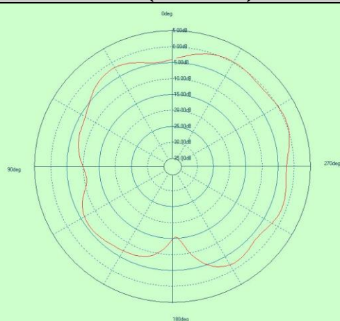
Free Space GAIN TOTAL (2480MHz) - XY cut
