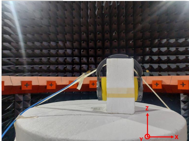
Test Setup Left Antenna
