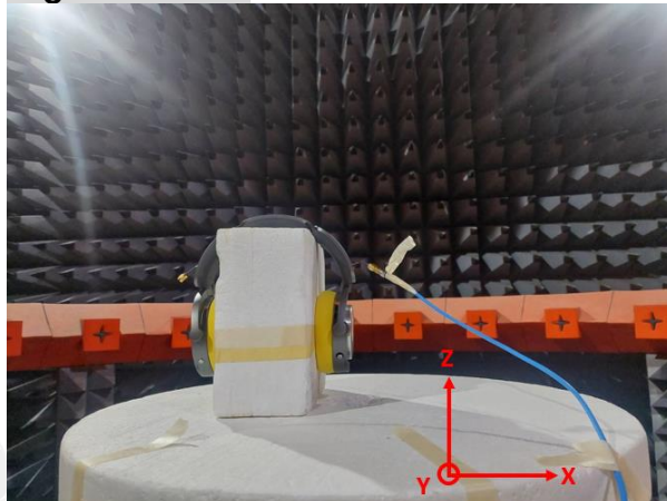
Right Antenna
