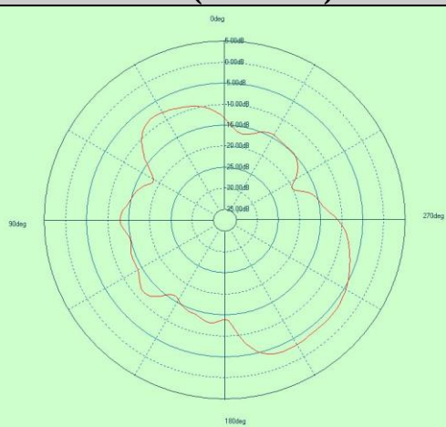
Free Space GAIN TOTAL (2440MHz) - YZ cut
