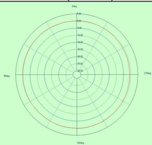
Free Space GAIN TOTAL (2402MHz) - YZ cut
