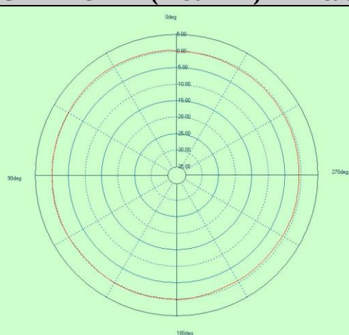
Free Space GAIN TOTAL (2480MHz) - YZ cut
