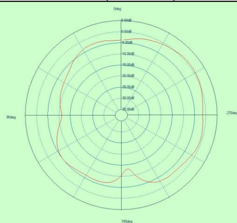
Free Space GAIN TOTAL (2402MHz) - XY cut
