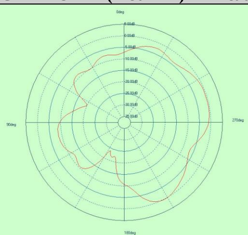
Free Space GAIN TOTAL (2480MHz) - YZ cut
