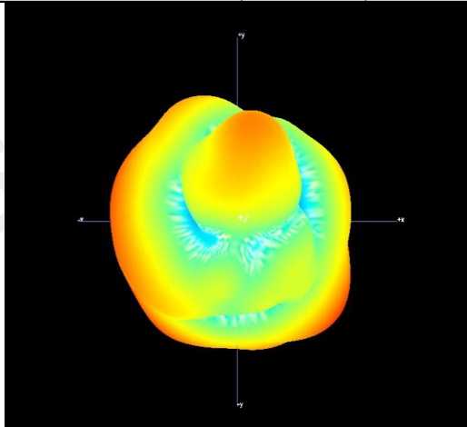
Free Space GAIN TOTAL (2440MHz) - 3D
