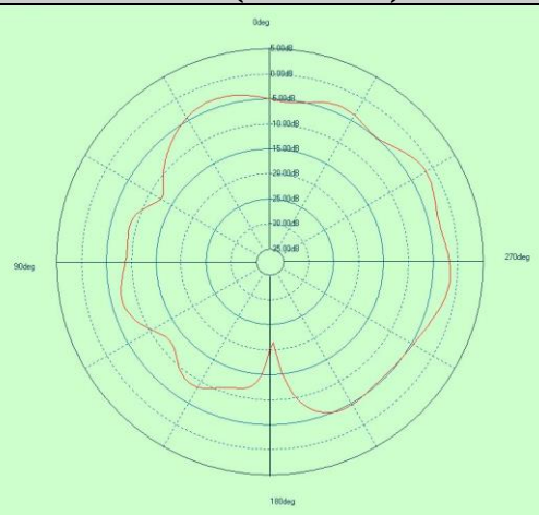
Free Space GAIN TOTAL (2402MHz) – YZ cut
