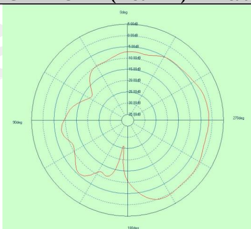
Free Space GAIN TOTAL (2480MHz) - XZ cut
