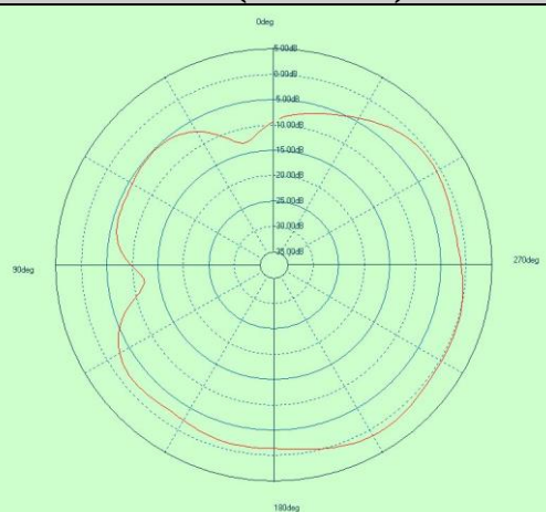
Free Space GAIN TOTAL (2480MHz) - XY cut
