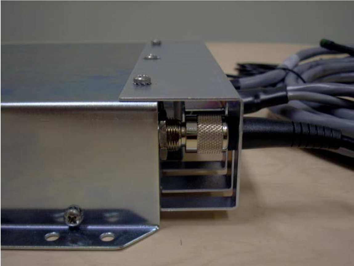
Photograph 4 - 9: Side view of the Fleetlink M1 OBC without Terminal.
