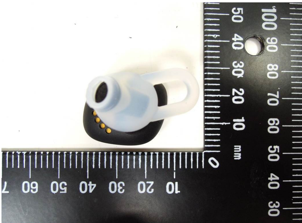
Front View of EUT (Right)
