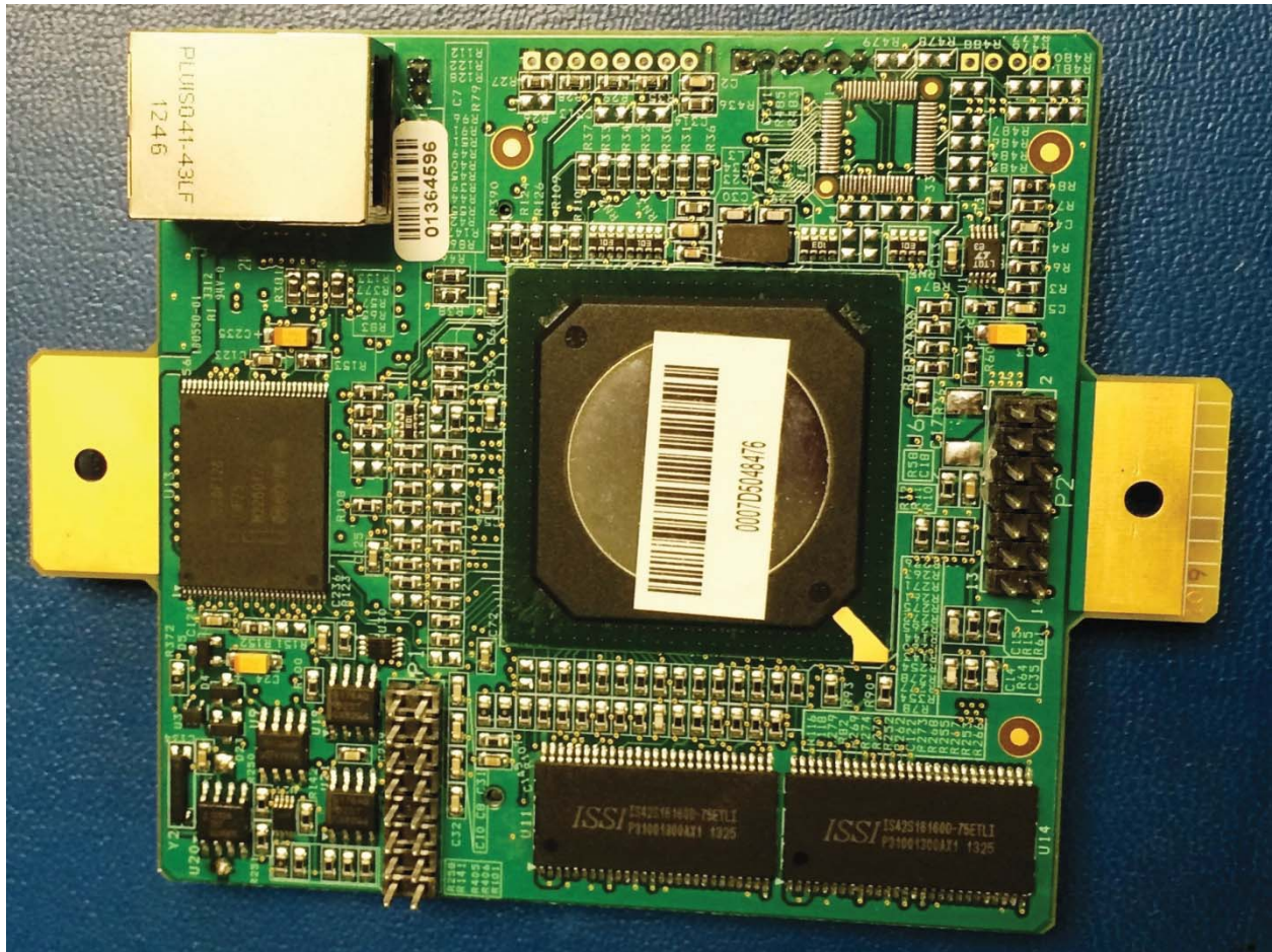
3e-523-3 Main Board Bottom View
