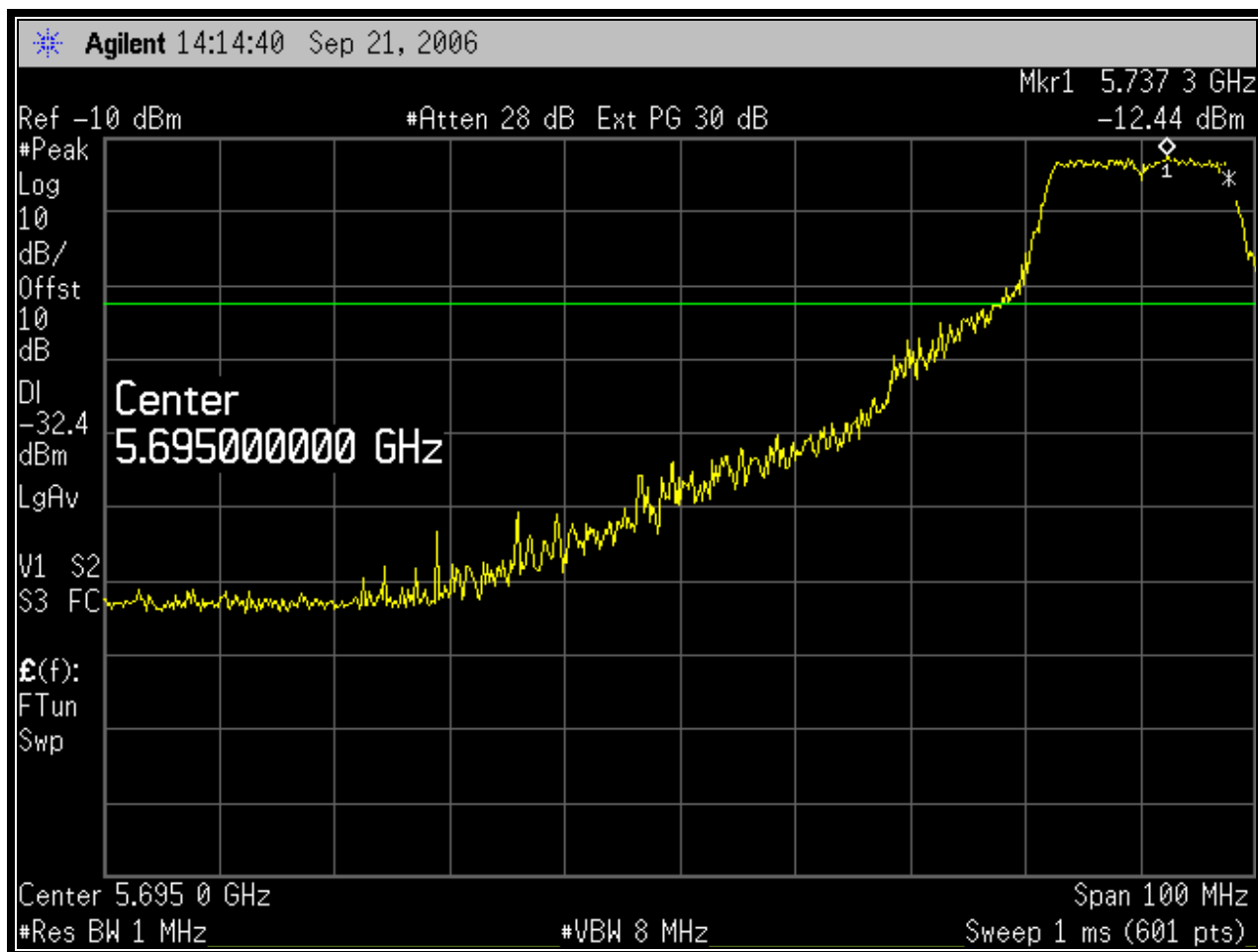
Plot 4-5: Lower Band Edge: Channel 149 (TX Frequency: 5745 MHz – 54 Mbs)
