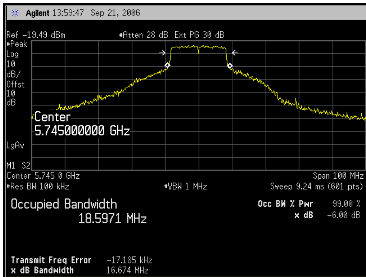
Plot 6-7: 6 dB Bandwidth Channel 149 (TX Frequency: 5745 MHz – 54 Mbps) 802.11a
