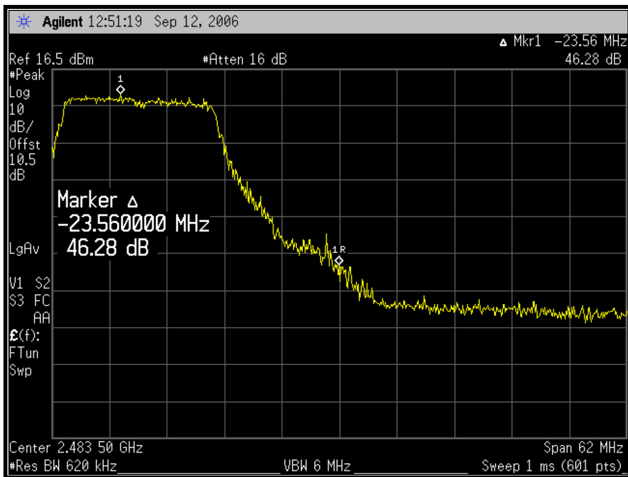
Plot 4-4: Upper Band Edge: Delta Measurement Channel 11 (TX Frequency: 2462 MHz – 54 Mbps)
