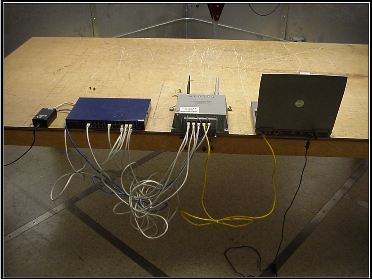
Photograph 5: Conducted Testing Back View
