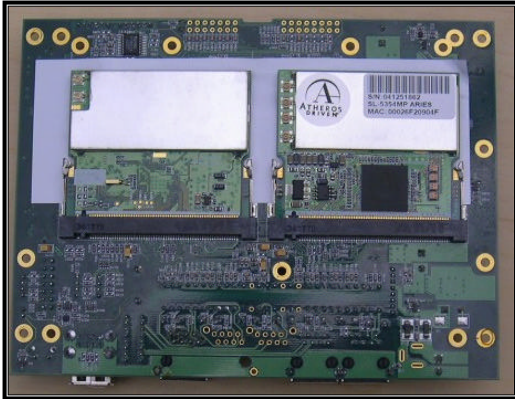
PHOTOGRAPH 11: XS 3 PT BOTTOM ASSEMBLY
