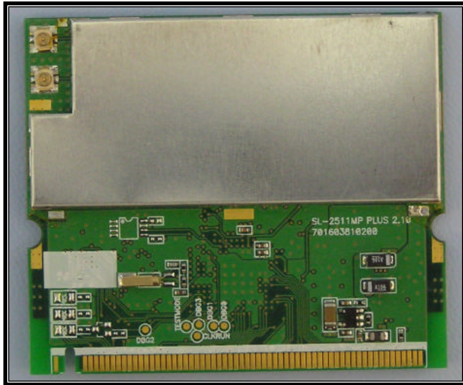
PHOTOGRAPH 13: 2511MP 11B TOP VIEW
