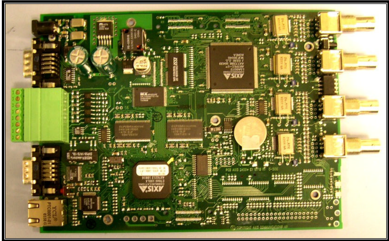
PHOTOGRAPH 16: VIDEO TOP VIEW
