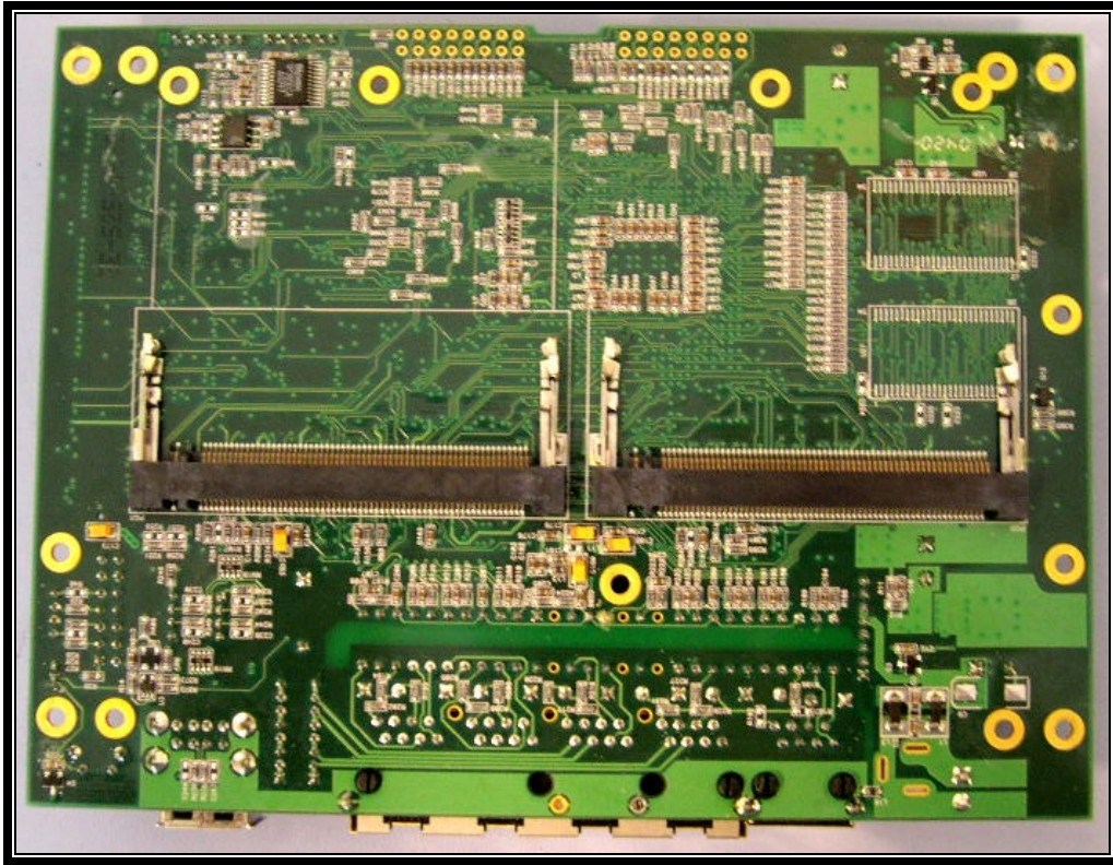
PHOTOGRAPH 9: XS 5 PT BOTTOM VIEW
