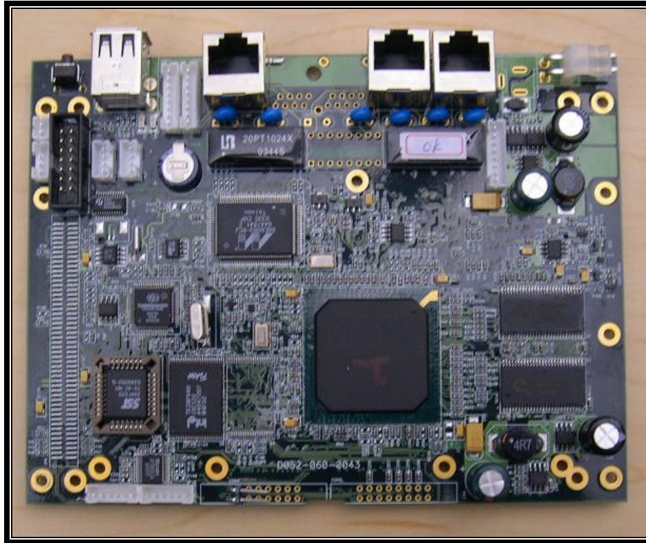
PHOTOGRAPH 10: XS 3 PT TOP VIEW
