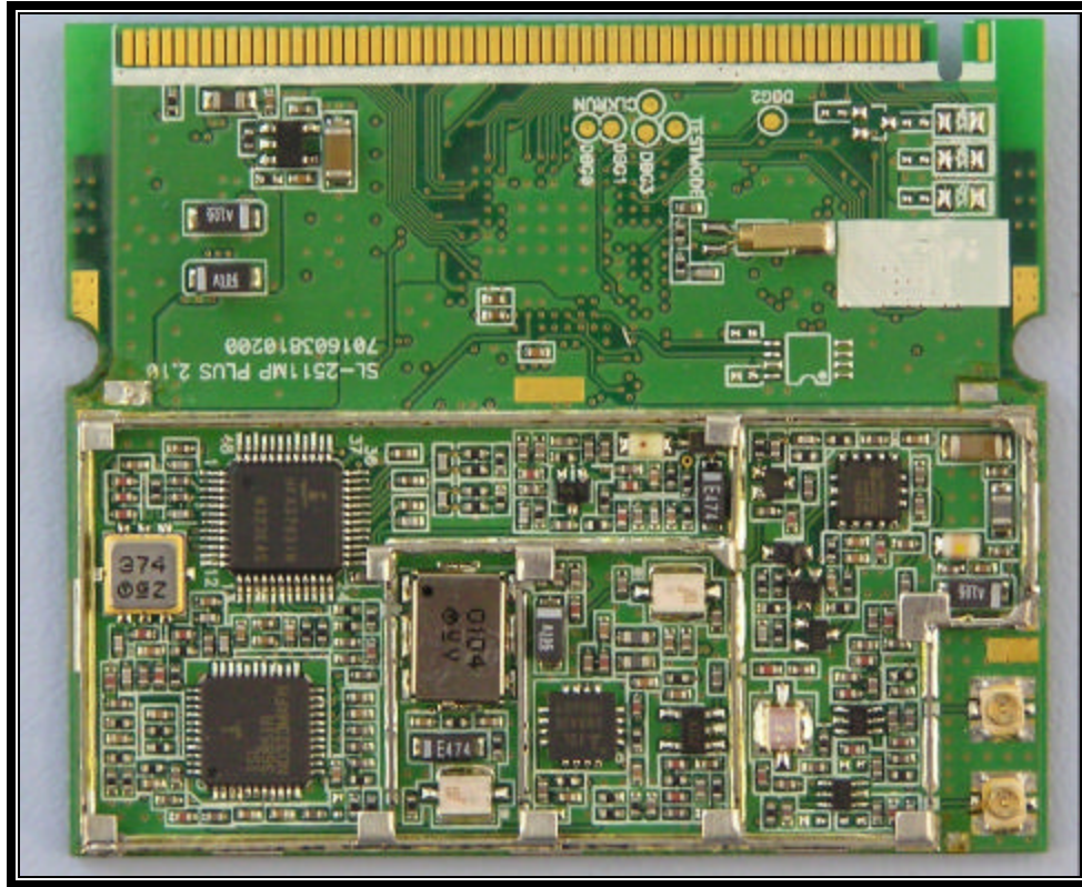
PHOTOGRAPH 14: 2511MP 11B TOP VIEW UNSHIELDED
