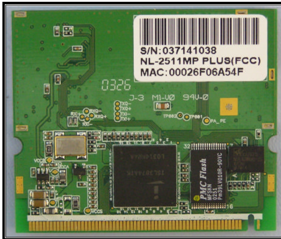
PHOTOGRAPH 15: 2511MP 11B BOTTOM VIEW
