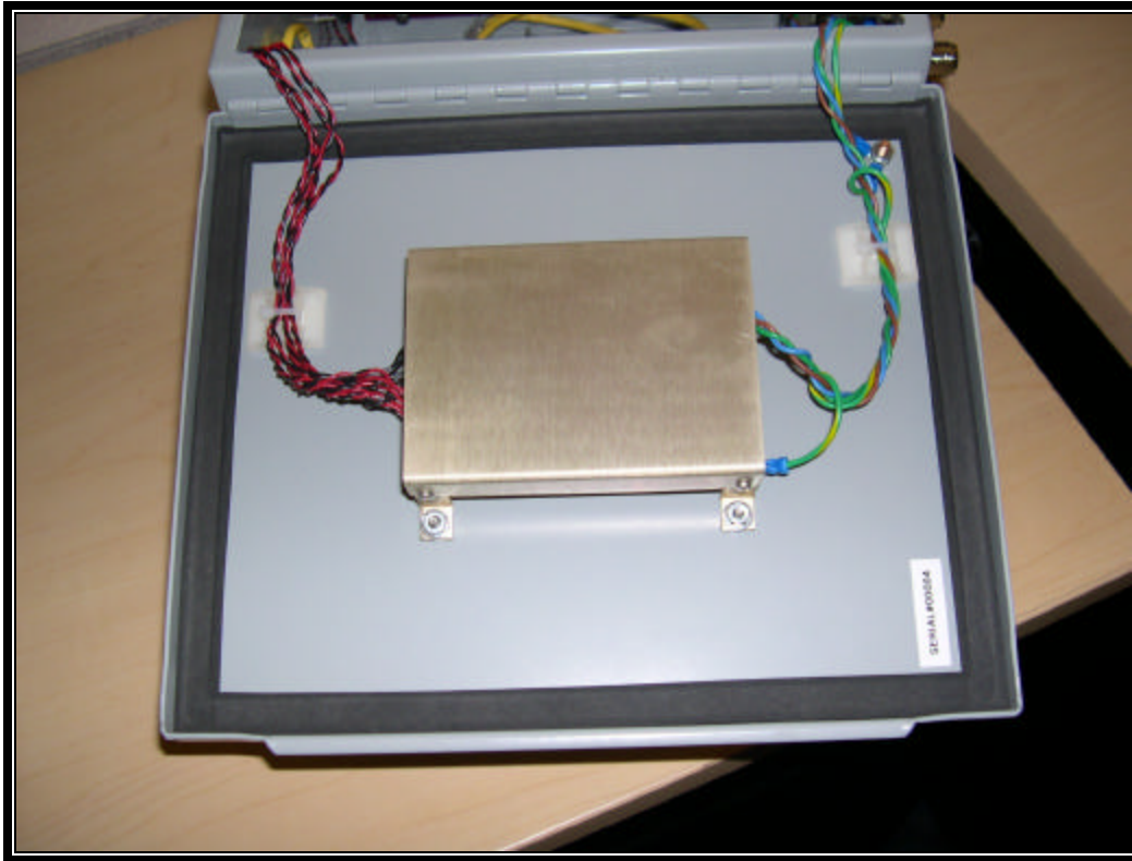
PHOTOGRAPH 7: INSIDE EUT
