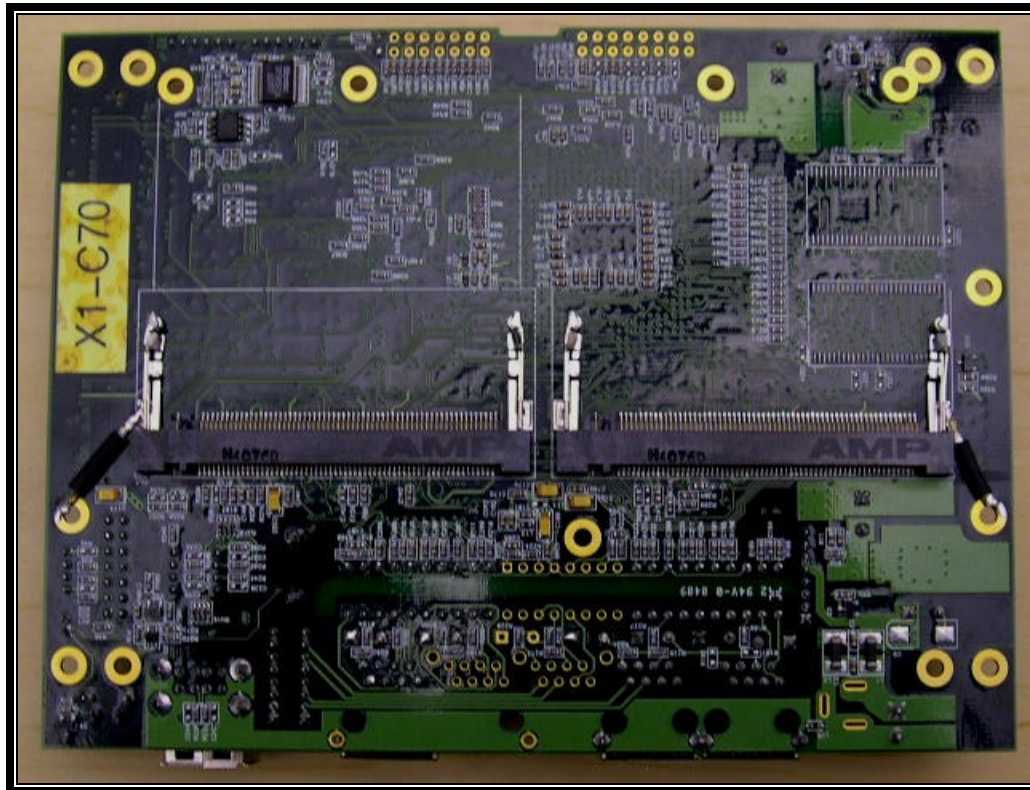
PHOTOGRAPH 12: XS 3 PT BOTTOM VIEW
