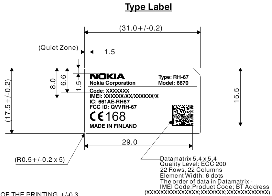
Figure 1 - Label artwork used in production
