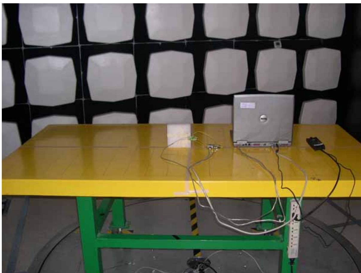
REAR VIEW
